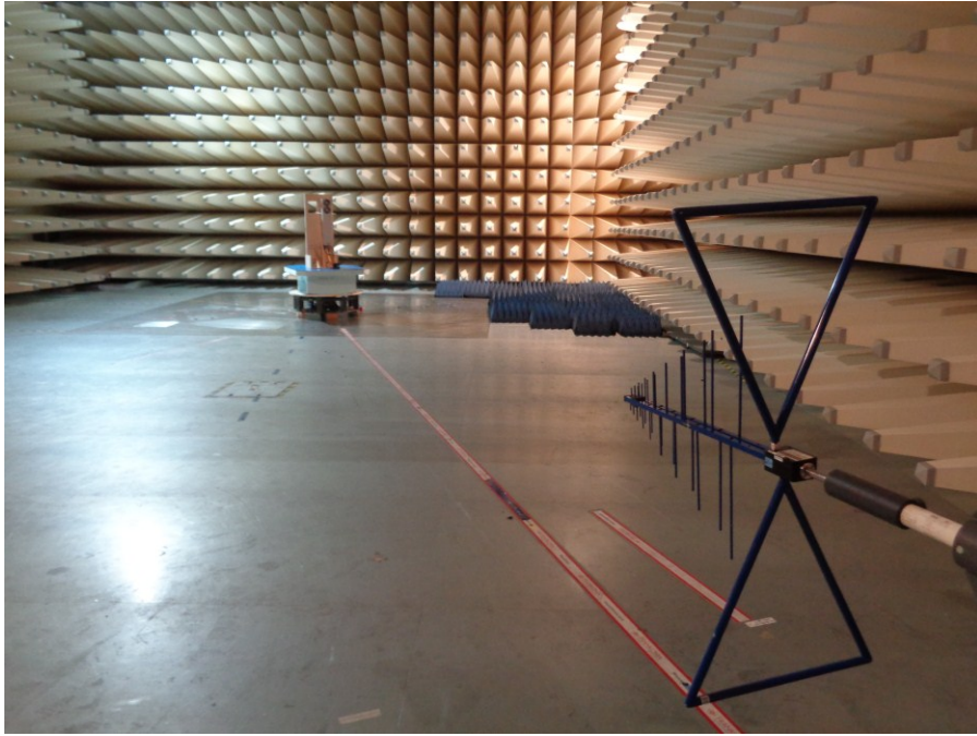
Test setup: Field Strength Emission <1 GHz @10m in the SAC
