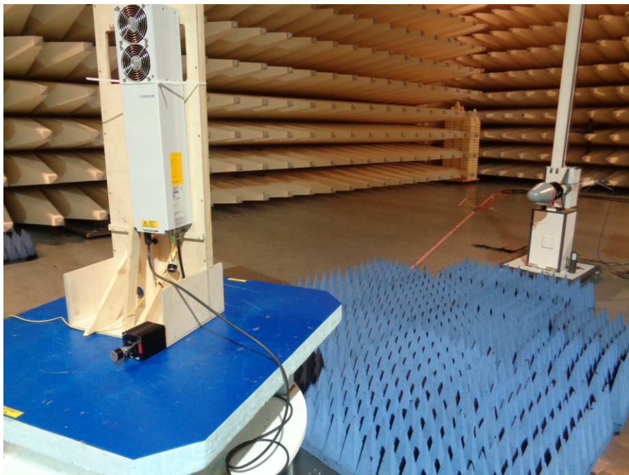
Test setup: Field Strength Emission >1 GHz @3m in the SAC
