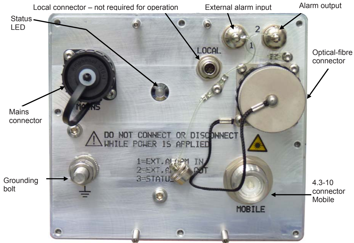
figure 4-5 Connector flange of ION-M17P/19P Advanced
