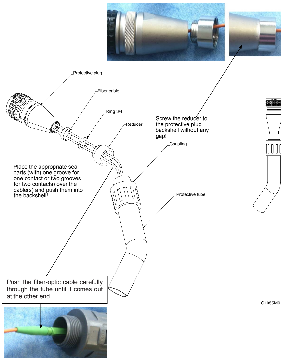
figure 4-8 Tube-kit installation
