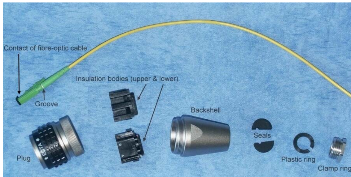
figure 4-7 Protective-plug assembly
