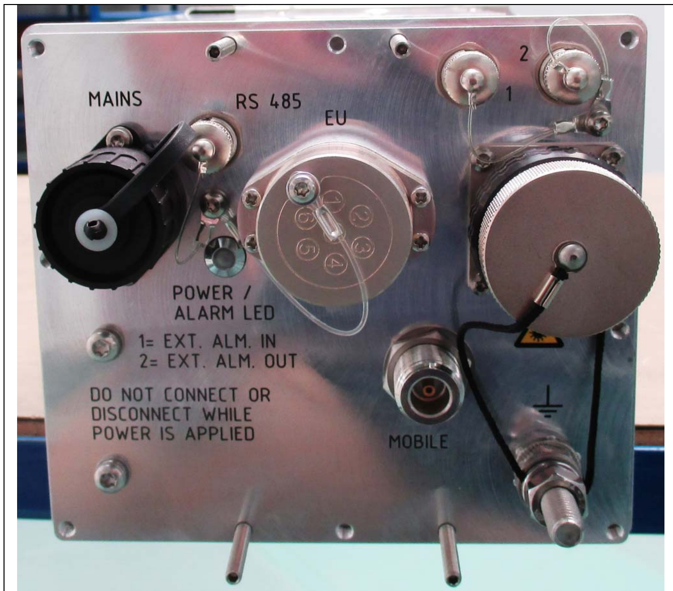
Front Flange
