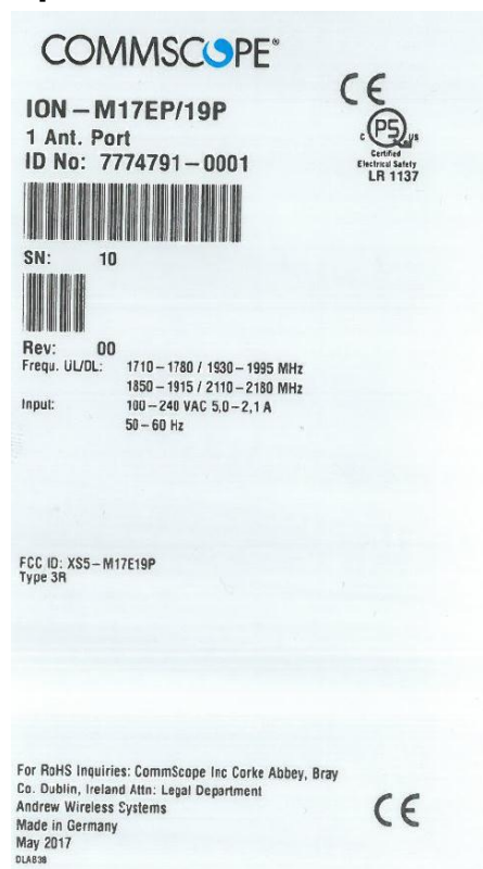
picture 8.1: label (EUT)
