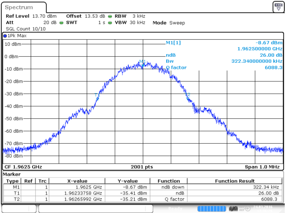
plot 6.3.2.1-#2 Occupied Bandwidth: $2.1049;; Test results; 26dB Bandwidth; GSM Input
