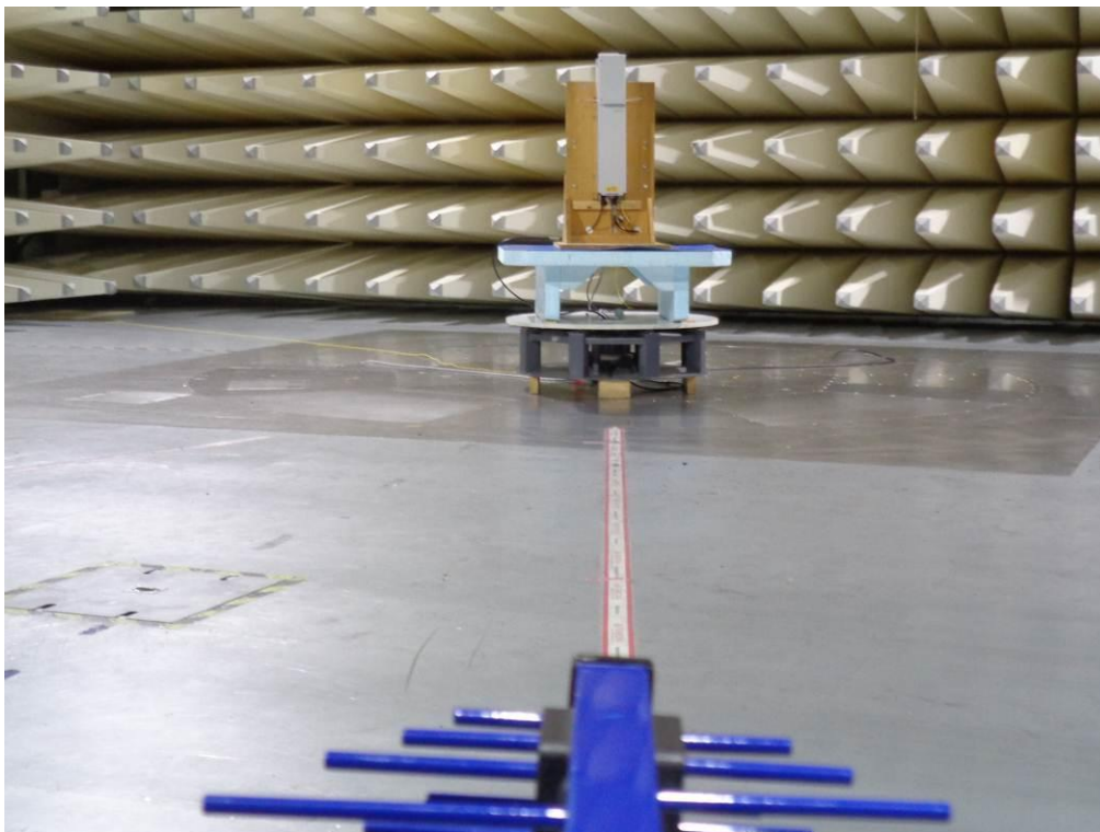
picture 8.2: Test setup: Field Strength Emission 30 M – 1 GHz @10m in the SAC
