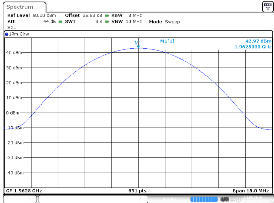
plot 5.3.1.5-#1 RF Power Out: $24.232, $2.1046; Test Results; Downlink; LTE Middle
