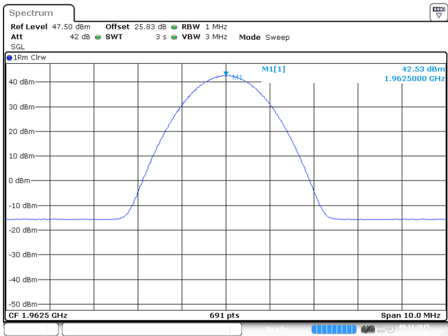
plot 5.3.1.2-#1 RF Power Out: §24.232, §2.1046; Test Results; Downlink; EDGE Middle
