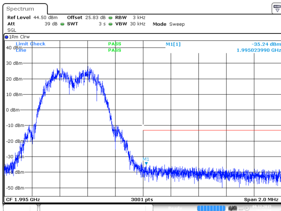
plot 8.3.1.1-#2 Intermodulation: §24.238, §2.1051; Test results; Downlink; GSM Upper Band Edge
