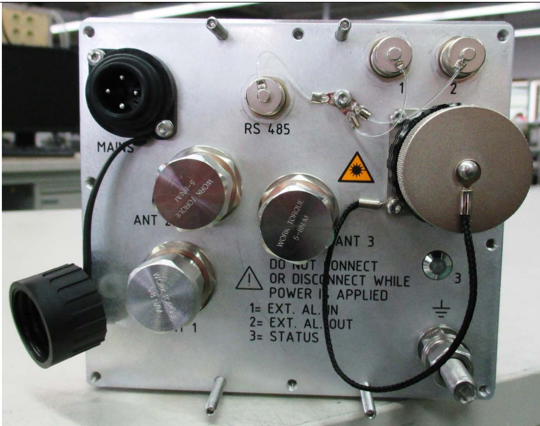
Front Flange
