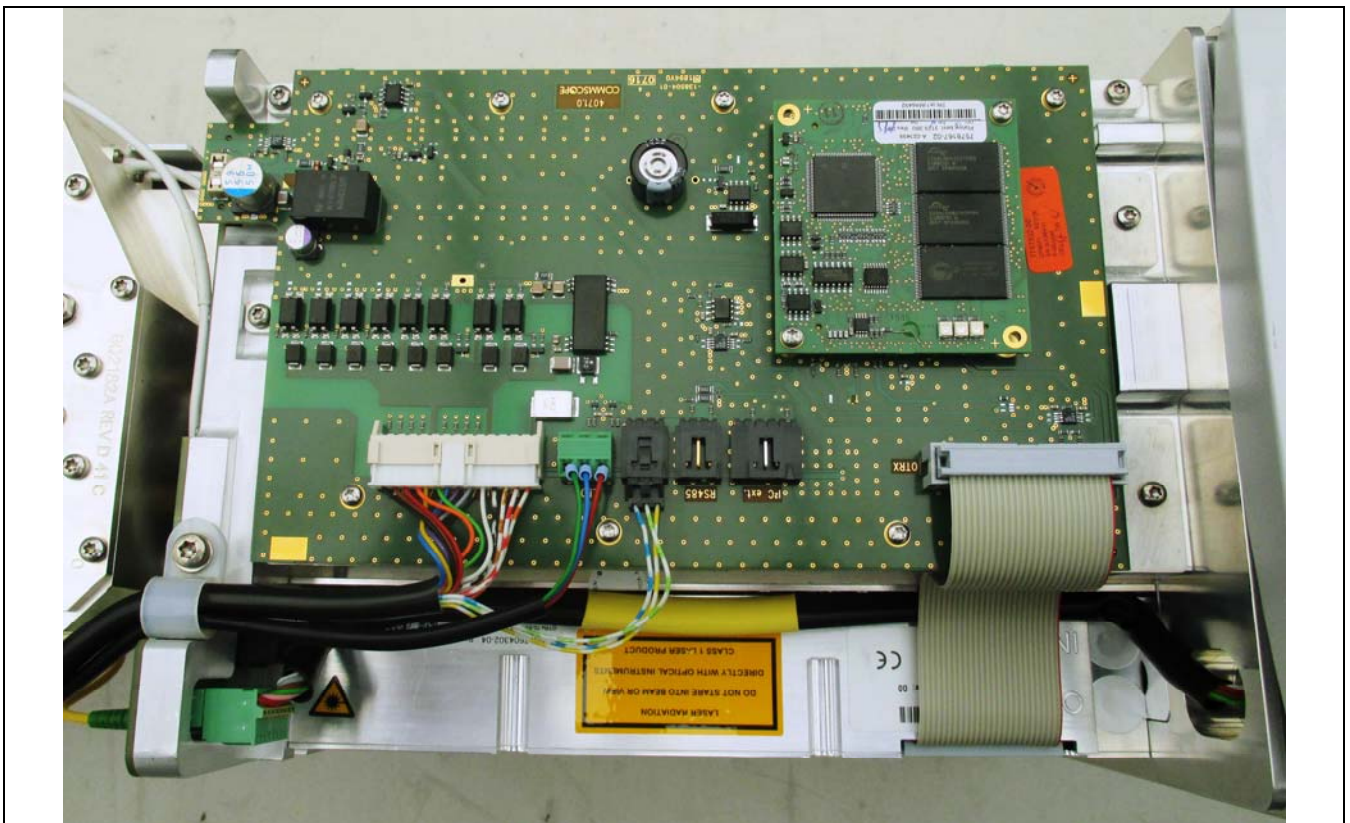
Controller PCB
