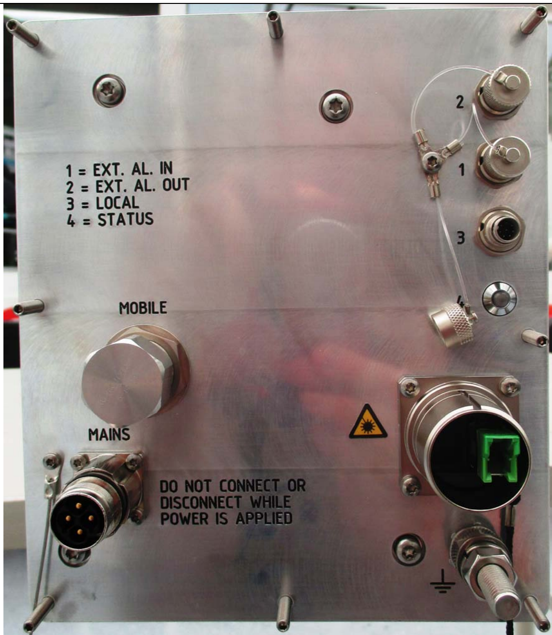
Front Flange
