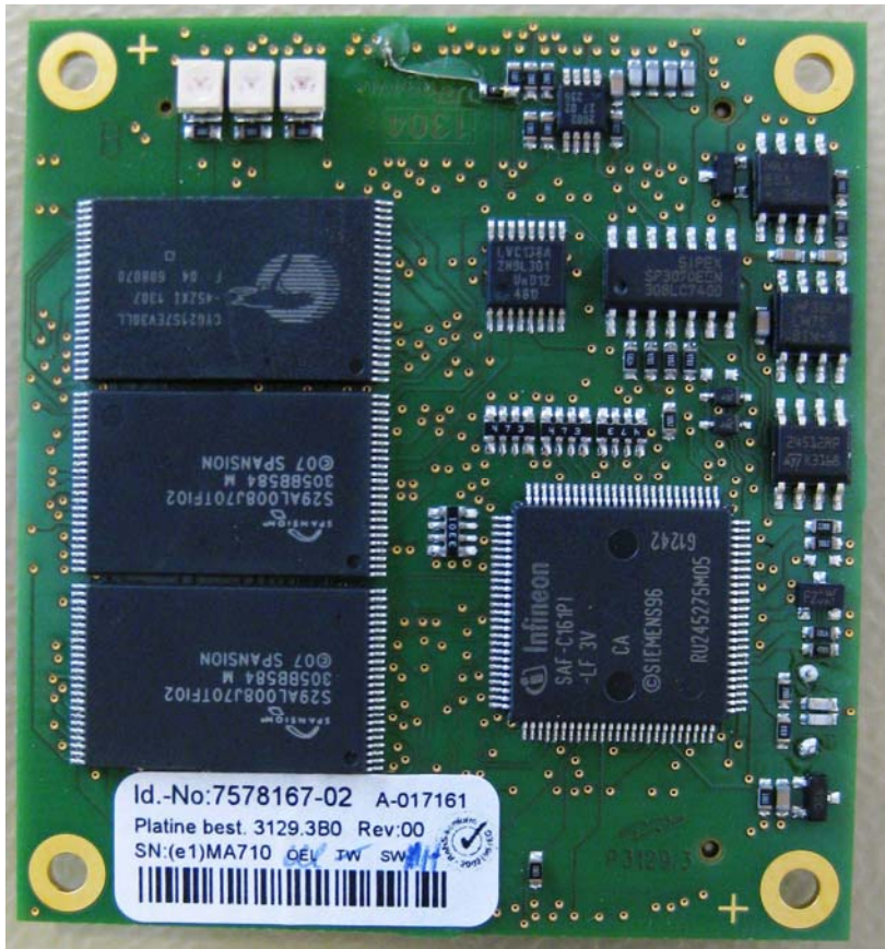
PCB P3129 Control Unit RCM161-C LT 7578167-02
