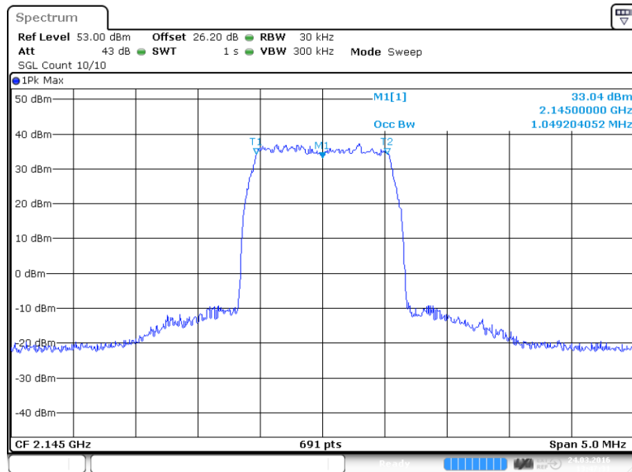
plot 6.3.1.3-#1 Occupied Bandwidth: 1.049; Test results; Downlink; LTE Output
