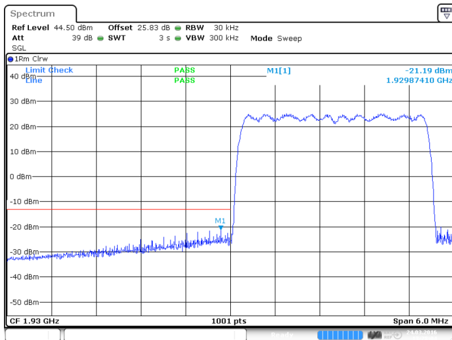
plot 8.3.1.3-#1 Intermodulation: §24.238, §2.1051; Test results; Downlink; CDMA Lower Band Edge
