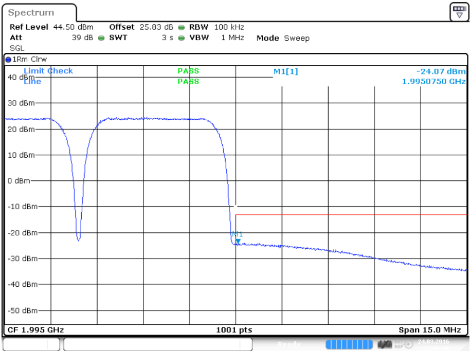
plot 8.3.1.4-#2 Intermodulation: §24.238, §2.1051; Test results; Downlink; WCDMA Upper Band Edge
