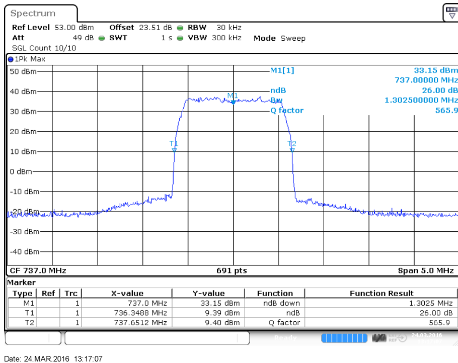
plot 6.3.2.1-#1 Occupied Bandwidth: §2.1049; Test results; 26dB Bandwidth; LTE 728 – 746MHz Output
