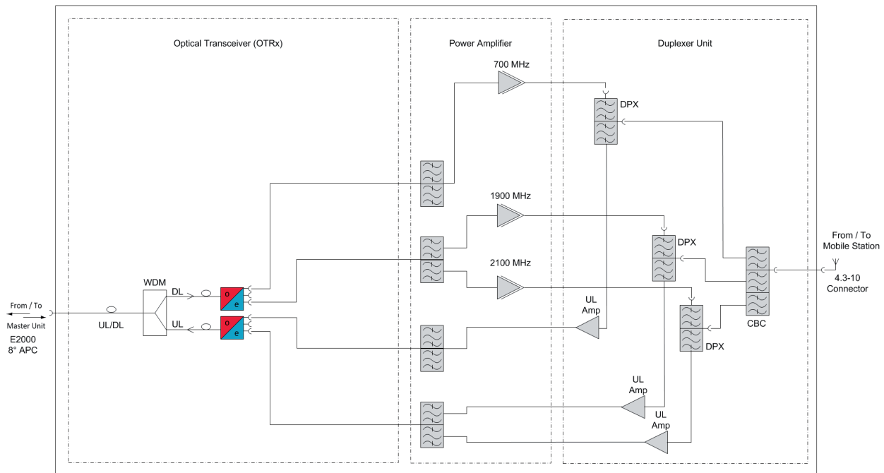
ION-M7P/17EP/19P Remote Unit Design Principle - Combined Antenna Port
