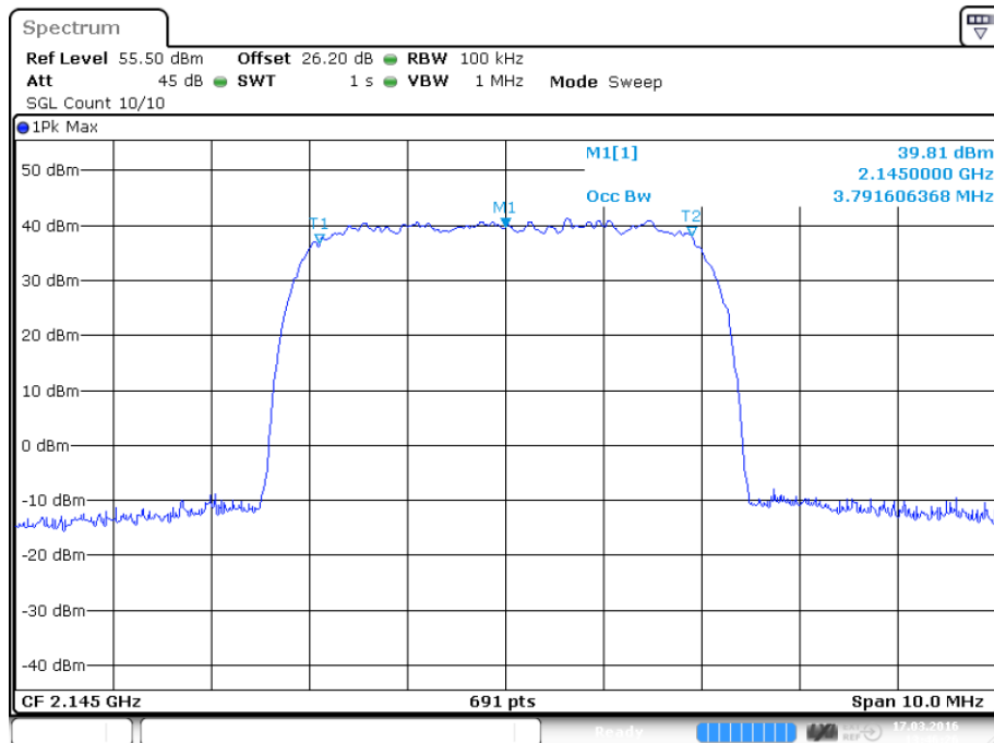
plot 6.3.1.2-#1 Occupied Bandwidth: 3.791606368 MHz; Test results; Downlink; W-CDMA Output
