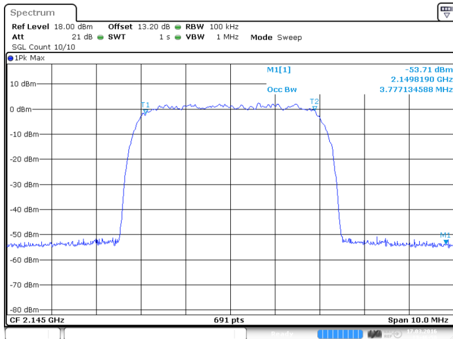
plot 6.3.1.2-#2 Occupied Bandwidth: 3.777134588 MHz; Test results; Downlink; W-CDMA Input
