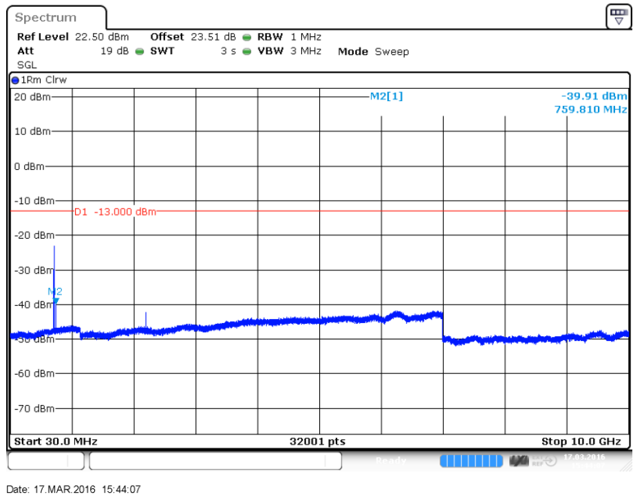
plot 7.3.1.1-#1 Spurious Emissions at Antenna Terminals: §27.53, §2.1051; Test results; Downlink; LTE 728 – 746MHz; 30 MHz – 10 GHz; carrier (737MHz) notched
