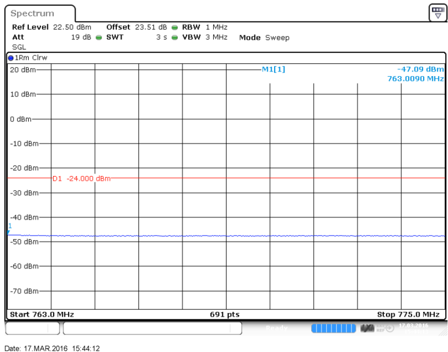
plot 7.3.1.1-#2 Spurious Emissions at Antenna Terminals: §27.53, §2.1051; Test results; Downlink; LTE 728 – 746MHz; 763 MHz – 775 MHz
