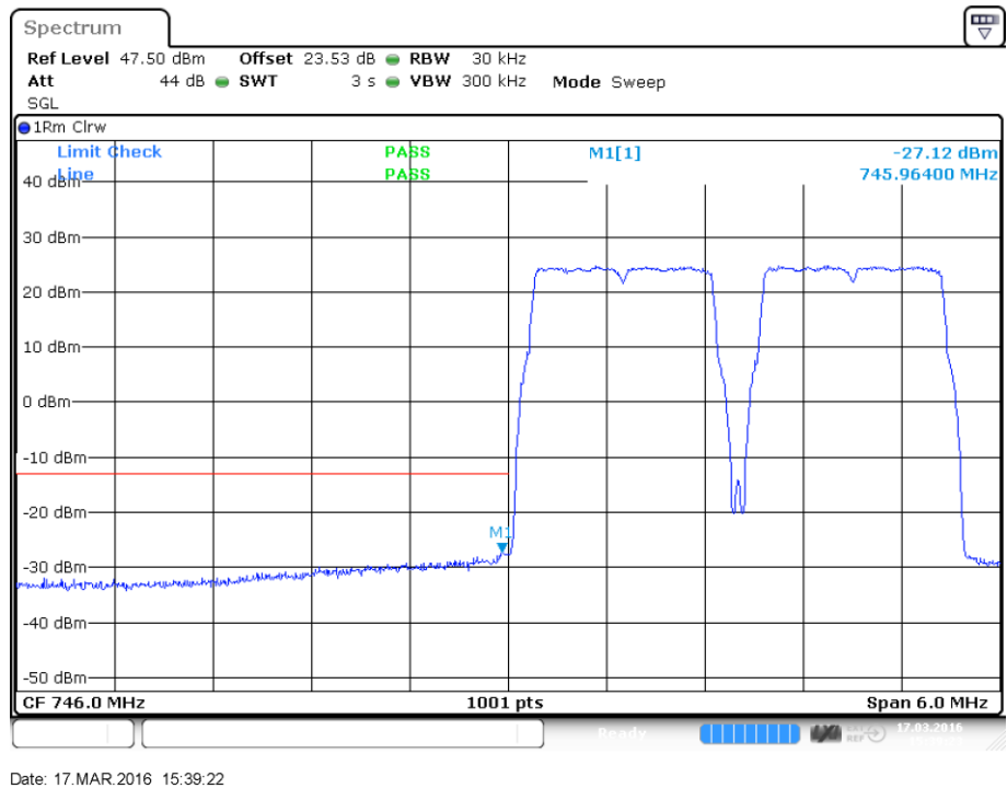
plot 8.3.1.2-#1 Intermodulation: §27.53, §2.1051; Test results; Downlink; LTE 746 – 757MHz Lower Band Edge
