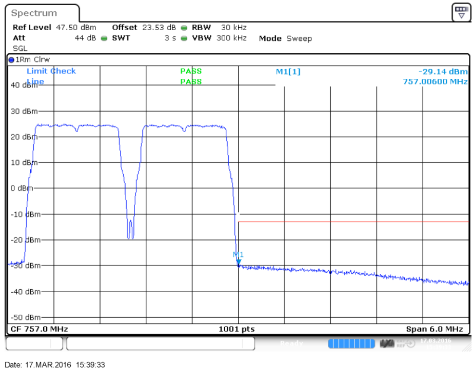
plot 8.3.1.2-#2 Intermodulation: §27.53, §2.1051; Test results; Downlink; LTE 746 – 757MHz Upper Band Edge
