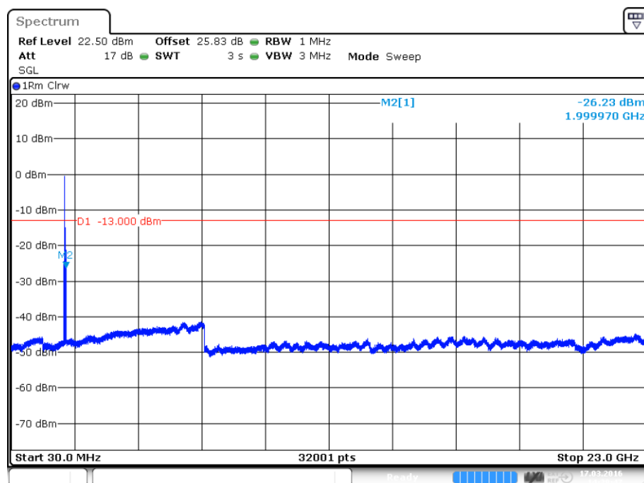
plot 7.3.1.1-#1 Spurious Emissions at Antenna Terminals: §24.238, §2.1051; Test results; Downlink; CDMA; carrier (1962.5 MHz) notched
