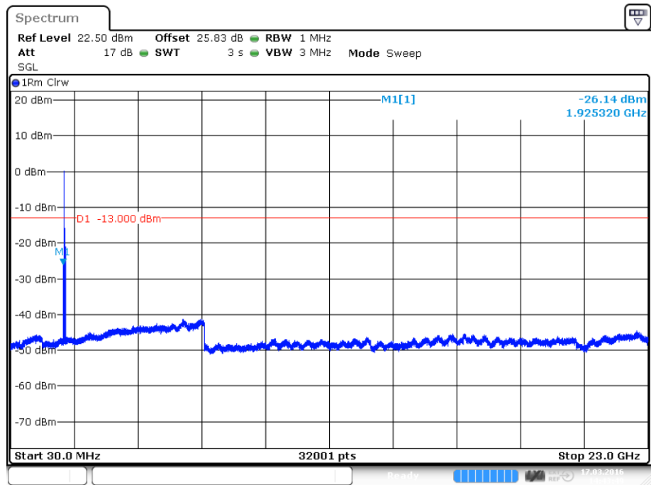
plot 7.3.1.2-#1 Spurious Emissions at Antenna Terminals: §24.238, §2.1051; Test results; Downlink; WCDMA; carrier (1962.5 MHz) notched
