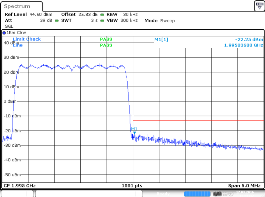
plot 8.3.1.1-#2 Intermodulation: §24.238, §2.1051; Test results; Downlink; CDMA Upper Band Edge
