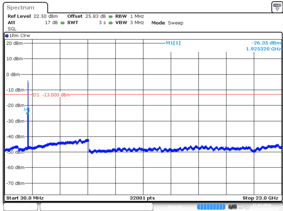
plot 7.3.1.3-#1 Spurious Emissions at Antenna Terminals: §24.238, §2.1051; Test results; Downlink; LTE; carrier (1962.5 MHz) notched
