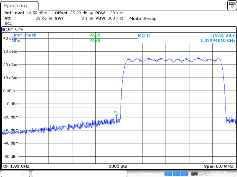
plot 8.3.1.1-#1 Intermodulation: §24.238, §2.1051; Test results; Downlink; CDMA Lower Band Edge
