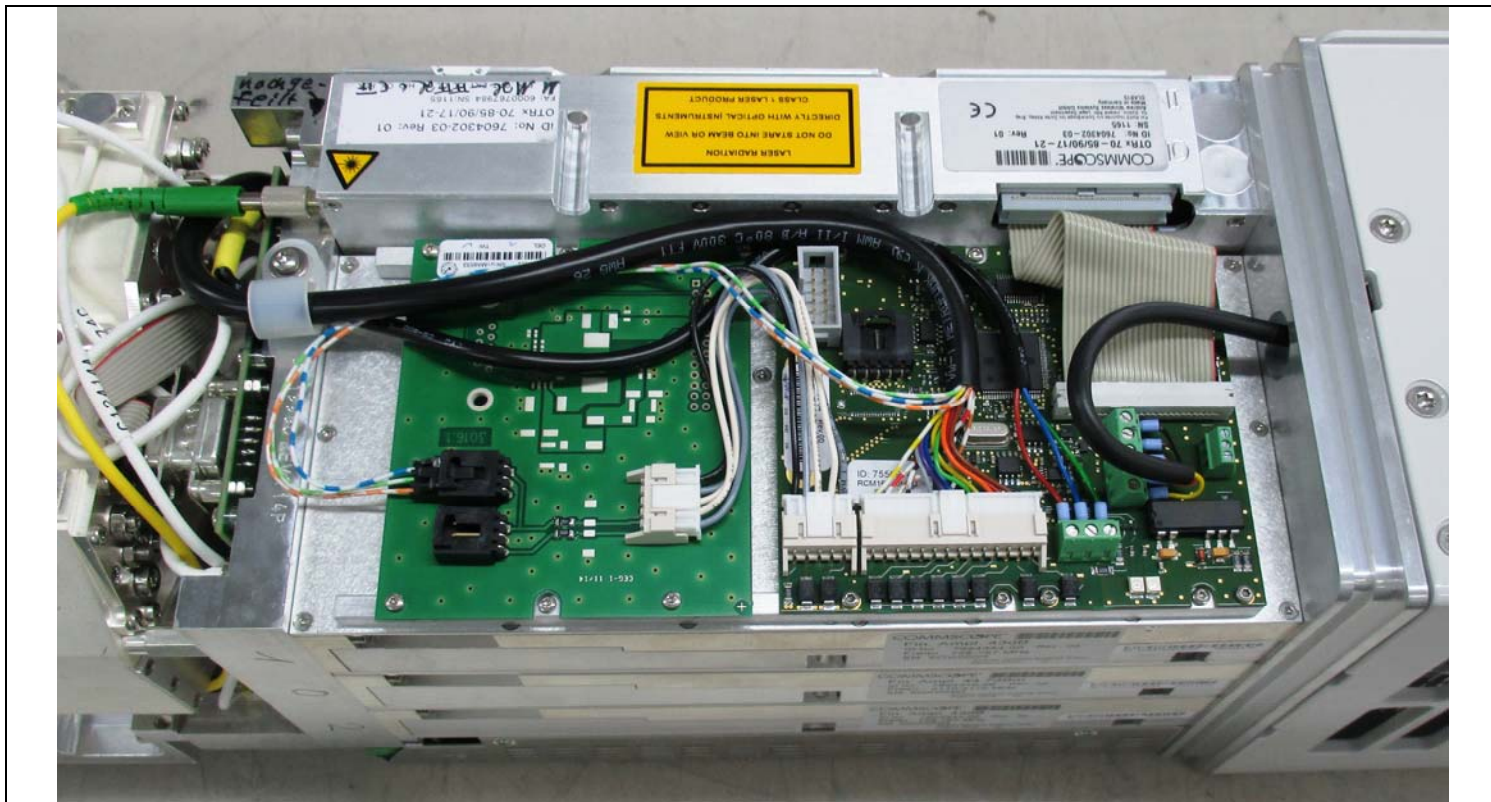
RCM161 Controller
