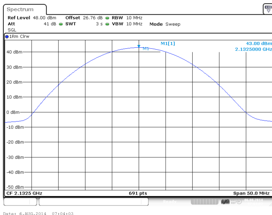
plot 5.3.1.2-#1 RF Power Out: §27.50, §2.1046; Test results; Downlink; W-CDMA Middle
