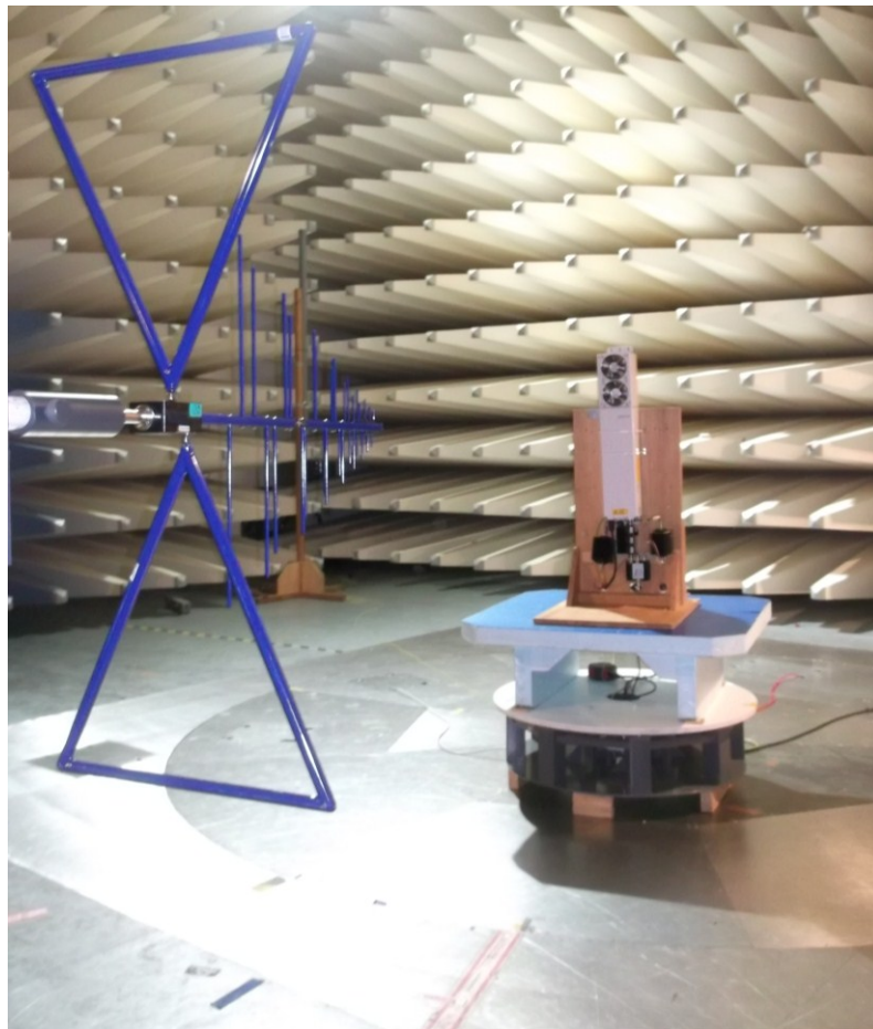
picture 8.2: Test setup: Field Strength Emission <1 GHz @3m in the SAC
