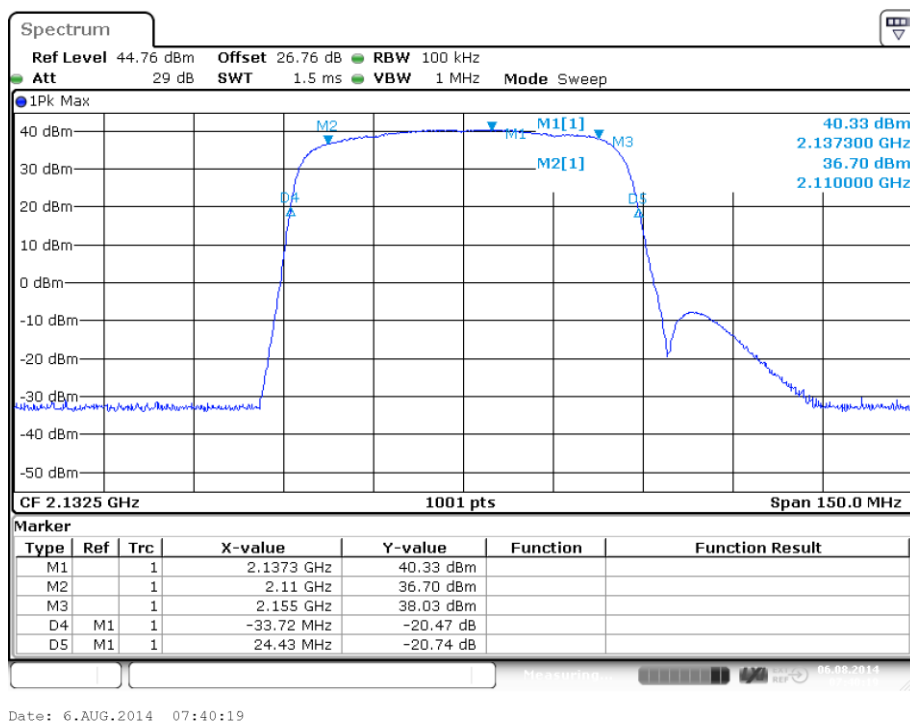
plot 8.3.1-#1 Out of Band Rejection; Test results; Downlink;
