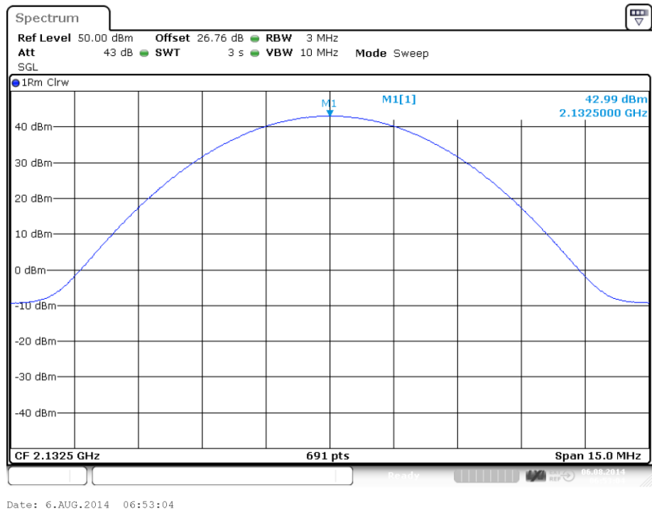
plot 5.3.1.3-#1 RF Power Out: §27.50, §2.1046; Test results; Downlink; LTE Middle
