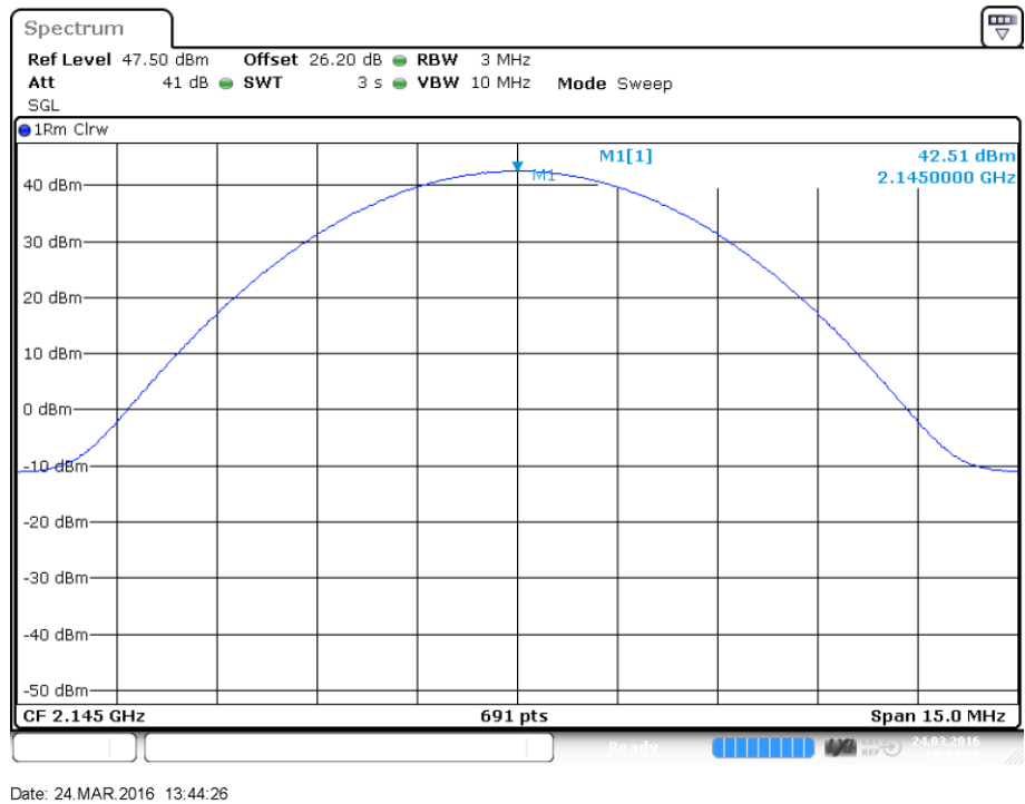
plot 5.3.1.1-#1 RF Power Out: §27.50, §2.1046; Test results; Downlink; CDMA Middle
