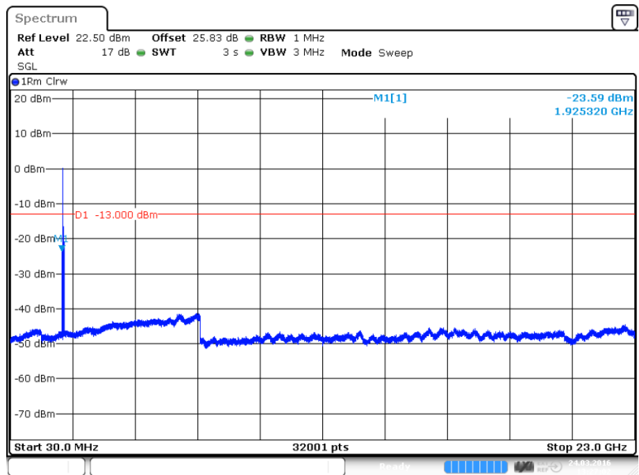
plot 7.3.1.3-#1 Spurious Emissions at Antenna Terminals: §24.238, §2.1051; Test results; Downlink; CDMA; carrier (1962.5 MHz) notched
