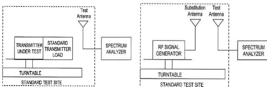
picture 8.3: Substitution method
