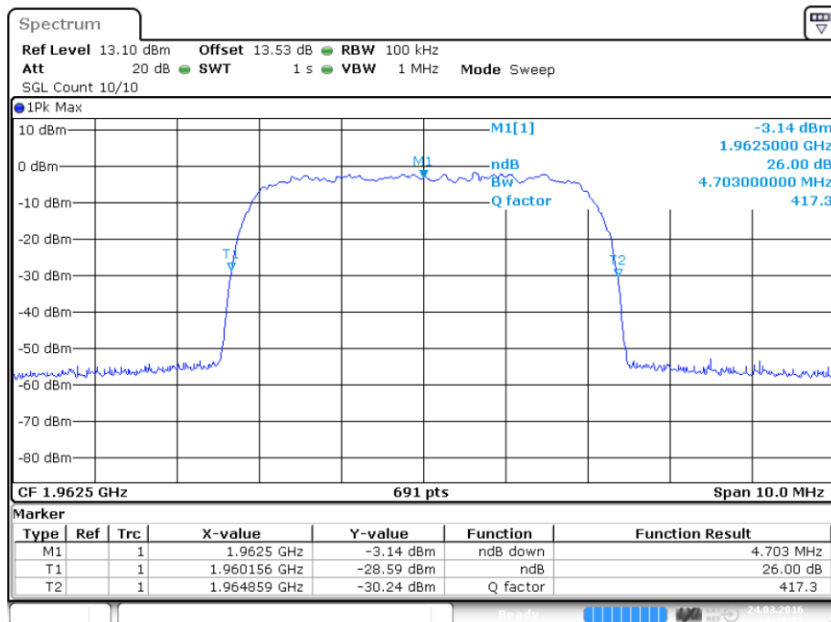
plot 6.3.2.4-#2 Occupied Bandwidth: $2.1049$; Test results; 26dB Bandwidth; WCDMA Input
