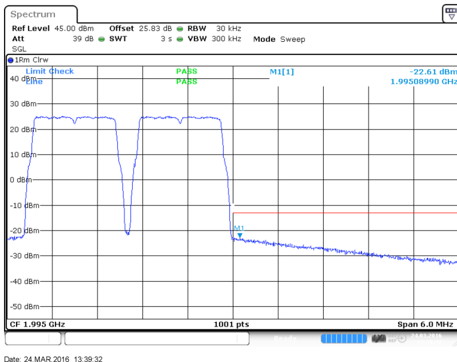
plot 8.3.1.5-#2 Intermodulation: §24.238, §2.1051; Test results; Downlink; LTE Upper Band Edge
