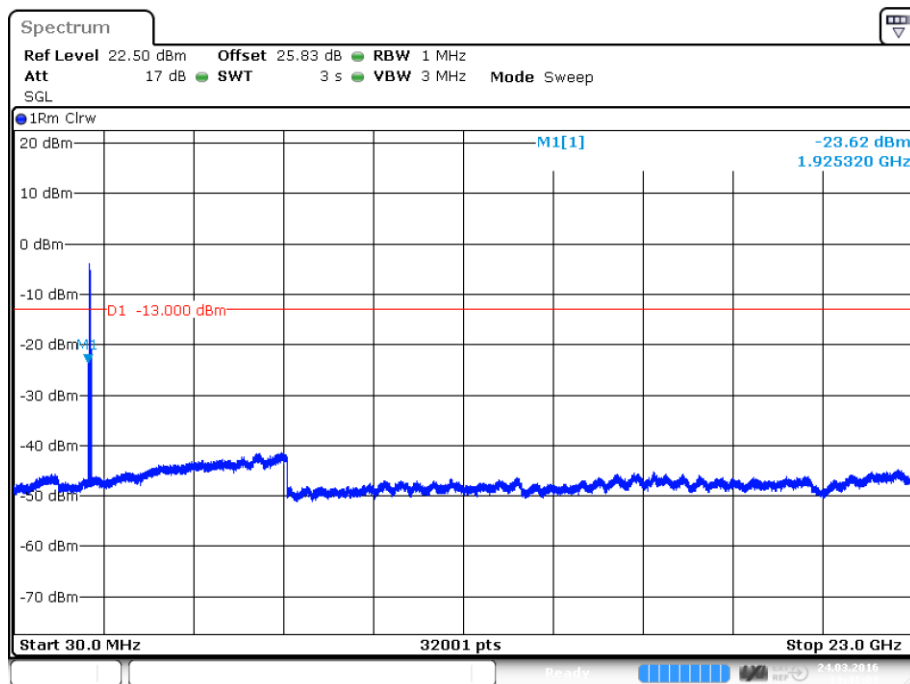
plot 7.3.1.4-#1 Spurious Emissions at Antenna Terminals: $24.238, $2.1051; Test results; Downlink; WCDMA; carrier (1962.5 MHz) notched
