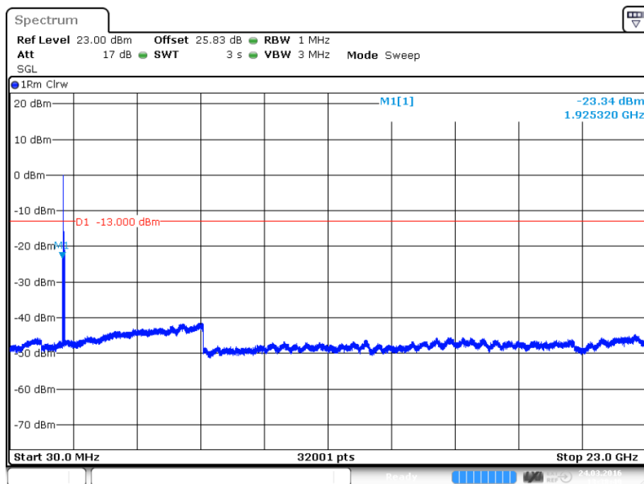
plot 7.3.1.5-#1 Spurious Emissions at Antenna Terminals: $24.238, $2.1051; Test results; Downlink; LTE; carrier (1962.5 MHz) notched
