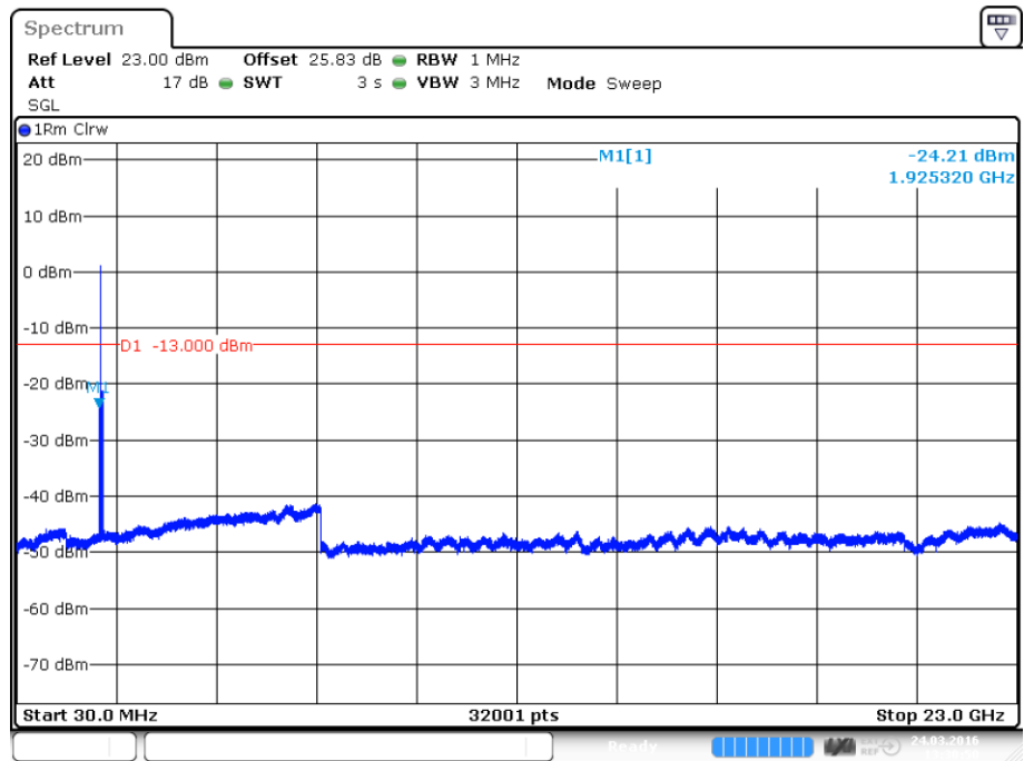
plot 7.3.1.2-#1 Spurious Emissions at Antenna Terminals: §24.238, §2.1051; Test results; Downlink; EDGE; carrier (1962.5 MHz) notched
