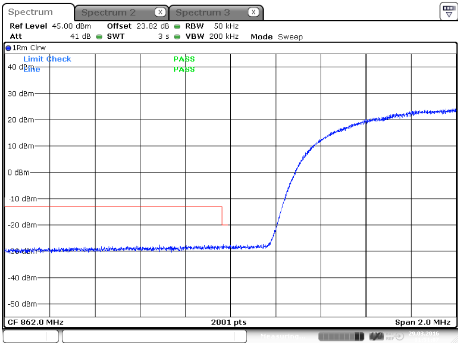
plot 9.3.1.4-#1 Emission Mask: §90.691, §2.1051; Test results; Downlink; WCDMA Lower Band Edge
