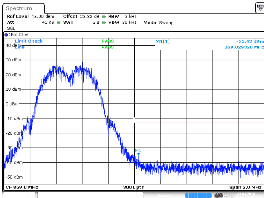
plot 8.3.1.1-#2 Intermodulation: §90.219, §2.1051; Test results; Downlink; GSM Upper Band Edge
