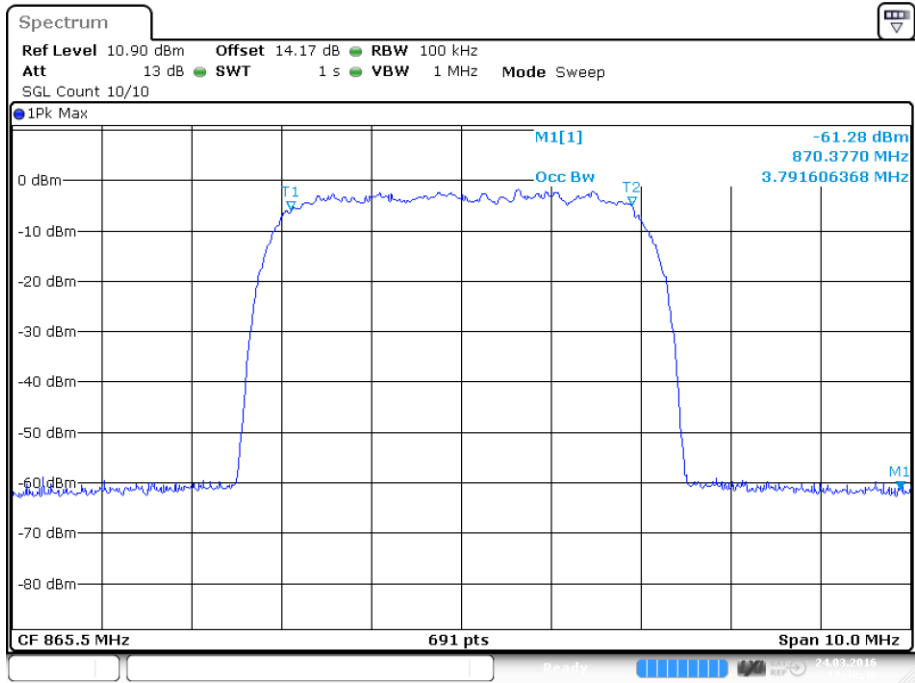
plot 6.3.1.4-#2 Occupied Bandwidth: $90.210, $2.1049; Test results; Downlink; WCDMA Input
