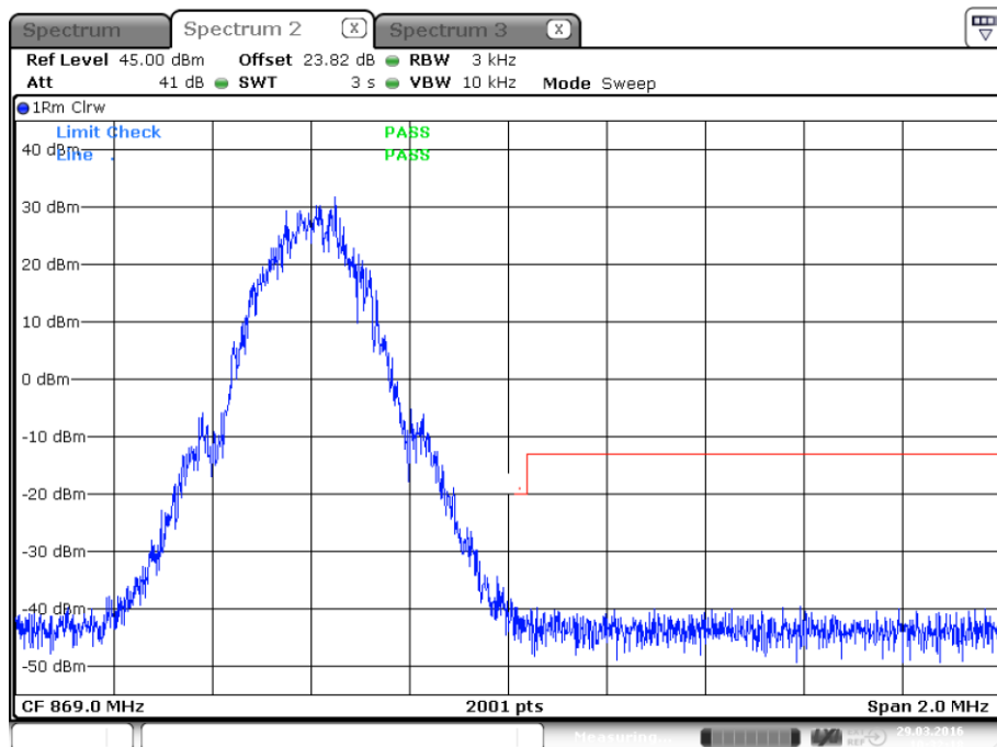
plot 9.3.1.1-#1 Emission Mask: §90.691, §2.1051; Test results; Downlink; GSM Lower Band Edge
