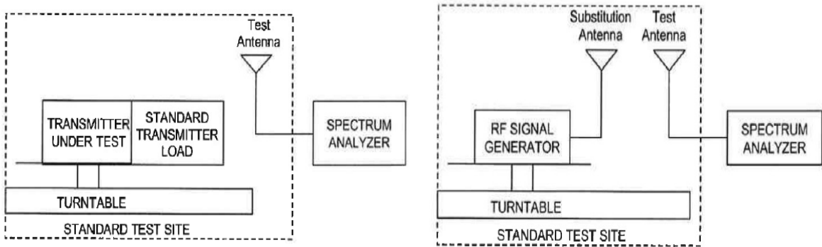
picture 8.3: Substitution method
