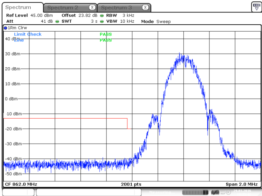
plot 9.3.1.2-#1 Emission Mask: §90.691, §2.1051; Test results; Downlink; EDGE Lower Band Edge
