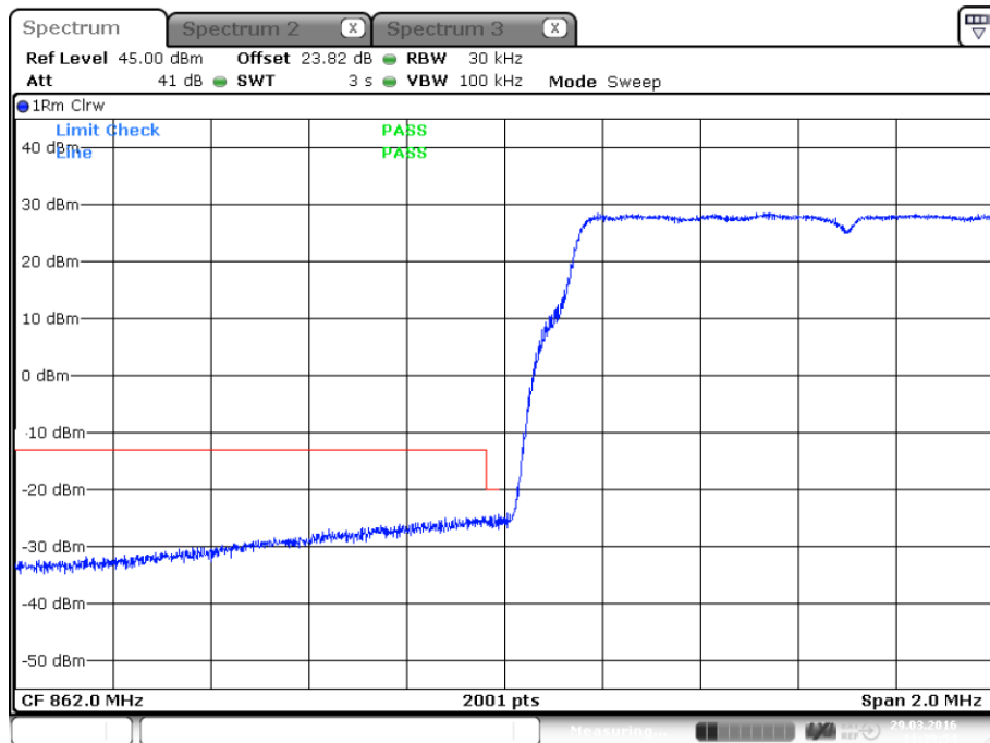
plot 9.3.1.5-#1 Emission Mask: §90.691, §2.1051; Test results; Downlink; LTE Lower Band Edge
