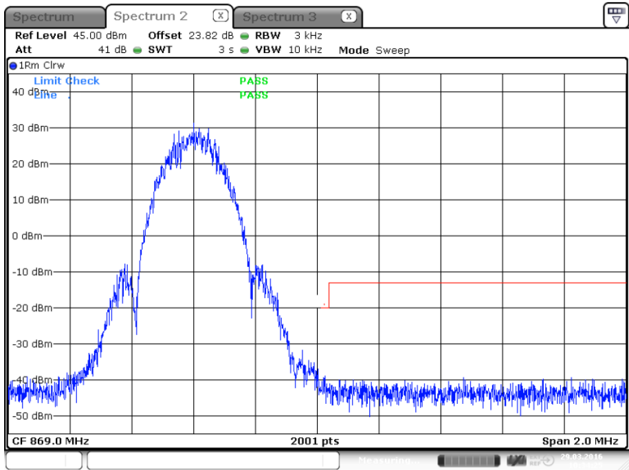
plot 9.3.1.2-#2 Emission Mask: §90.691, §2.1051; Test results; Downlink; EDGE Upper Band Edge
