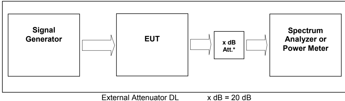
figure 5-#1 Test setup: RF Power Out: §90.635, §2.1046
