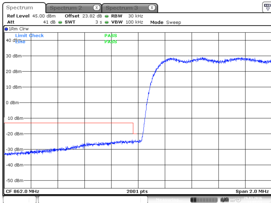
plot 9.3.1.3-#1 Emission Mask: §90.691, §2.1051; Test results; Downlink; CDMA Lower Band Edge
