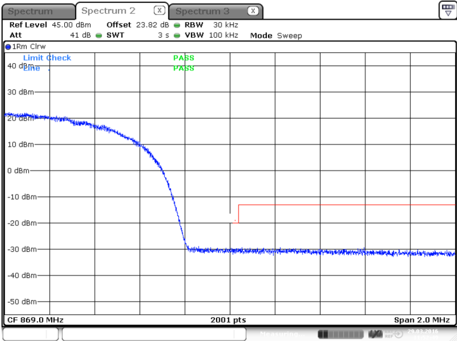
plot 9.3.1.4-#2 Emission Mask: §90.691, §2.1051; Test results; Downlink; WCDMA Upper Band Edge
