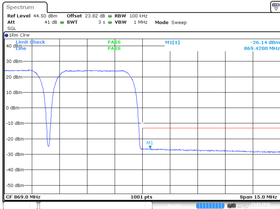
plot 8.3.1.4-#2 Intermodulation: §90.219, §2.1051; Test results; Downlink; WCDMA Upper Band Edge
