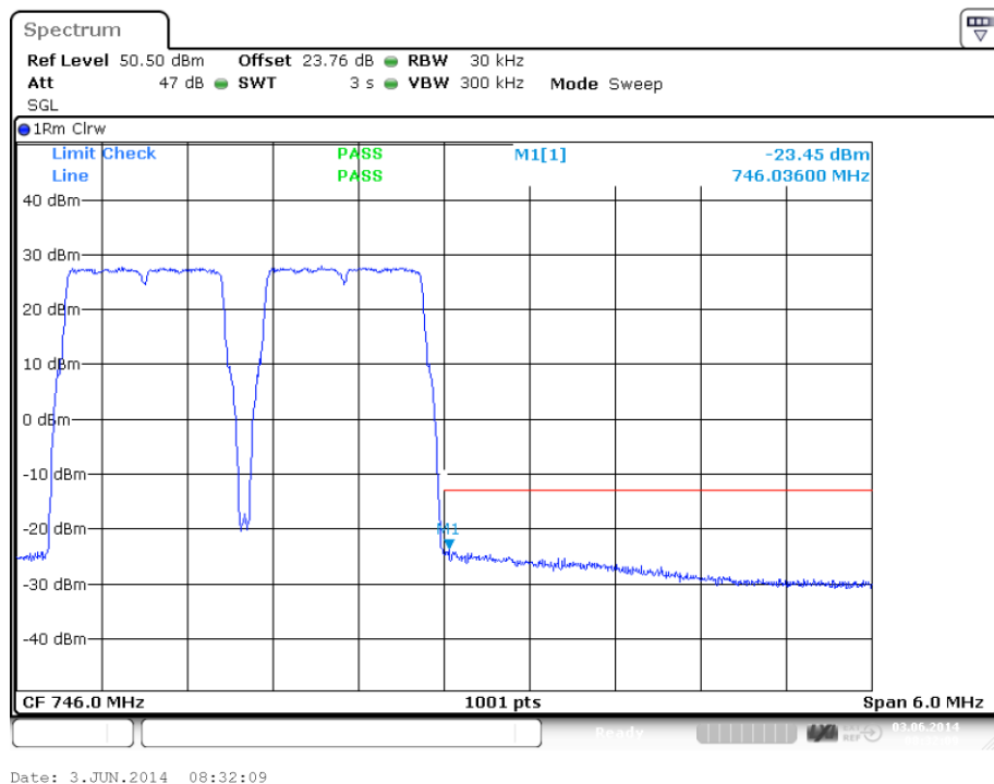
plot 7.3.1.1-#2 Spurious Emissions at Antenna Terminals: §27.53, §2.1051; Test results; Downlink; LTE < 1MHz to band edge; 728 – 746MHz Upper Band Edge
