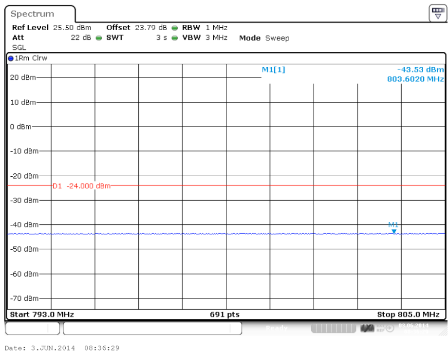
plot 7.3.1.4-#3 Spurious Emissions at Antenna Terminals: §27.53, §2.1051; Test results; Downlink; LTE > 1MHz to band edge 746 – 757MHz; 793 MHz – 805 MHz
