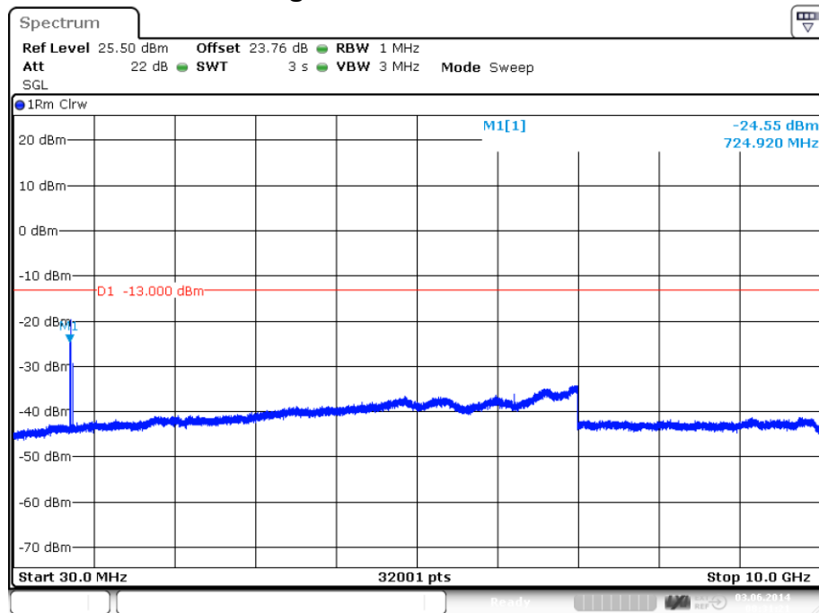
plot 7.3.1.3-#1 Spurious Emissions at Antenna Terminals: §27.53, §2.1051; Test results; Downlink; LTE &gt; 1MHz to band edge 728 – 746MHz; 30 MHz – 10 GHz; carrier (737MHz) notched
