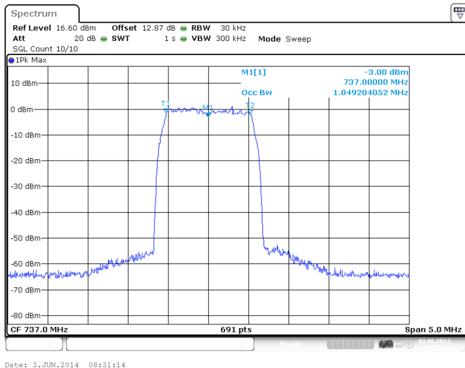
plot 6.3.1.1-#2 Occupied Bandwidth: $90.210, $2.1049; Test results; Downlink; LTE 728 – 746MHz Input
