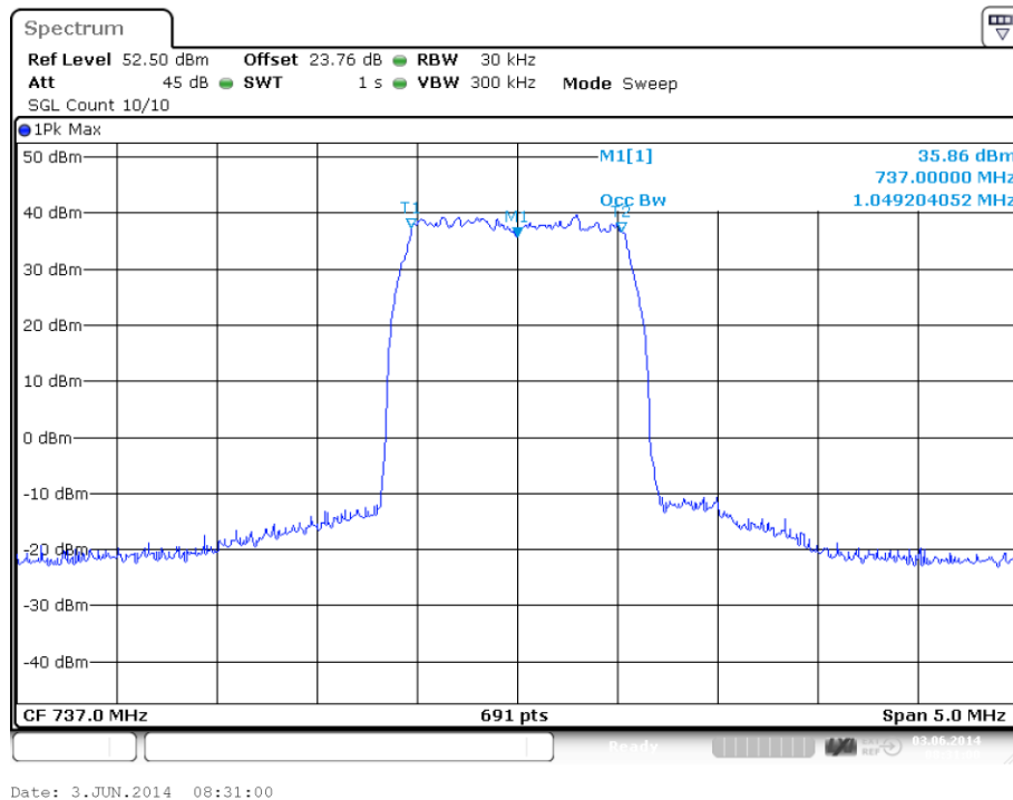
plot 6.3.1.1-#1 Occupied Bandwidth: $90.210, $2.1049; Test results; Downlink; LTE 728 – 746MHz Output
