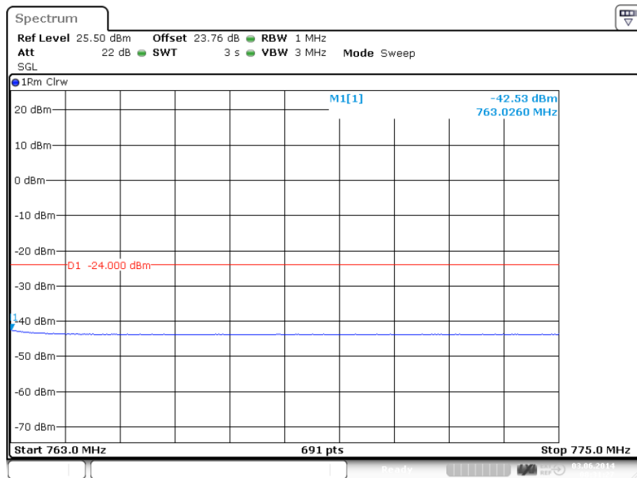
plot 7.3.1.3-#2 Spurious Emissions at Antenna Terminals: §27.53, §2.1051; Test results; Downlink; LTE &gt; 1MHz to band edge 728 – 746MHz; 763 MHz – 775 MHz
