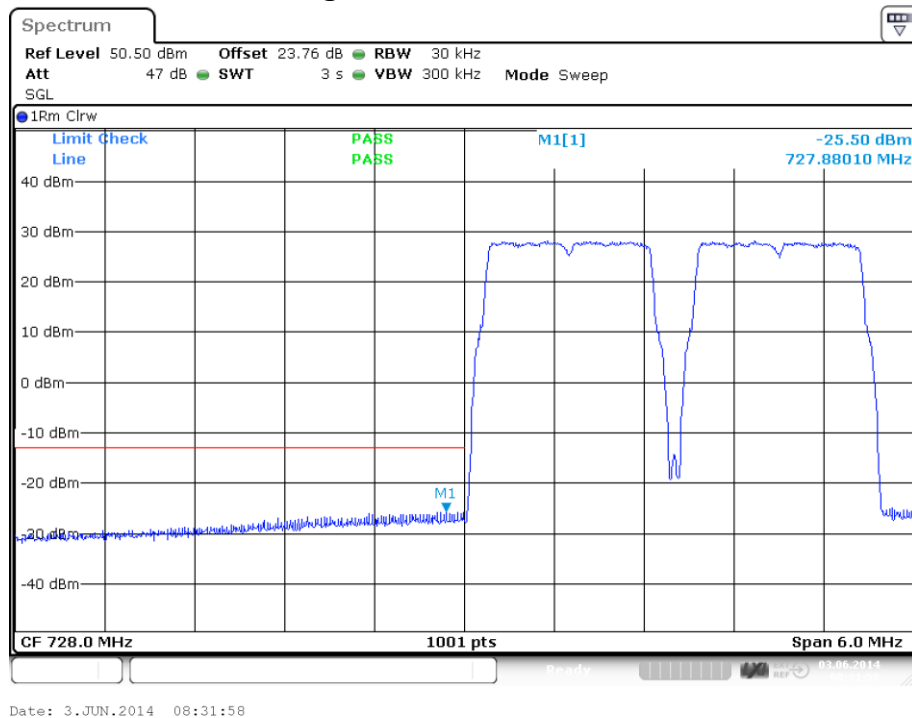
plot 7.3.1.1-#1 Spurious Emissions at Antenna Terminals: §27.53, §2.1051; Test results; Downlink; LTE < 1MHz to band edge; 728 – 746MHz Lower Band Edge
