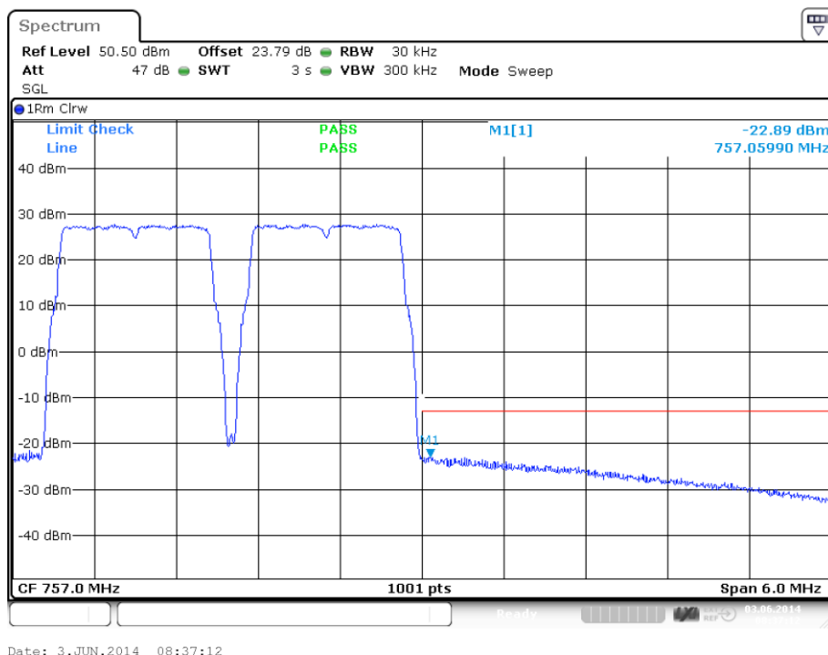
plot 7.3.1.2-#2 Spurious Emissions at Antenna Terminals: §27.53, §2.1051; Test results; Downlink; LTE &lt; 1MHz to band edge 746 – 757MHz Upper Band Edge
