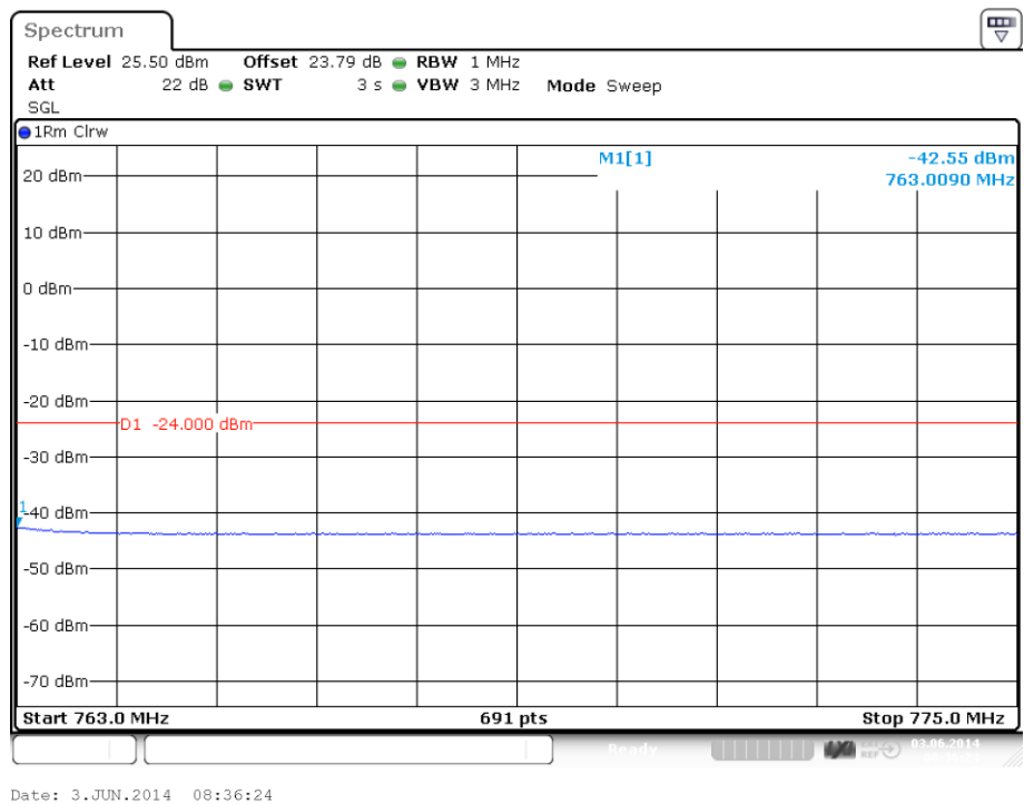
plot 7.3.1.4-#2 Spurious Emissions at Antenna Terminals: §27.53, §2.1051; Test results; Downlink; LTE > 1MHz to band edge 746 – 757MHz; 763 MHz – 775 MHz
