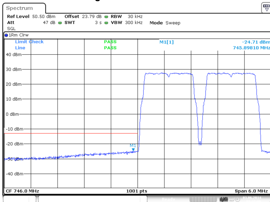
plot 7.3.1.2-#1 Spurious Emissions at Antenna Terminals: §27.53, §2.1051; Test results; Downlink; LTE &lt; 1MHz to band edge 746 – 757MHz Lower Band Edge
