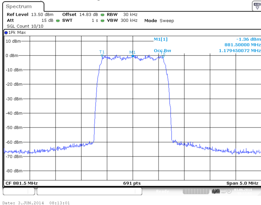
plot 6.3.1.4-#2 Occupied Bandwidth: $2.1049; RSS-GEN; Test results; Downlink; CDMA Input
