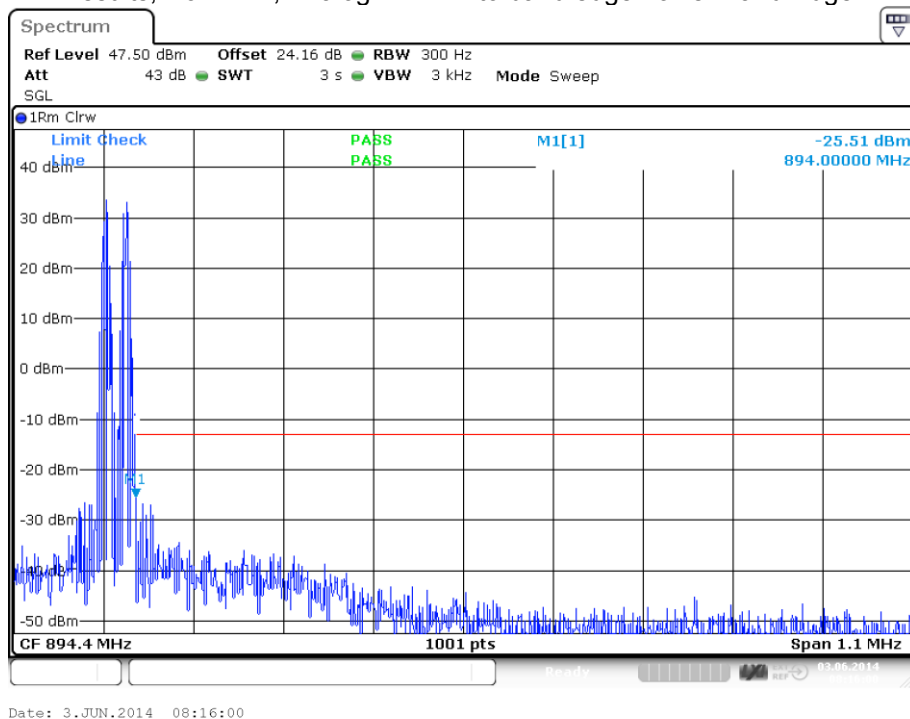
plot 7.3.1.1-#2 Spurious Emissions at Antenna Terminals: §22.917, §2.1051; RSS-131, RSS-GEN; Test results; Downlink; Analog < 1MHz to band edge Upper Band Edge
