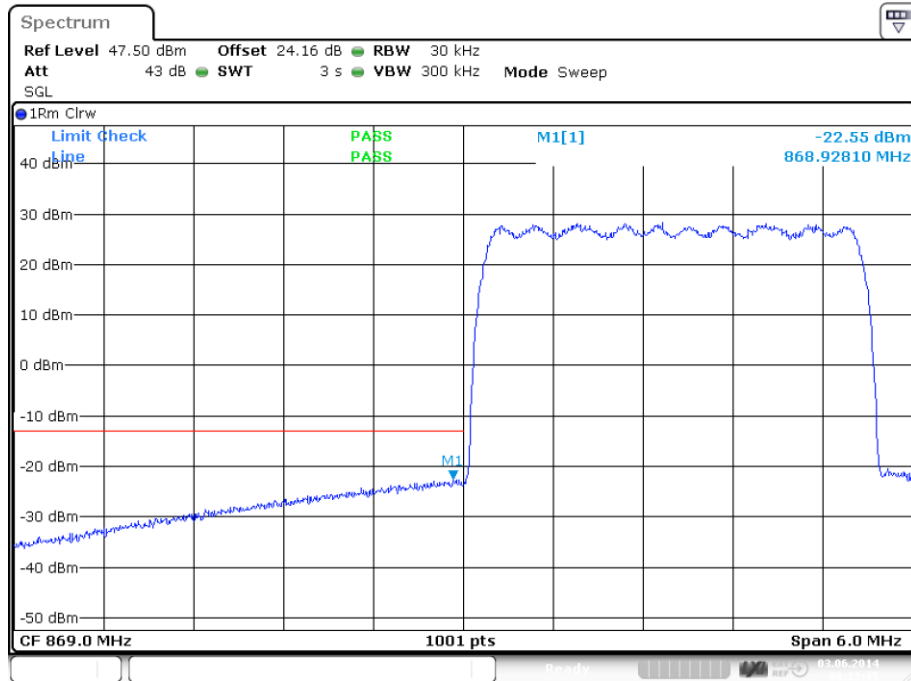
plot 7.3.1.4-#1 Spurious Emissions at Antenna Terminals: §22.917, §2.1051; RSS-131, RSS-GEN; Test results; Downlink; CDMA &lt; 1MHz to band edge Lower Band Edge
