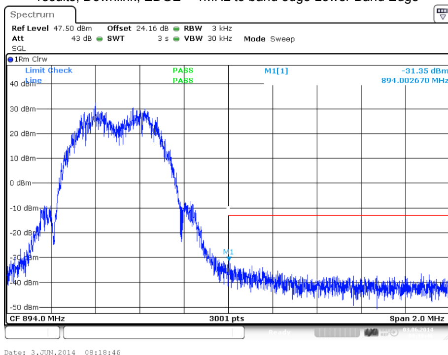
plot 7.3.1.3-#2 Spurious Emissions at Antenna Terminals: §22.917, §2.1051; RSS-131, RSS-GEN; Test results; Downlink; EDGE < 1MHz to band edge Upper Band Edge
