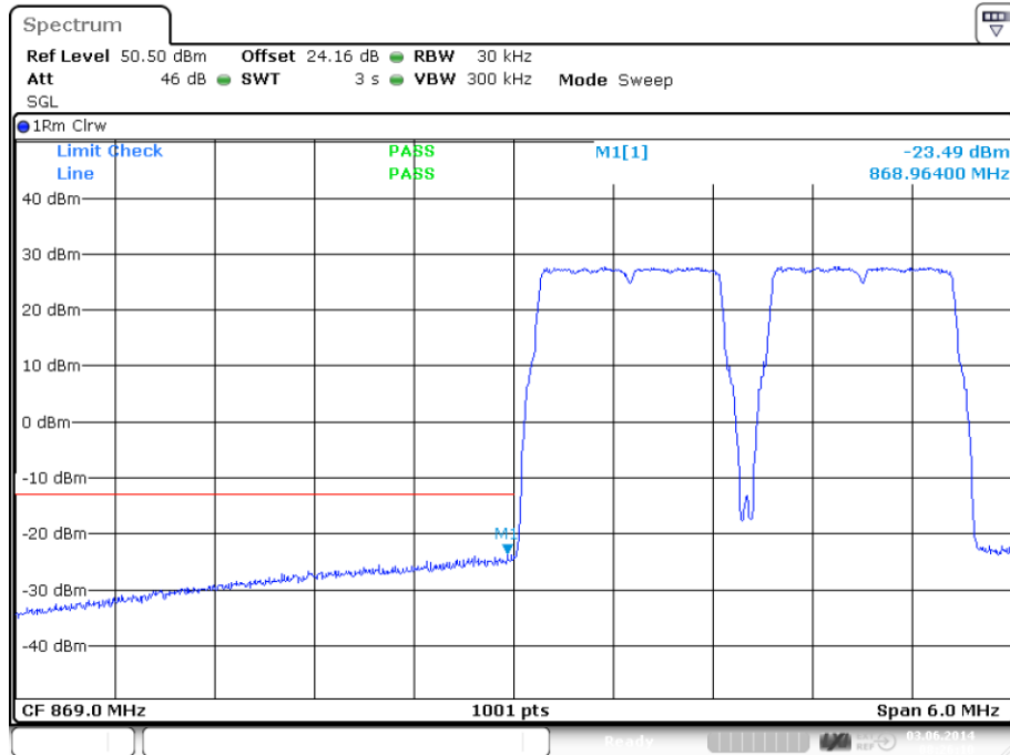
plot 7.3.1.6-#1 Spurious Emissions at Antenna Terminals: §22.917, §2.1051; RSS-131, RSS-GEN; Test results; Downlink; LTE &lt; 1MHz to band edge Lower Band Edge
