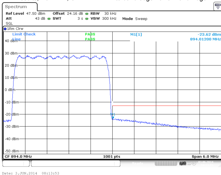
plot 7.3.1.4-#2 Spurious Emissions at Antenna Terminals: §22.917, §2.1051; RSS-131, RSS-GEN; Test results; Downlink; CDMA &lt; 1MHz to band edge Upper Band Edge
