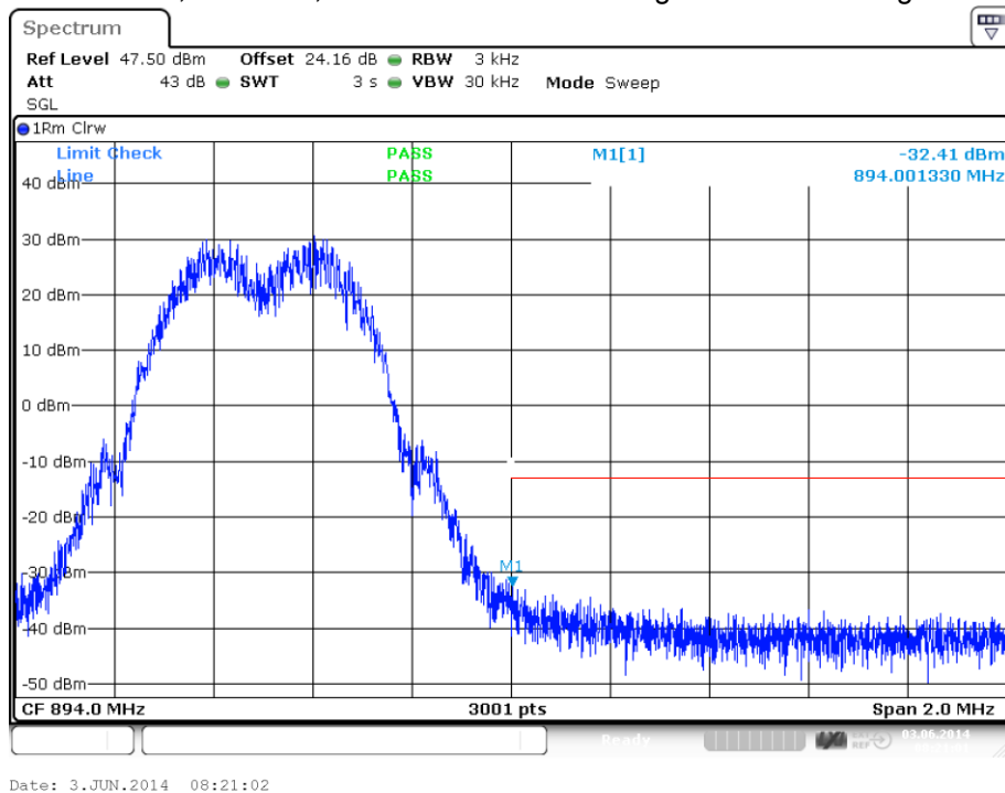
plot 7.3.1.2-#2 Spurious Emissions at Antenna Terminals: §22.917, §2.1051; RSS-131, RSS-GEN; Test results; Downlink; GSM < 1MHz to band edge Upper Band Edge
