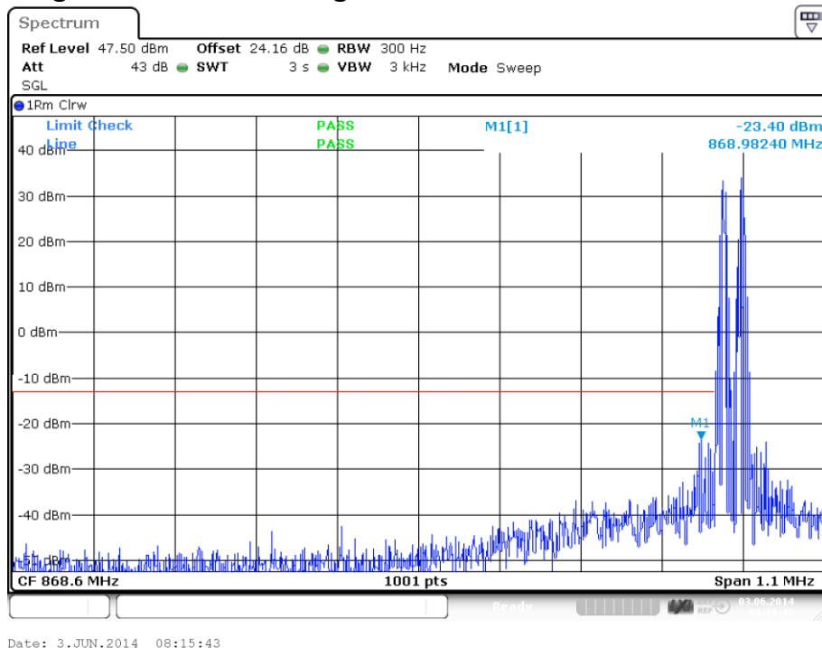
plot 7.3.1.1-#1 Spurious Emissions at Antenna Terminals: §22.917, §2.1051; RSS-131, RSS-GEN; Test results; Downlink; Analog < 1MHz to band edge Lower Band Edge
