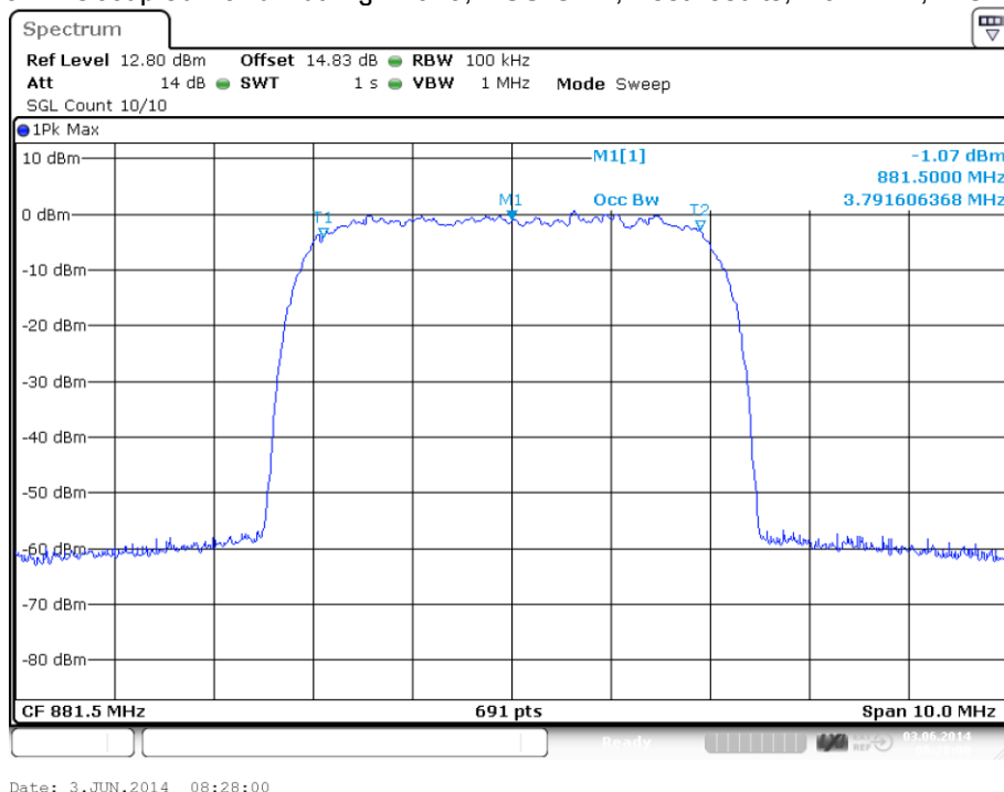
plot 6.3.1.5-#2 Occupied Bandwidth: §2.1049; RSS-GEN; Test results; Downlink; WCDMA Input
