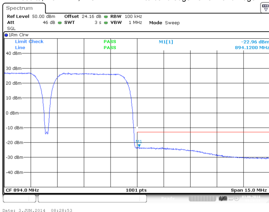
plot 7.3.1.5-#2 Spurious Emissions at Antenna Terminals: §22.917, §2.1051; RSS-131, RSS-GEN; Test results; Downlink; WCDMA < 1MHz to band edge Upper Band Edge
