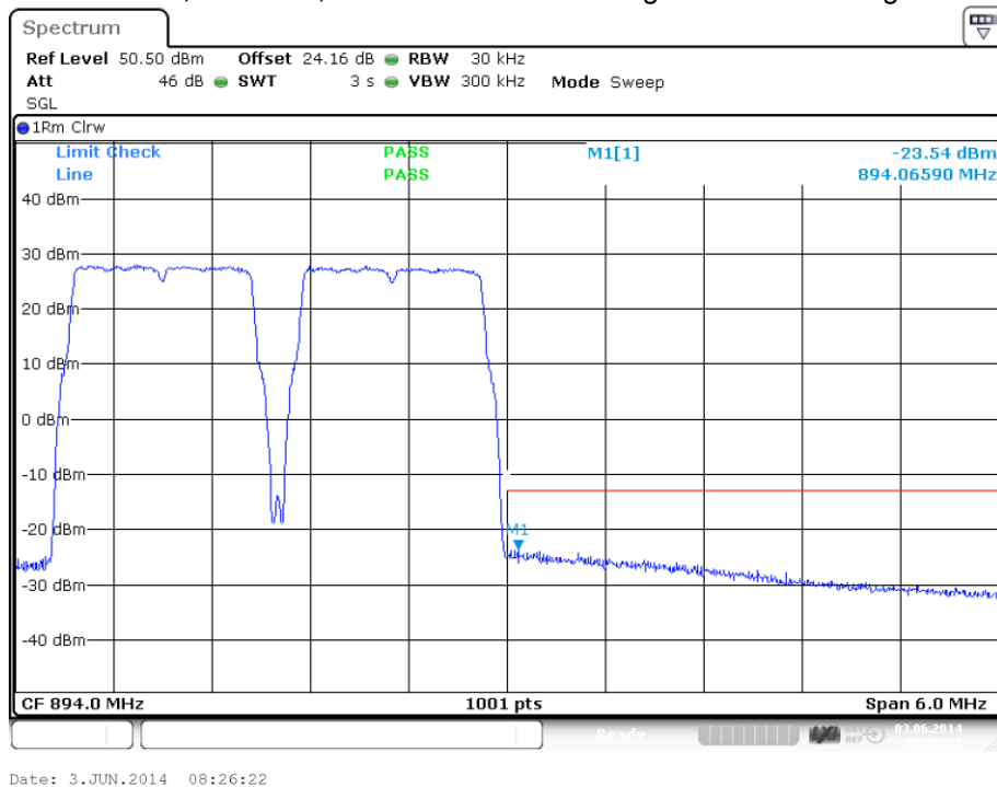
plot 7.3.1.6-#2 Spurious Emissions at Antenna Terminals: §22.917, §2.1051; RSS-131, RSS-GEN; Test results; Downlink; LTE &lt; 1MHz to band edge Upper Band Edge
