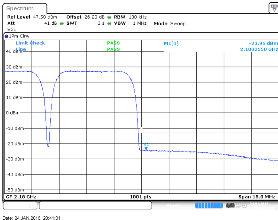
plot 8.3.1.2-#2 Intermodulation: §27.53, §2.1051; Test results; Downlink; WCDMA Upper Band Edge
