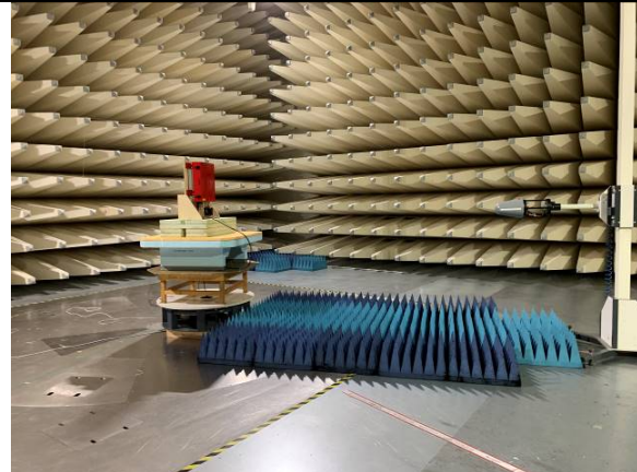
Radiated Mesaruements over 1 GHz
