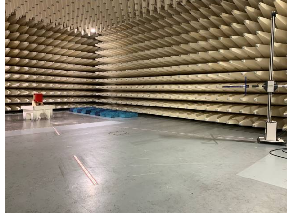
Radiated Mesaruements 30 MHz up to 1 GHz
