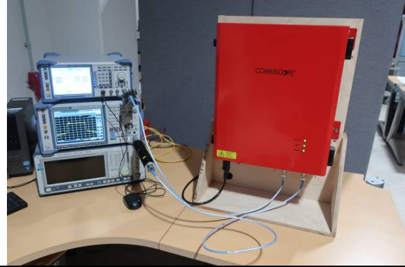
Conducted Mesaruements
