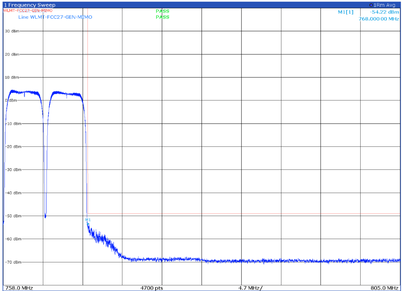
Figure 8.5-1: Antenna port 1 upper block edge intermodulation products with input signal at AGC threshold
