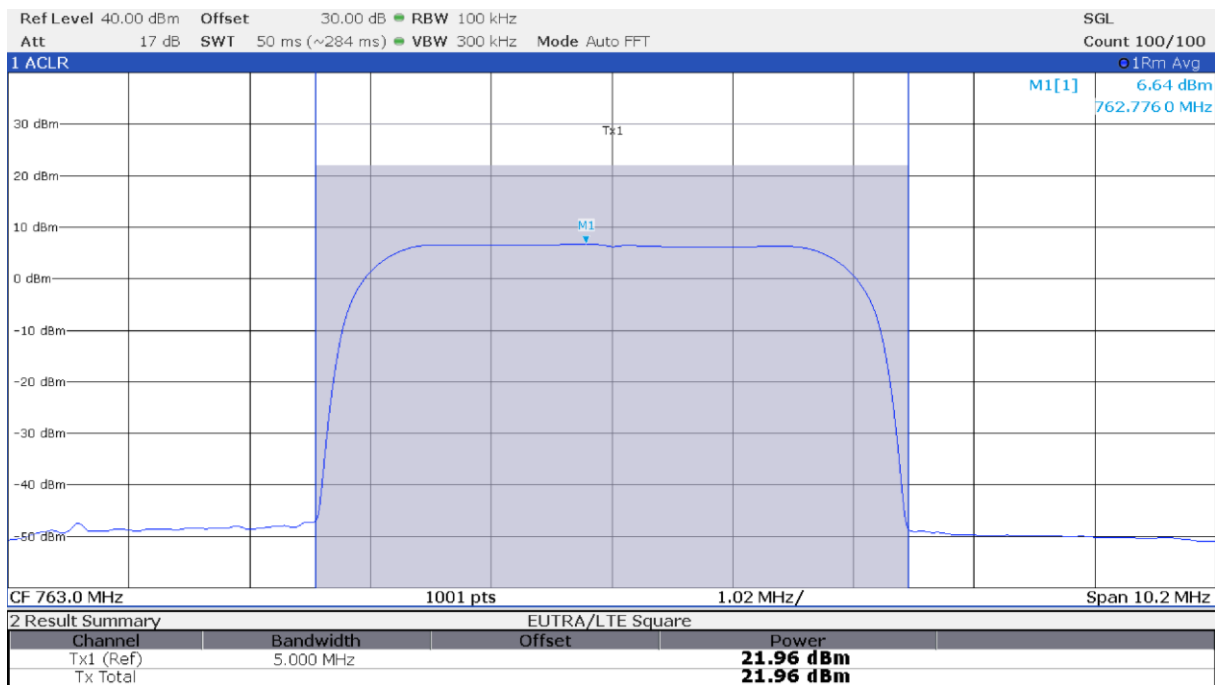
Figure 8.4-4: Output power at antenna port 1 with input signal at AGC threshold +3 dB
