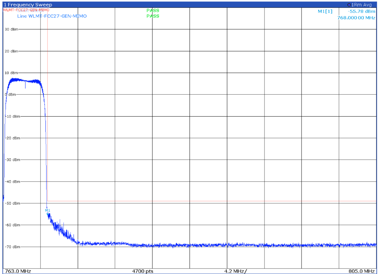
Figure 8.5-14: Antenna port 2 single carrier upper block edge with input signal at AGC threshold +3 dB
