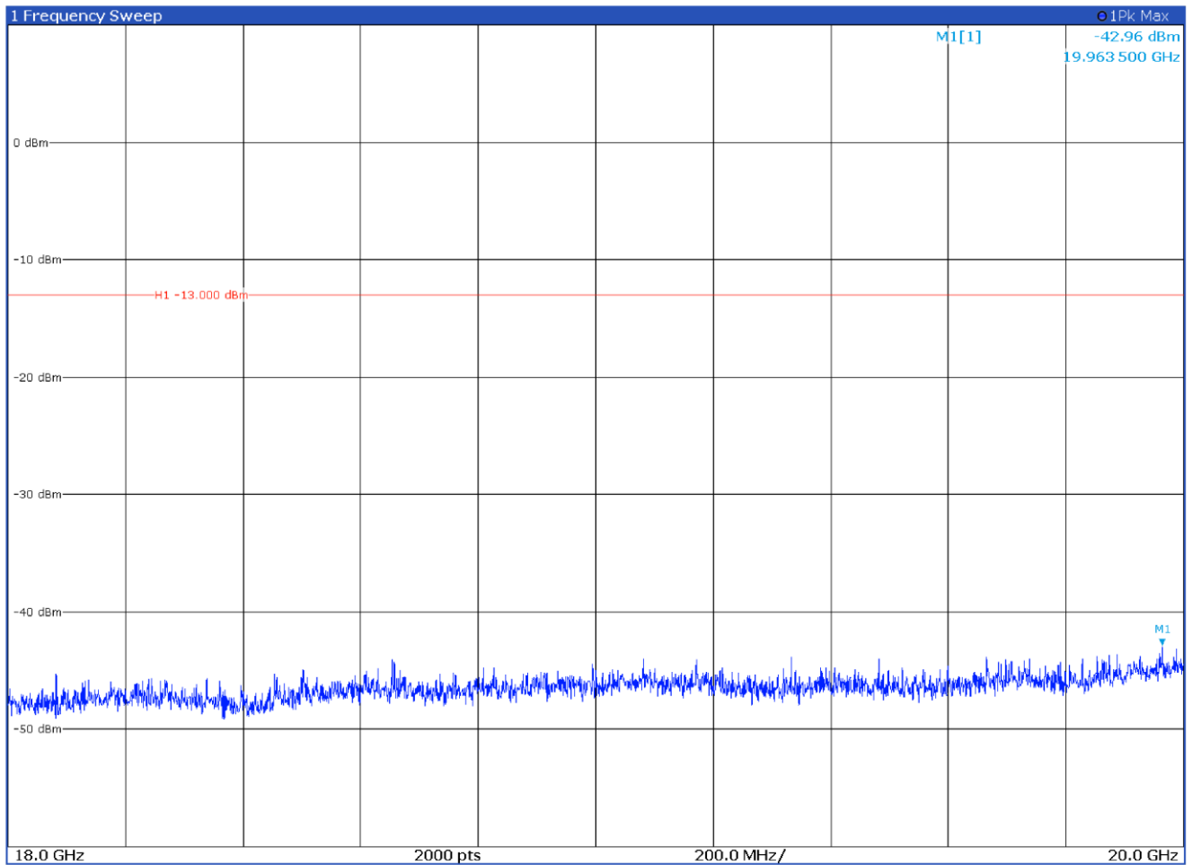
Figure 8.7-9: Radiated spurious emissions from 18 GHz to to 10th harmonic, mid channel with antenna in horizontal polarization
