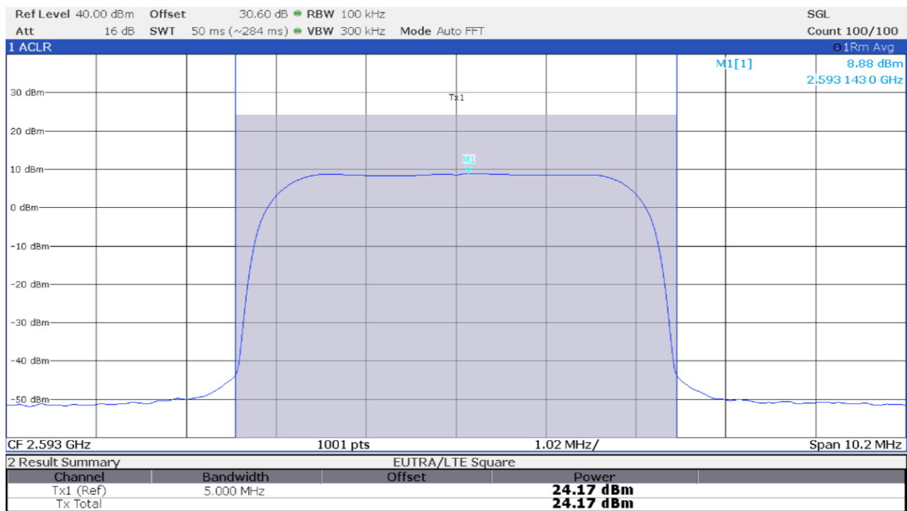
Figure 8.4-6: Output power at antenna port 2 with input signal at AGC threshold
