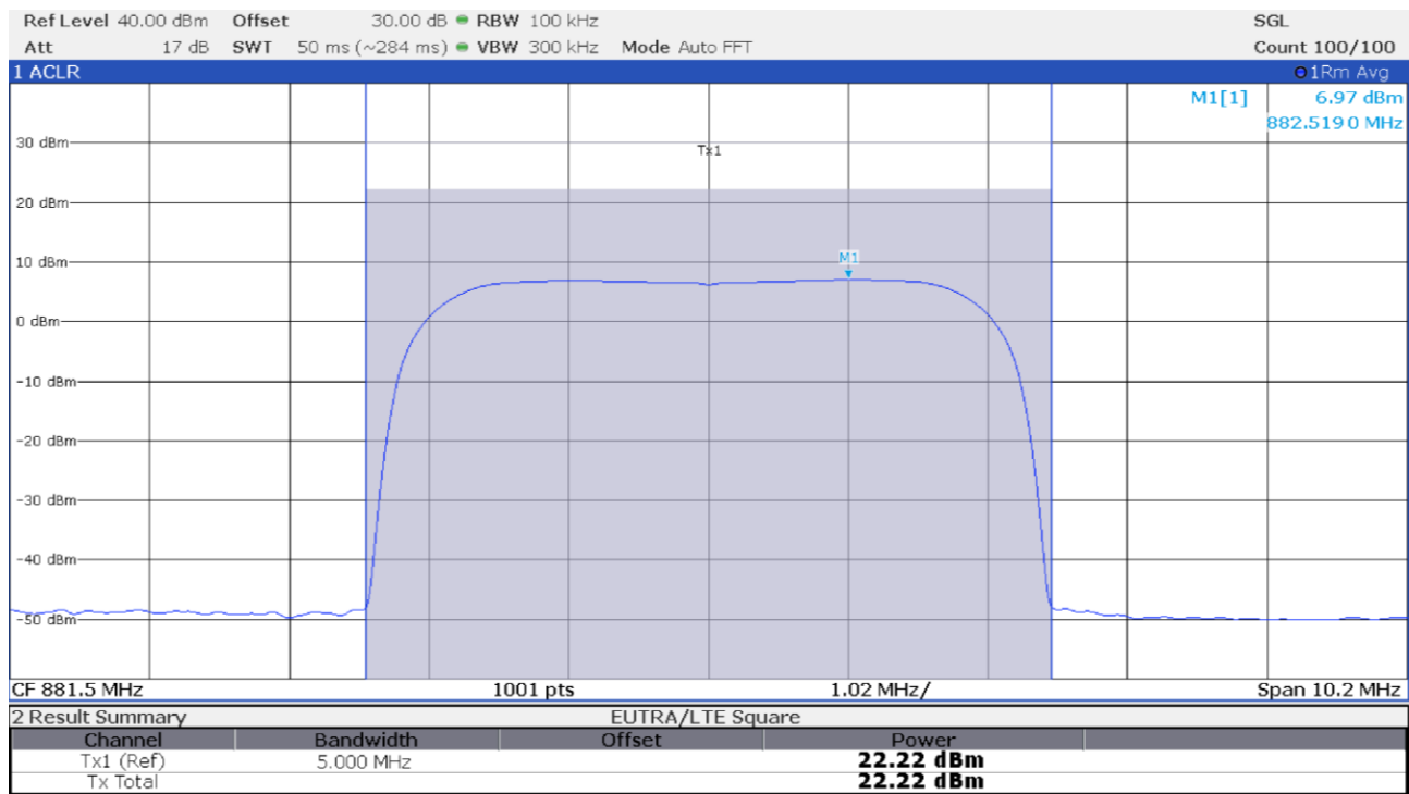
Figure 8.1-3: Antenna port 2 output spectral plot with input at AGC threshold
