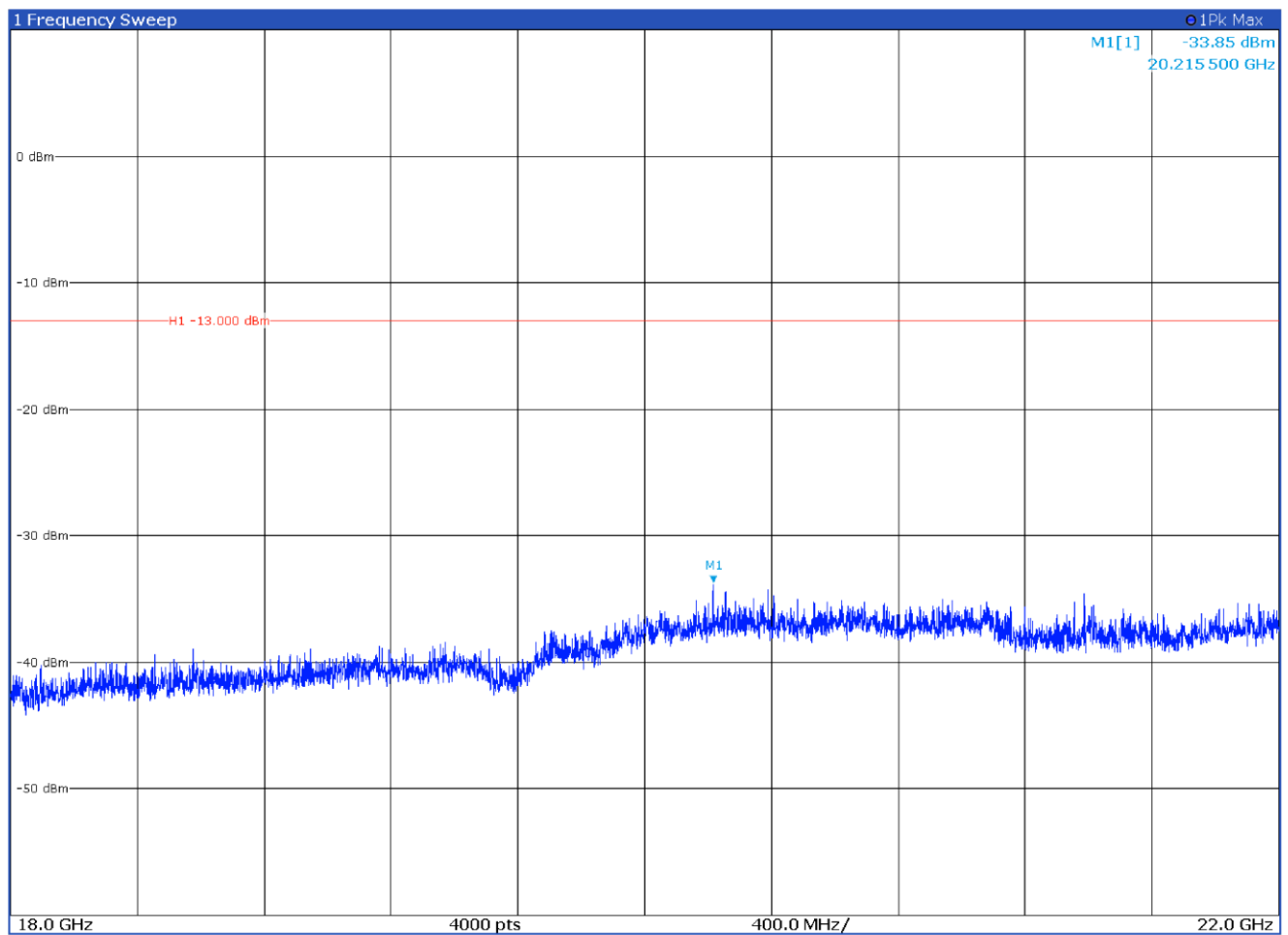
Figure 8.7-9: Radiated spurious emissions from 18 GHz to to 10th harmonic, middle channel with antenna in horizontal polarization
