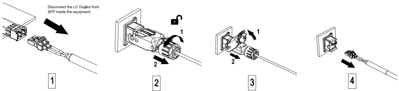
Figure 4. OCTIS Universal Lever Unmating Instructions
