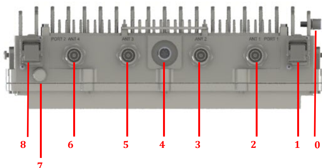
Figure 2. CAP L2 Connectors and LED (4 antennas)
