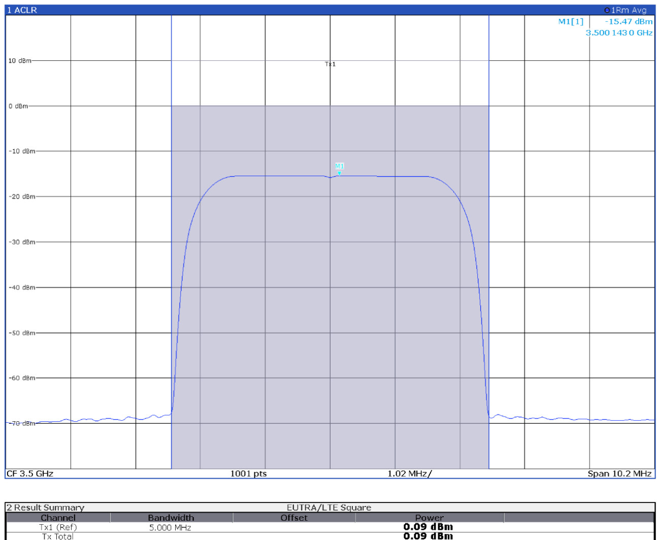
Figure 8.4-3: Input power at antenna port 1 with input signal at AGC threshold +3 dB
