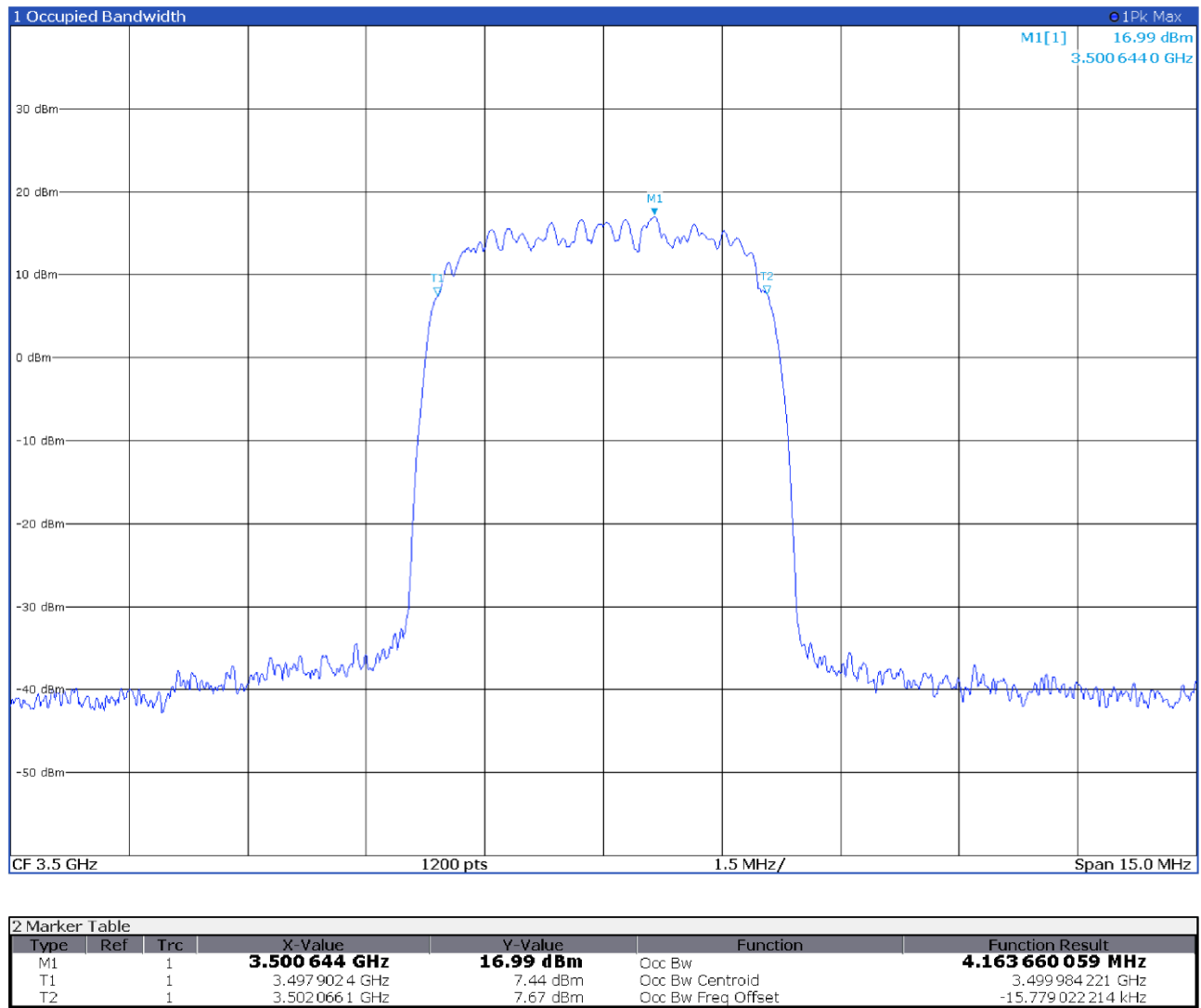
Figure 8.3-16: 99% occupied bandwidth, antenna port 2 output signal at AGC threshold +3 dB spectral plot
