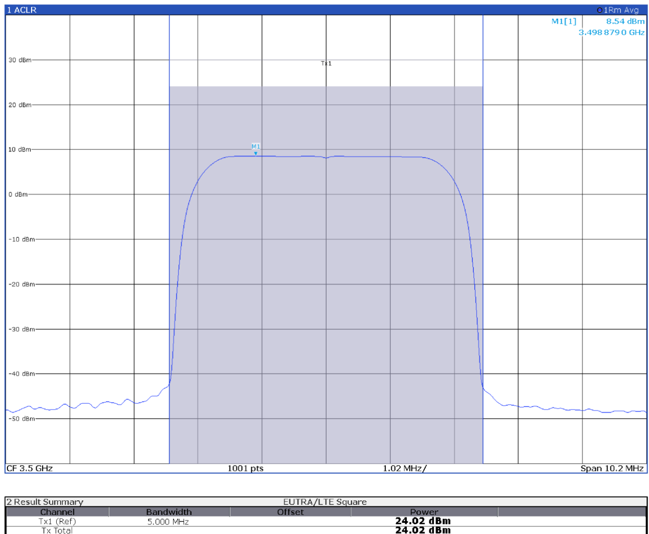
Figure 8.4-6: Output power at antenna port 2 with input signal at AGC threshold
