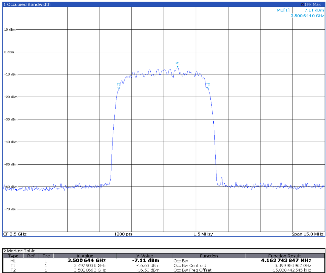
Figure 8.3-11: 99% occupied bandwidth, antenna port 1 input signal at AGC threshold +3 dB spectral plot
