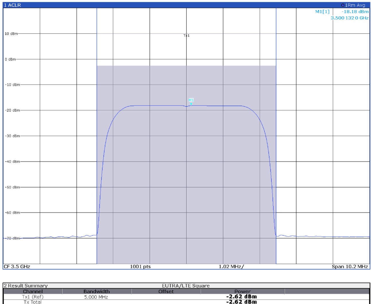
Figure 8.4-1: Input power at antenna port 1 with input signal at AGC threshold
