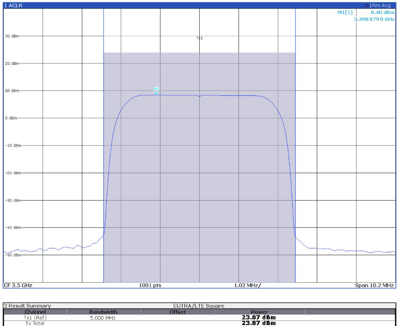
Figure 8.4-8: Output power at antenna port 2 with input signal at AGC threshold +3 dB
