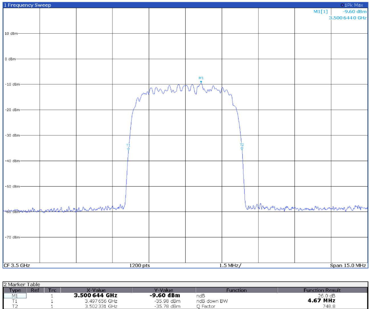
Figure 8.3-1: 26 dB occupied bandwidth, antenna port 1 input signal at AGC threshold spectral plot
