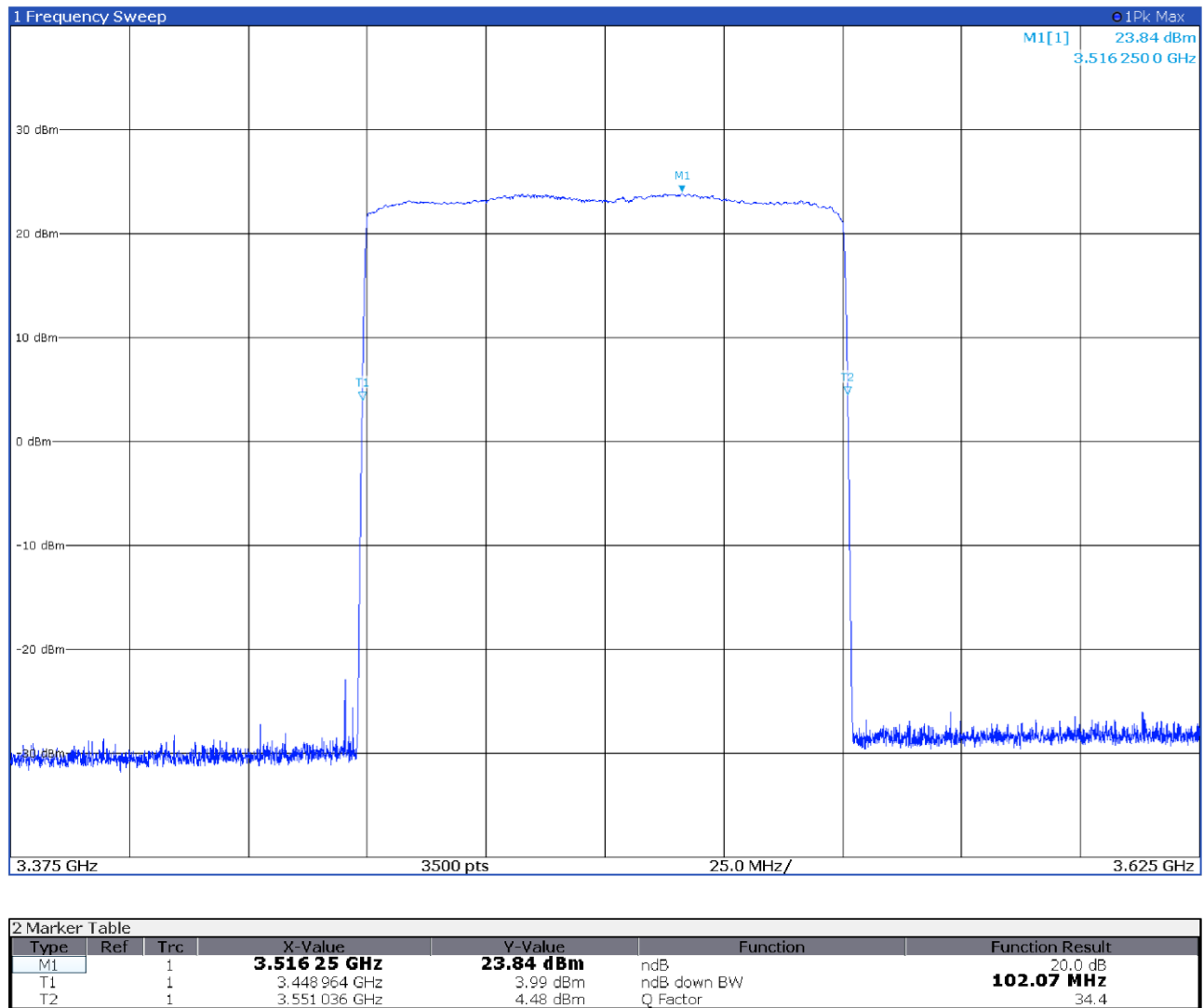
Figure 8.2-2: Out-of-band-rejection 20dB BW spectral plot for Antenna port 2
