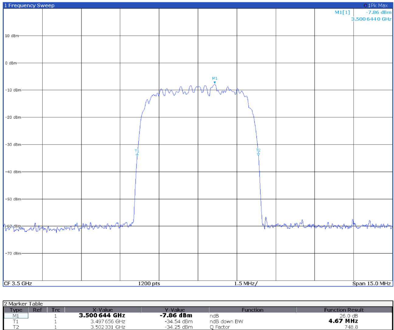
Figure 8.3-7: 26 dB occupied bandwidth, antenna port 2 input signal at AGC threshold +3 dB spectral plot
