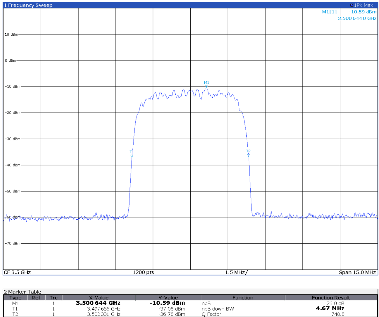
Figure 8.3-5: 26 dB occupied bandwidth, antenna port 2 input signal at AGC threshold spectral plot
