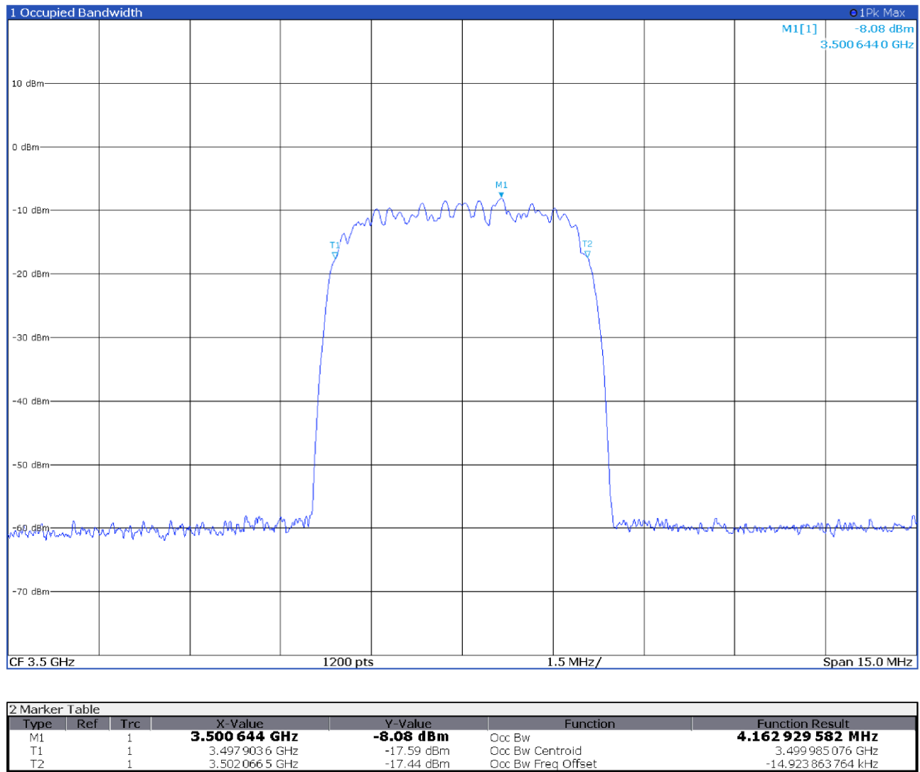
Figure 8.3-15: 99% occupied bandwidth, antenna port 2 input signal at AGC threshold +3 dB spectral plot
