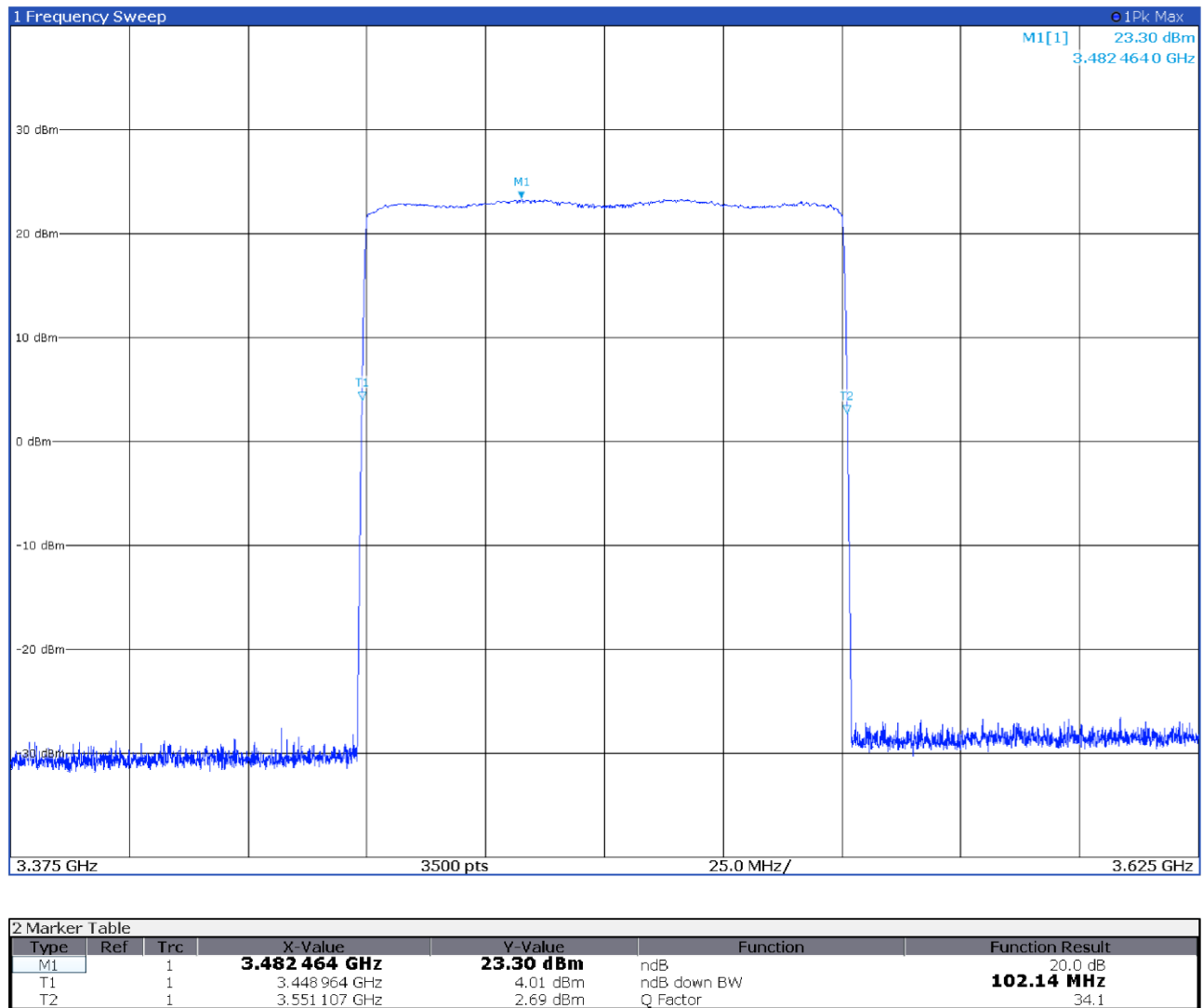
Figure 8.2-1: Out-of-band-rejection 20dB BW spectral plot for Antenna port 1
