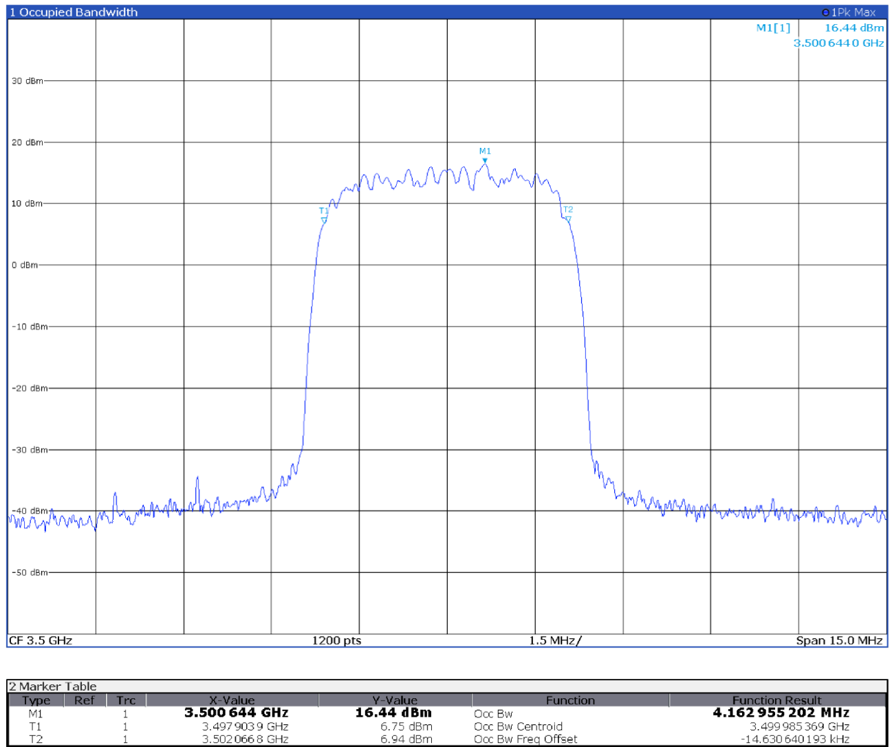
Figure 8.3-10: 99% occupied bandwidth, antenna port 1 output signal at AGC threshold spectral plot
