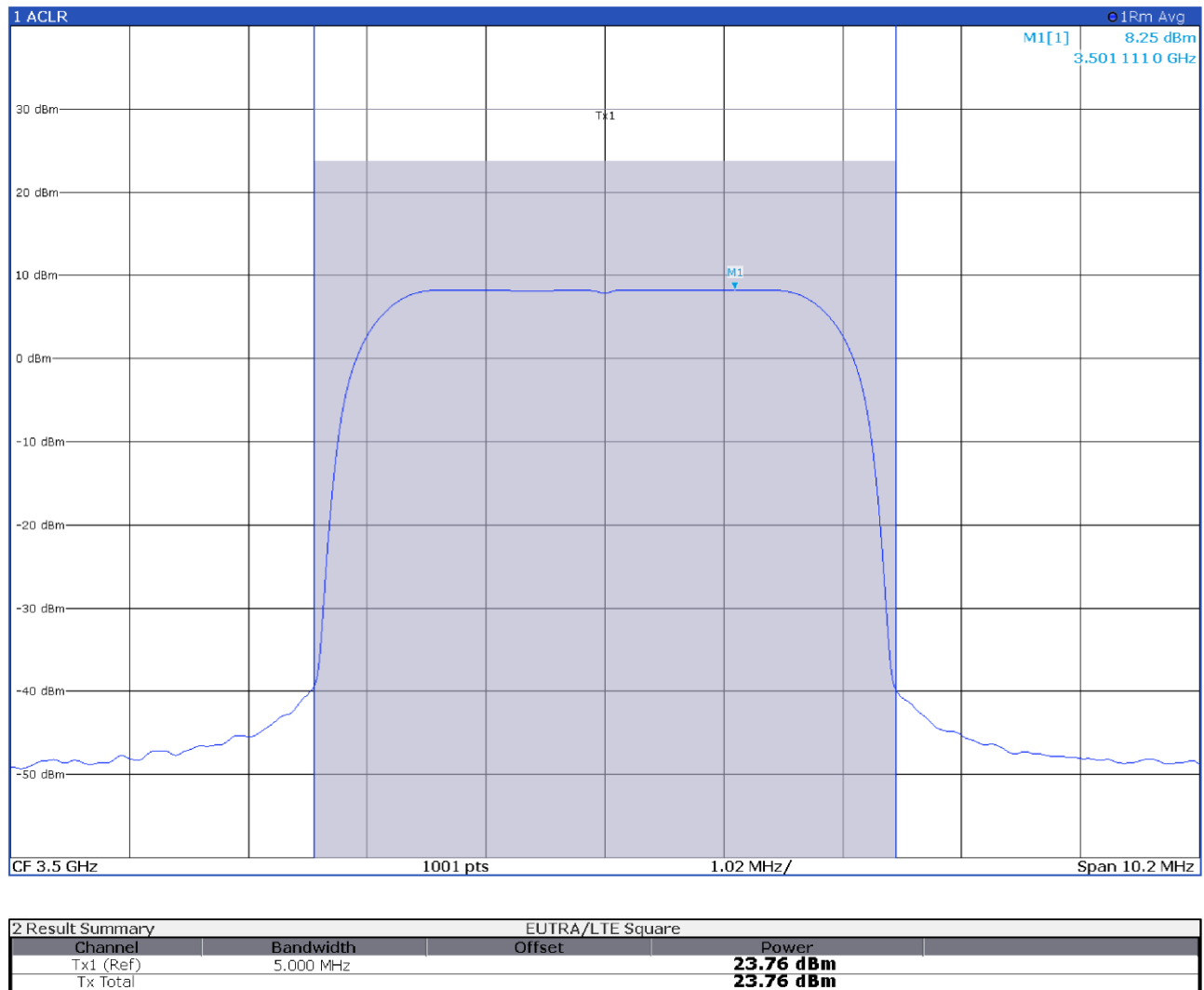
Figure 8.1-2: Antenna port 1 output spectral plot with input at AGC threshold +1 dBm
