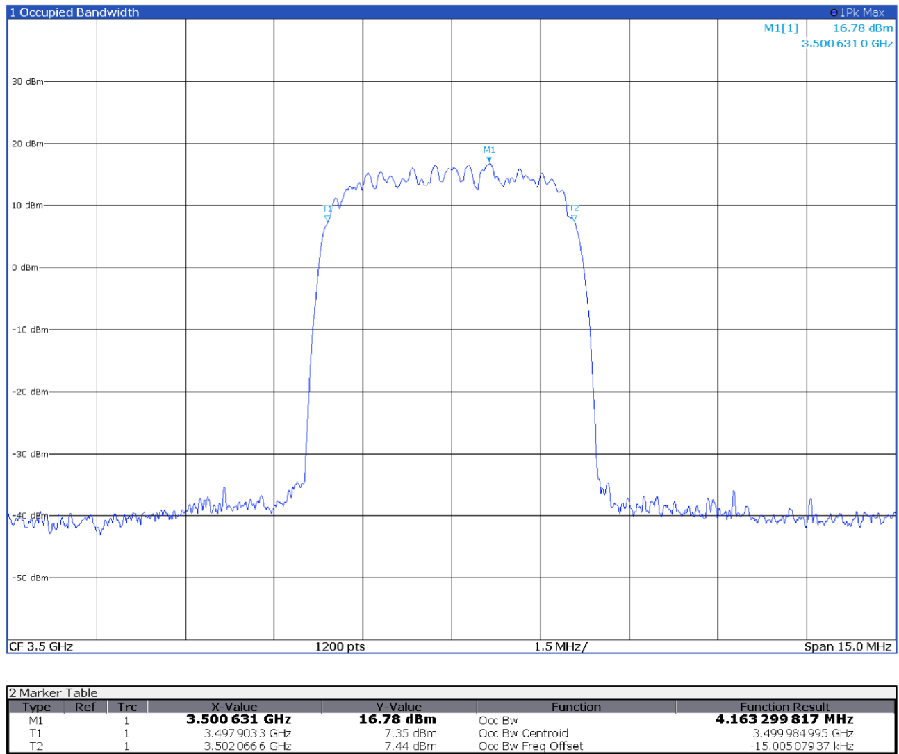
Figure 8.3-14: 99% occupied bandwidth, antenna port 2 output signal at AGC threshold spectral plot
