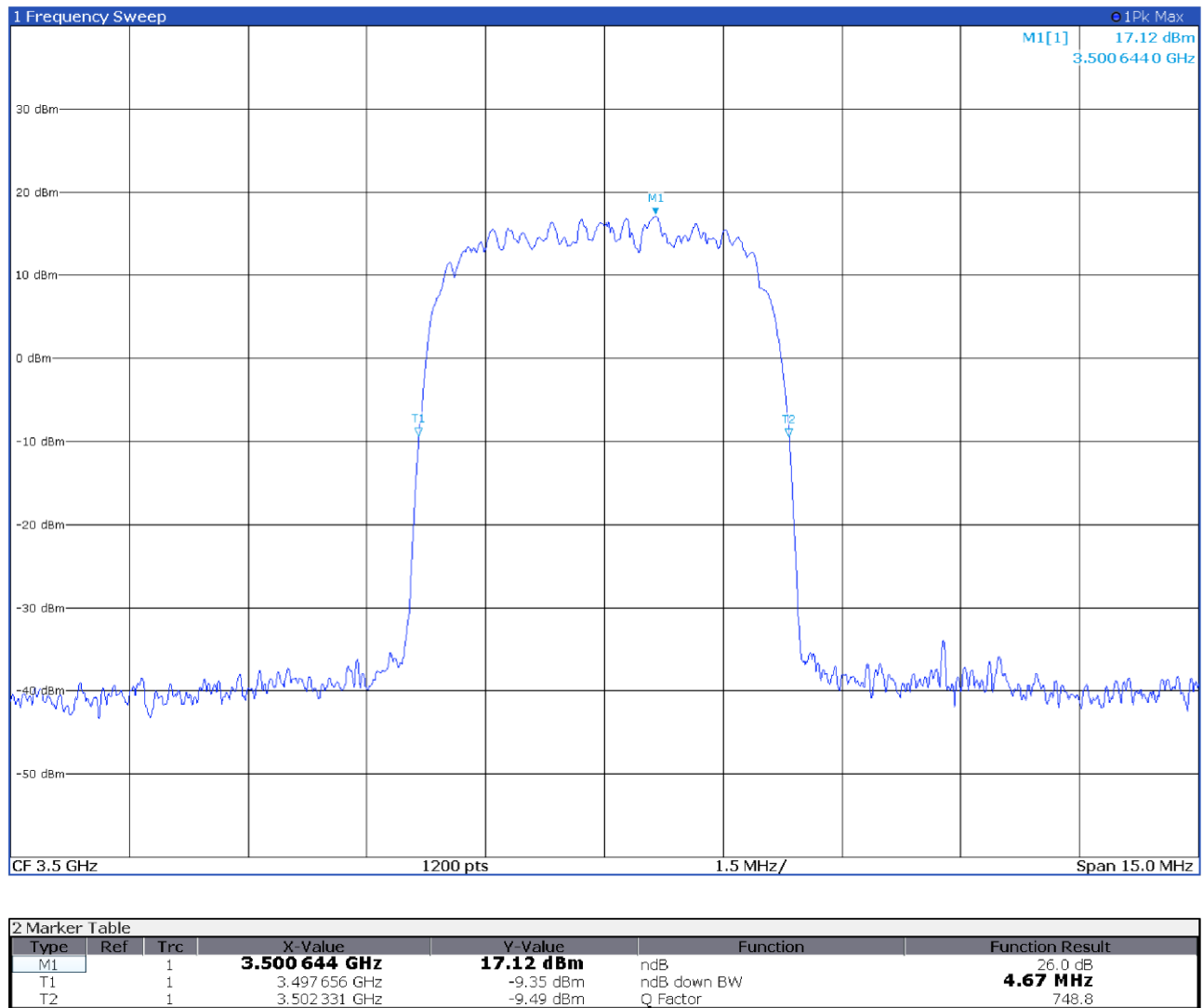
Figure 8.3-6: 26 dB occupied bandwidth, antenna port 2 output signal at AGC threshold spectral plot
