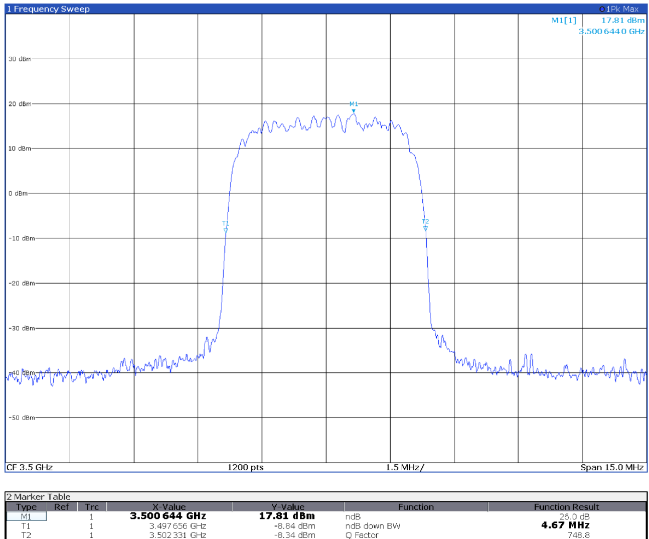
Figure 8.3-2: 26 dB occupied bandwidth, antenna port 1 output signal at AGC threshold spectral plot
