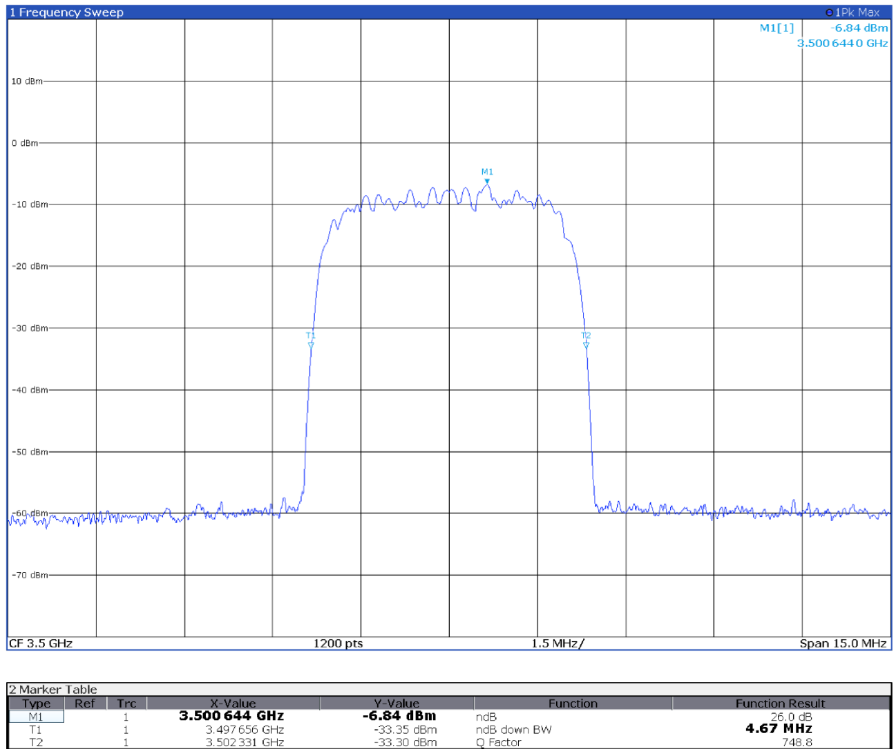
Figure 8.3-3: 26 dB occupied bandwidth, antenna port 1 input signal at AGC threshold +3 dB spectral plot
