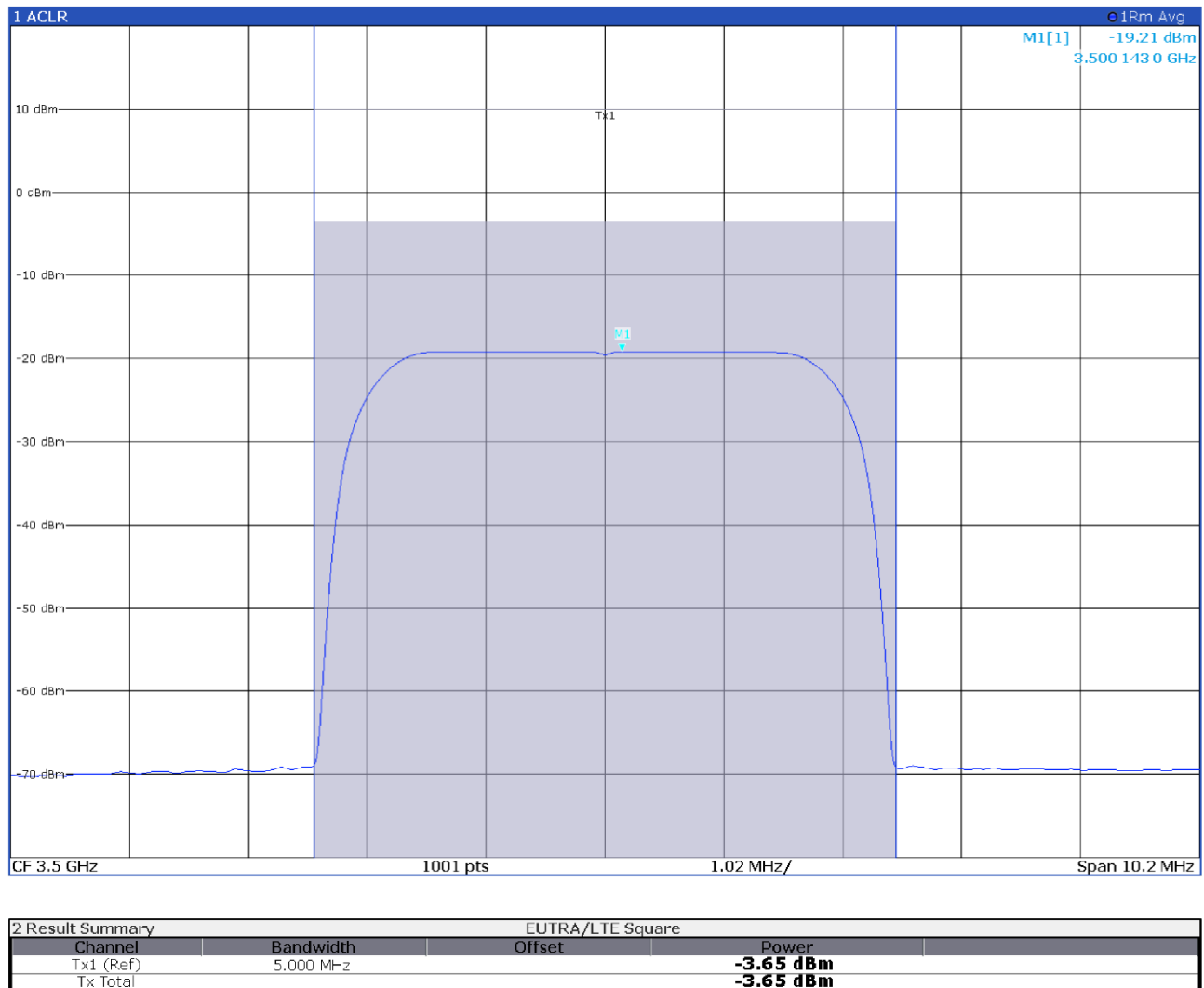
Figure 8.4-5: Input power at antenna port 2 with input signal at AGC threshold
