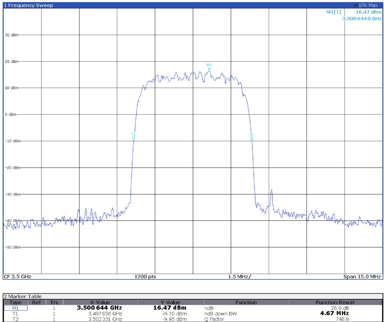
Figure 8.3-8: 26 dB occupied bandwidth, antenna port 2 output signal at AGC threshold +3 dB spectral plot
