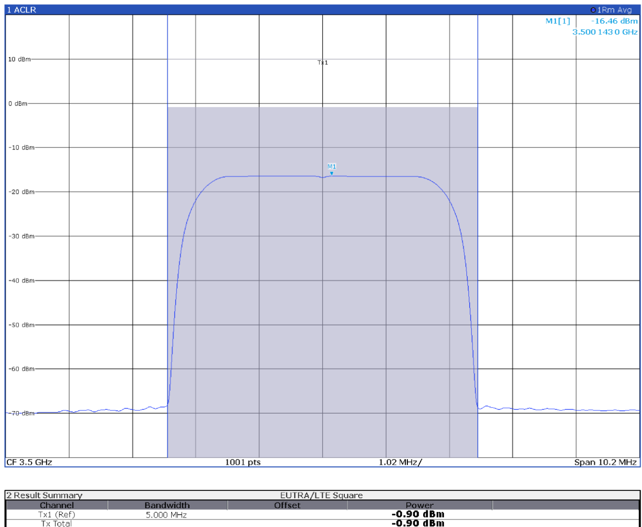
Figure 8.4-7: Input power at antenna port 2 with input signal at AGC threshold +3 dB
