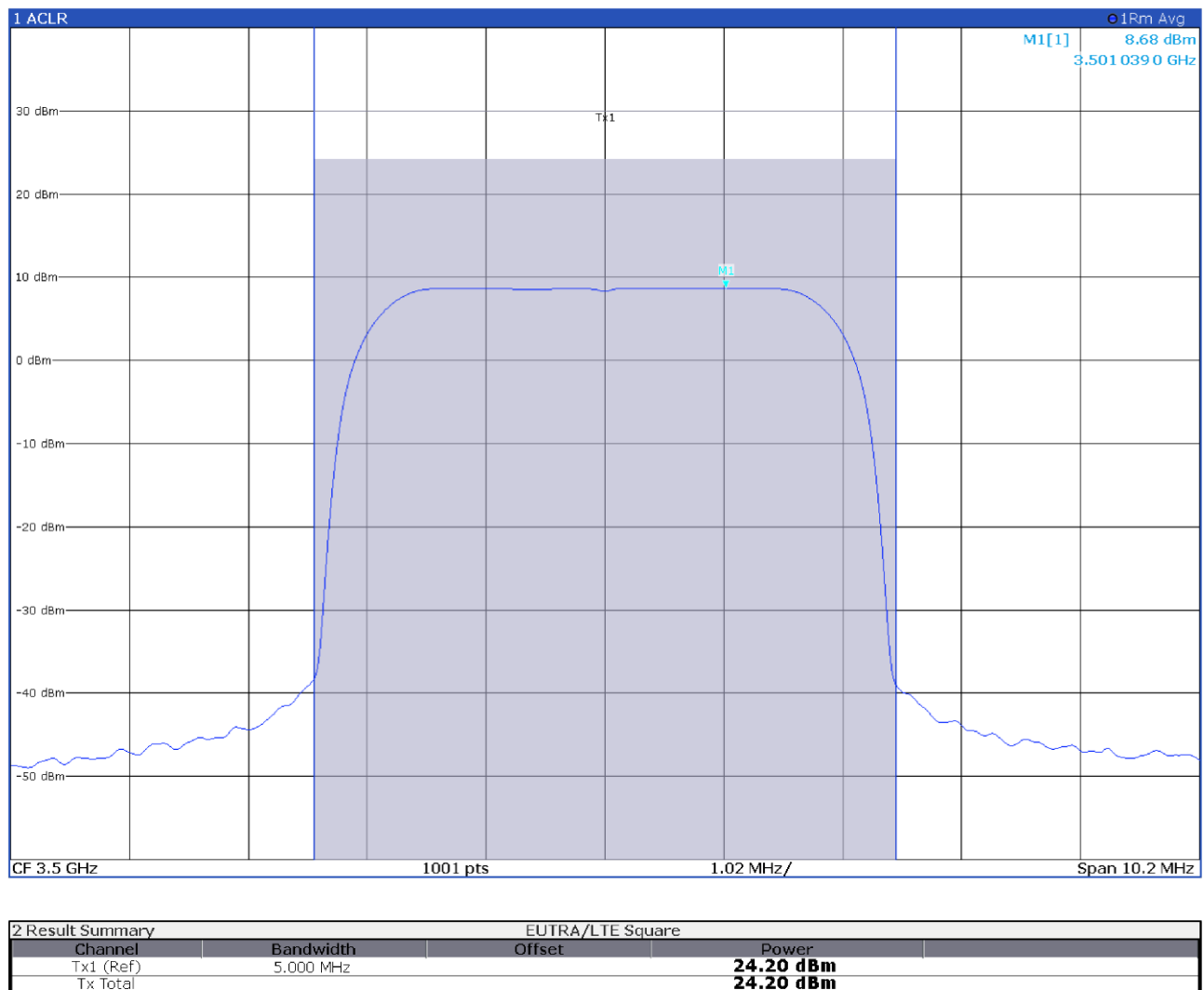
Figure 8.4-4: Output power at antenna port 1 with input signal at AGC threshold +3 dB
