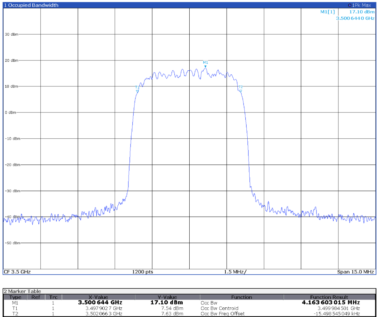
Figure 8.3-12: 99% occupied bandwidth, antenna port 1 output signal at AGC threshold +3 dB spectral plot
