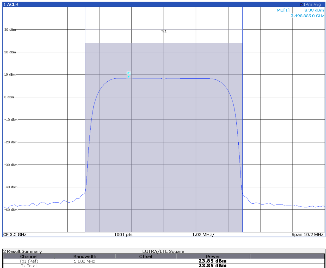
Figure 8.1-4: Antenna port 2 output spectral plot with input at AGC threshold +1 dBm
