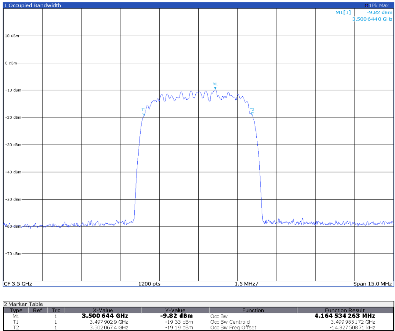
Figure 8.3-9: 99% occupied bandwidth, antenna port 1 input signal at AGC threshold spectral plot
