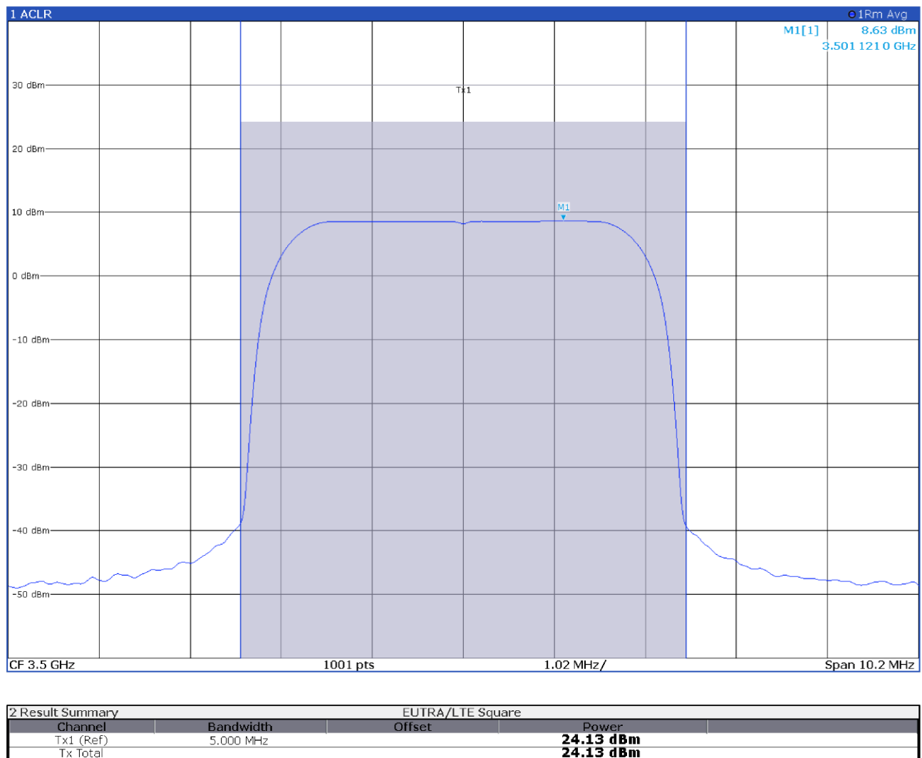
Figure 8.4-2: Output power at antenna port 1 with input signal at AGC threshold
