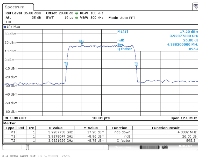
Output Signal
