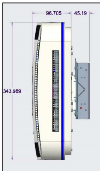
FIGURE 2: Dimensions of the UAP2 with Mounting Kit
