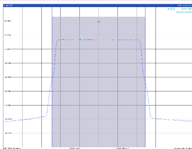
TM3p1, 5 MHz, high channel
