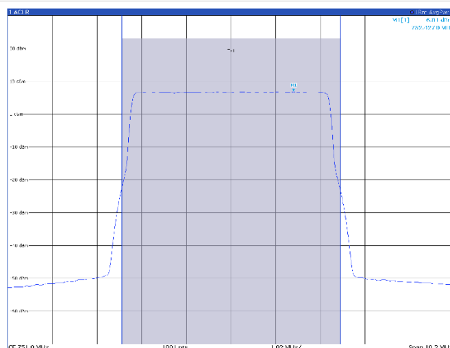
TM3p1a, 5 MHz, mid channel
