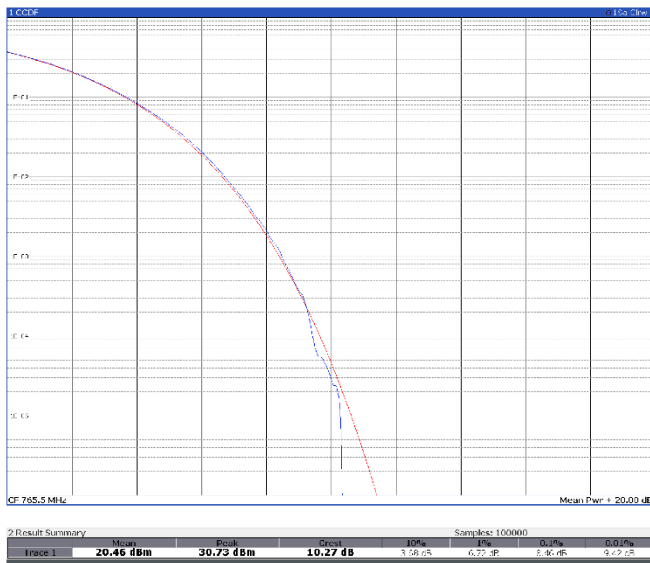
TM3p3, 5 MHz, mid channel
