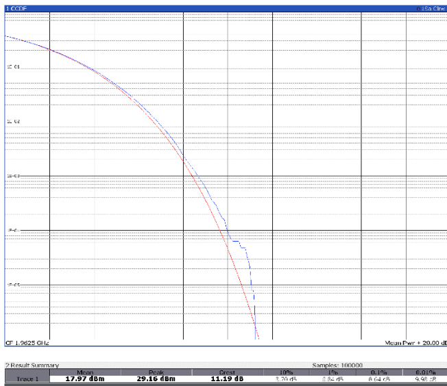
TM3p3, 15 MHz, mid channel
