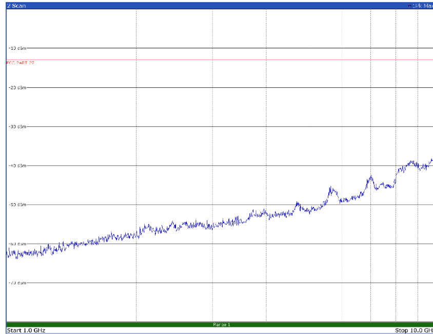
Radiated emissions spectral plot (1 GHz - 10 GHz), vertical polarization, mid channel, TM3p1 modulation
