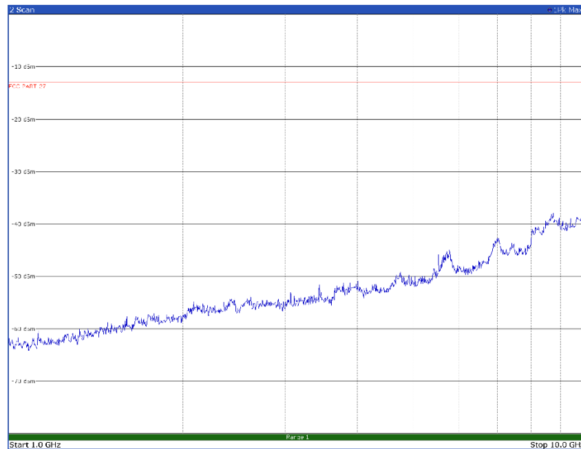
Radiated emissions spectral plot (1 GHz - 10 GHz), horizontal polarization, mid channel, TM3p1 modulation
