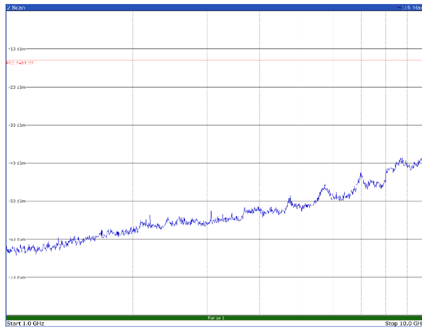
Radiated emissions spectral plot (1 GHz - 10 GHz), horizontal polarization, low channel, TM3p1 modulation
