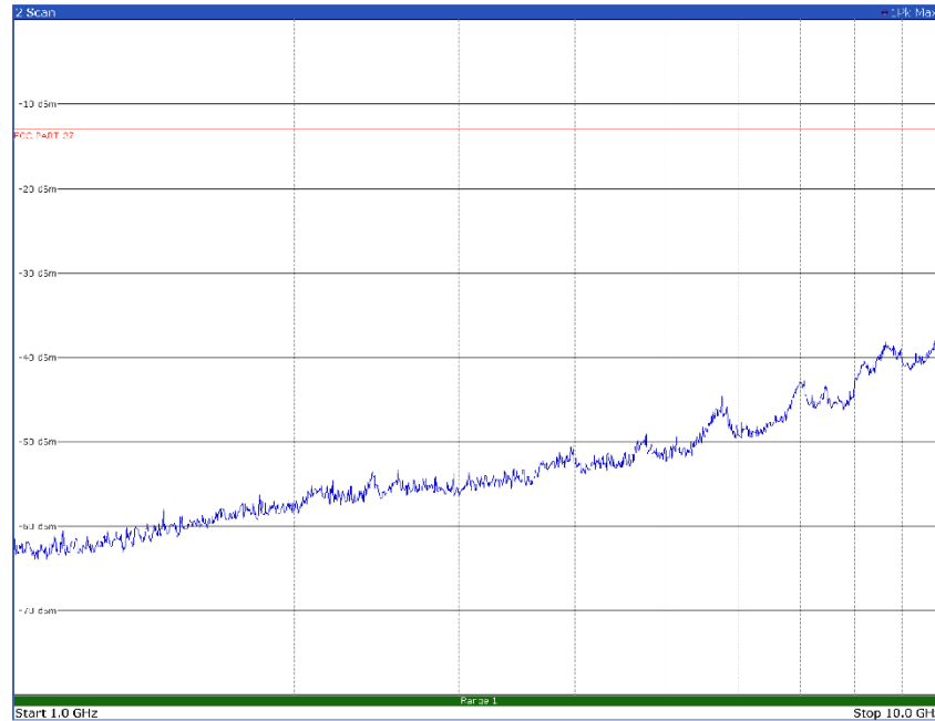
Radiated emissions spectral plot (1 GHz - 10 GHz), vertical polarization, low channel, TM3p1 modulation
