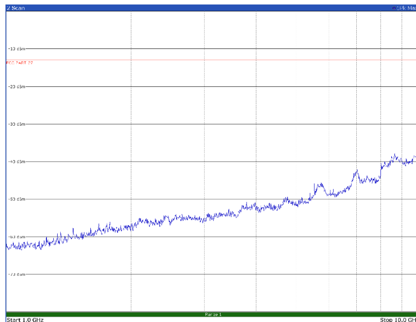
Radiated emissions spectral plot (1 GHz - 10 GHz), horizontal polarization, high channel, TM3p1 modulation
