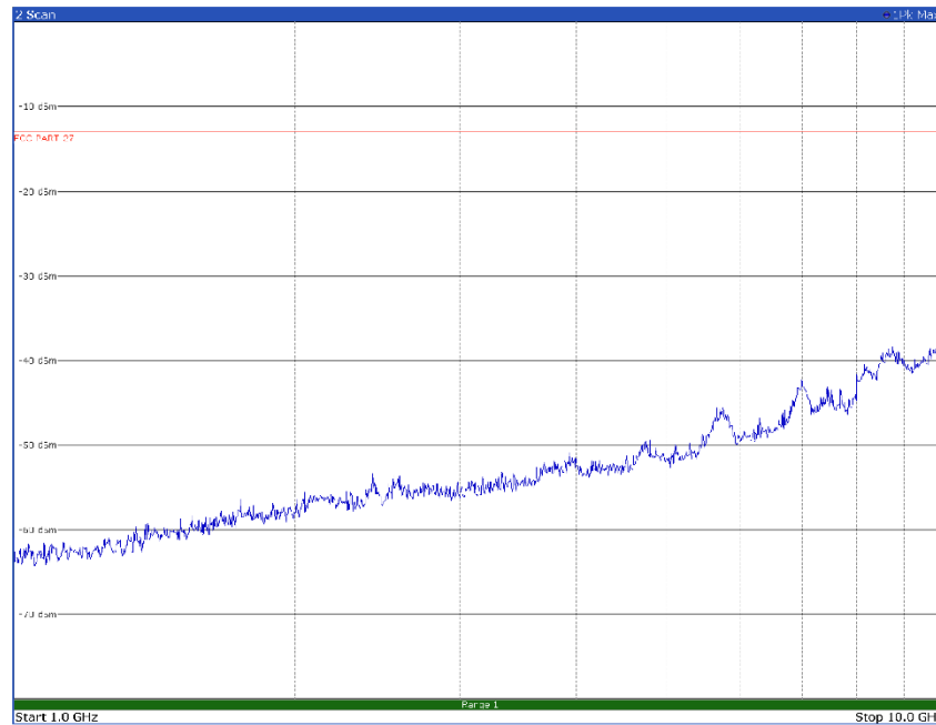
Radiated emissions spectral plot (1 GHz - 10 GHz), vertical polarization, high channel, TM3p1 modulation
