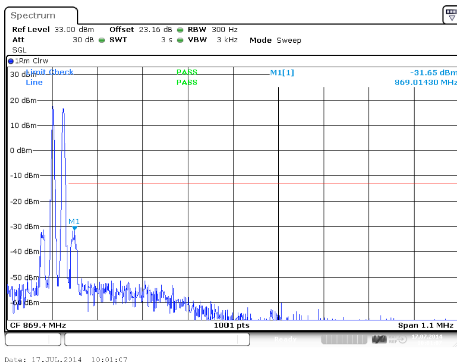
plot 7.3.1.2-#2 Spurious Emissions at Antenna Terminals: §90.210, §2.1051; Test results; Downlink; APCO Phase1 C4FM < 1MHz to band edge; Upper Band Edge
