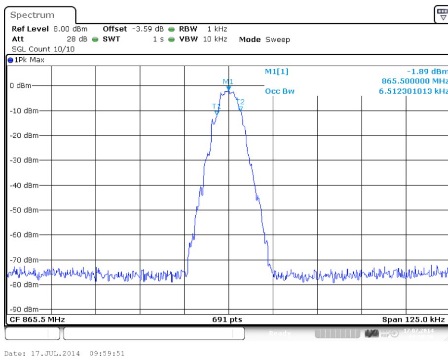
plot 6.3.1.2-#2 Occupied Bandwidth: $90.210, $2.1049; Test results; Downlink; APCO Phase1 C4FM Input
