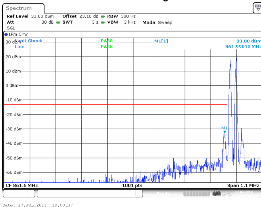
plot 7.3.1.2-#1 Spurious Emissions at Antenna Terminals: §90.210, §2.1051; Test results; Downlink; APCO Phase1 C4FM < 1MHz to band edge; Lower Band Edge
