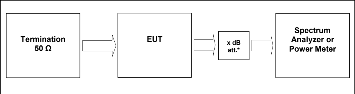
External Attenuator DL x dB = 0 dB figure 9-#1 Test setup: Noise floor
