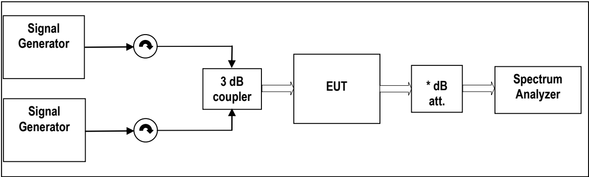
External Attenuator DL x dB = 20 dB figure 7-#1 Test setup: Spurious Emissions at Antenna Terminals: §90.543, §2.1051
