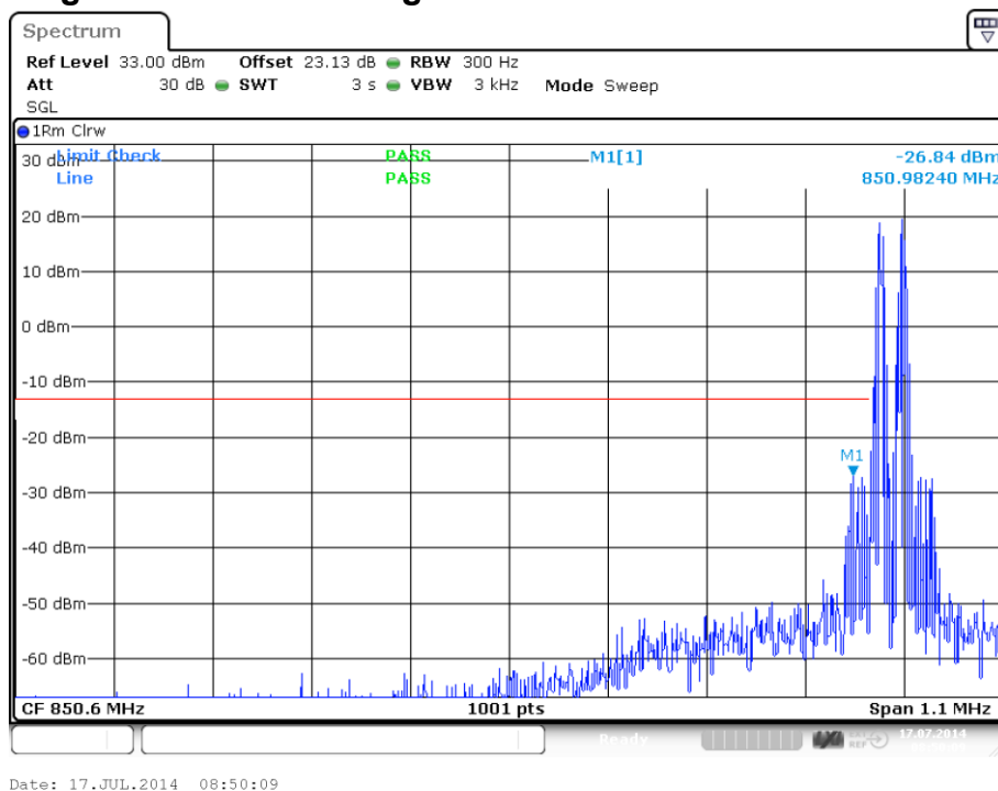
plot 7.3.1.1-#1 Spurious Emissions at Antenna Terminals: §90.210, §2.1051; Test results; Downlink; Analog < 1MHz to band edge; Lower Band Edge
