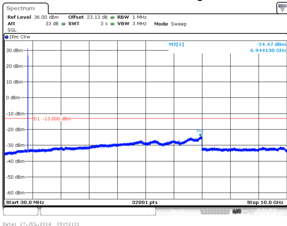
plot 7.3.1.6-#1 Spurious Emissions at Antenna Terminals: §90.210, §2.1051; Test results; Downlink; APCO Phase2 H-DQPSK > 1MHz to band edge
