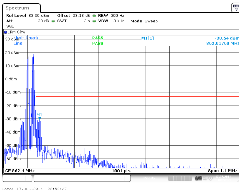
plot 7.3.1.1-#2 Spurious Emissions at Antenna Terminals: §90.210, §2.1051; Test results; Downlink; Analog < 1MHz to band edge; Upper Band Edge
