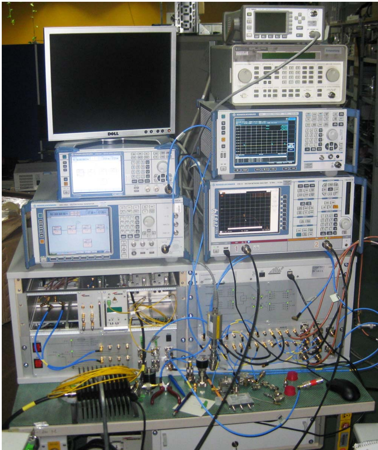
Measurement Equipment
