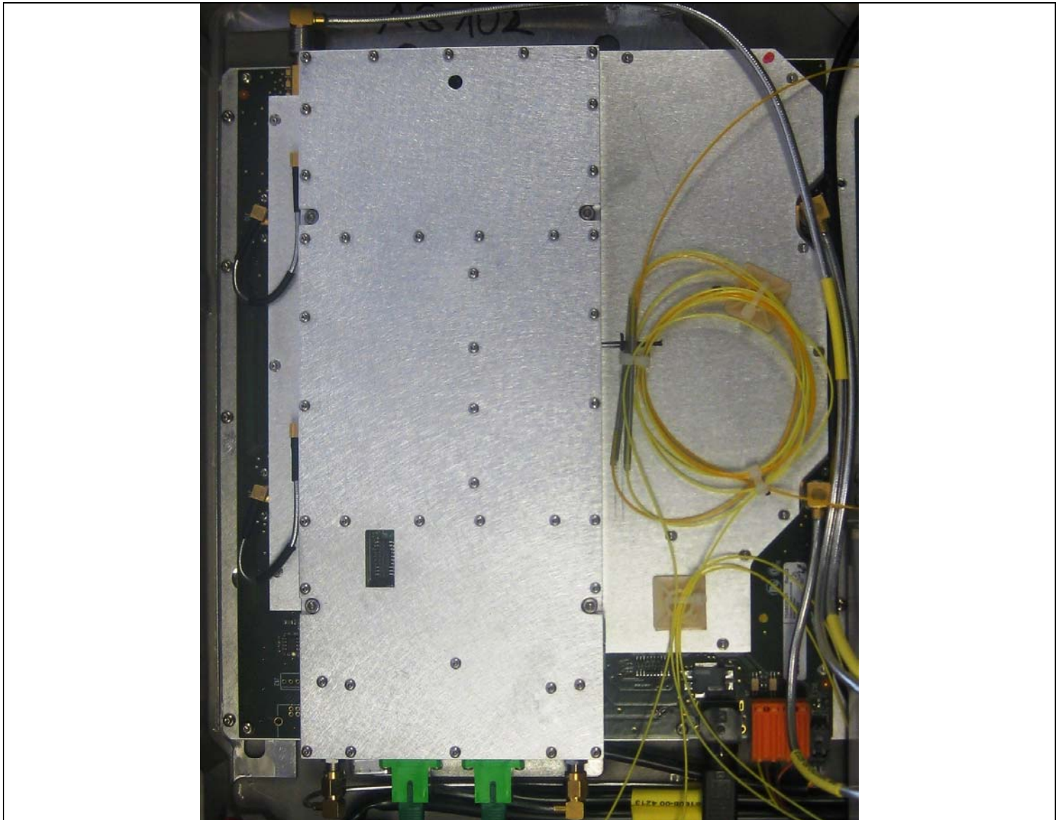
Amplification Part for 70/80 and optical module
