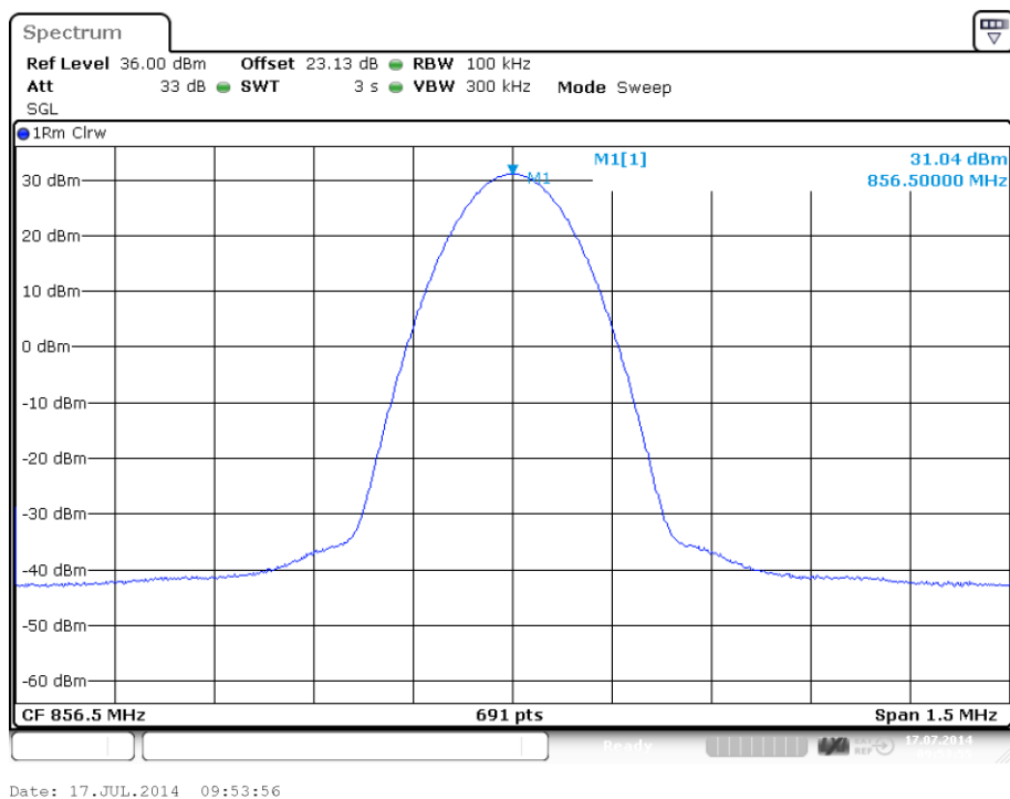
plot 5.3.1.2-#1 RF Power Out: §90.635, §2.1046; Test Results; Downlink; APCO Phase1 C4FM
