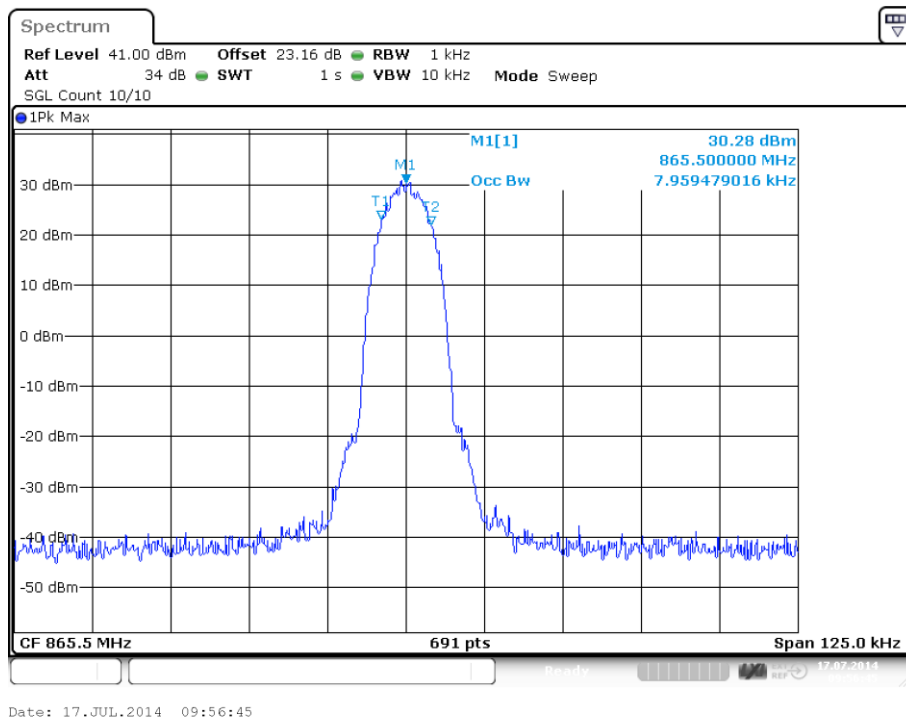
plot 6.3.1.3-#1 Occupied Bandwidth: $90.210, $2.1049; Test results; Downlink; APCO Phase2 H-DQPSK Output
