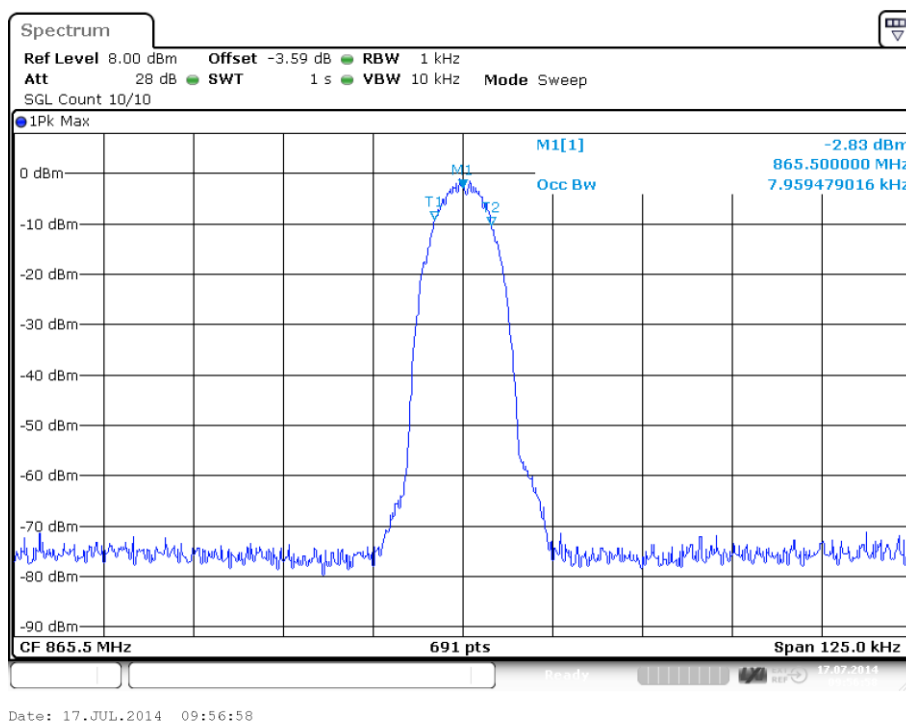
plot 6.3.1.3-#2 Occupied Bandwidth: $90.210, $2.1049; Test results; Downlink; APCO Phase2 H-DQPSK Input
