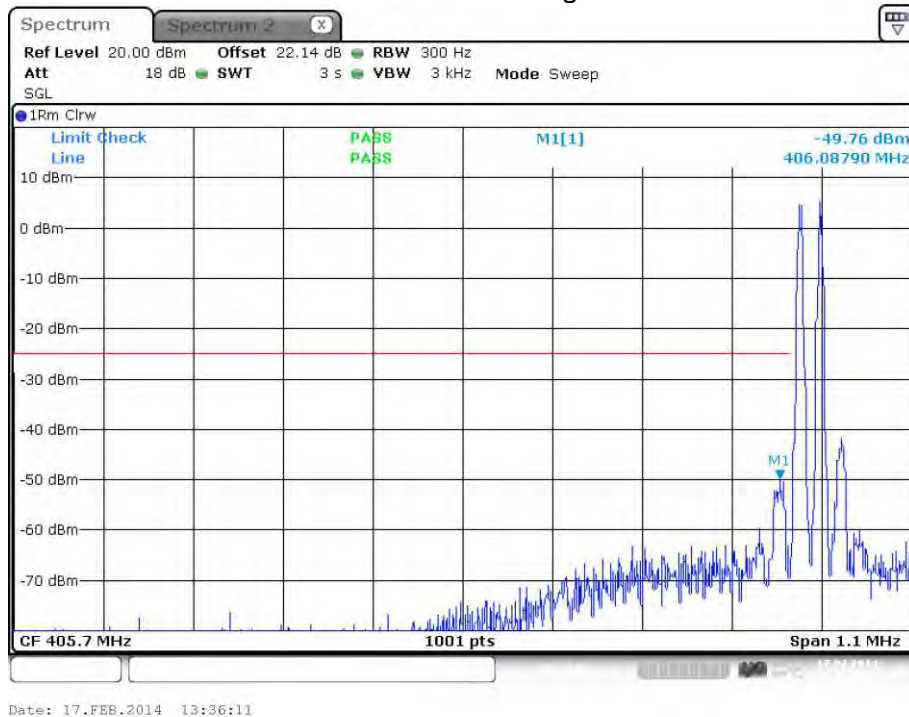
plot 7.3.1.1-#1 Spurious Emissions at Antenna Terminals: §90.210, §2.1051; Test results; Downlink; Band # 1; APCO Phase1 C4FM < 1MHz to band edge; Lower Band Edge
