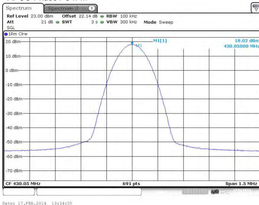
plot 5.3.1.1-#1 RF Power Out: §90.635, §2.1046; Test Results; Downlink; Band # 1; APCO Phase1 C4FM
