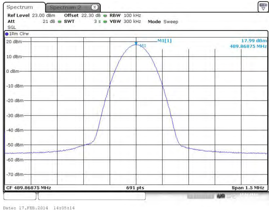
plot 5.3.1.4-#1 RF Power Out: $90.635, $2.1046; Test Results; Downlink; Band # 4; APCO Phase1 C4FM
