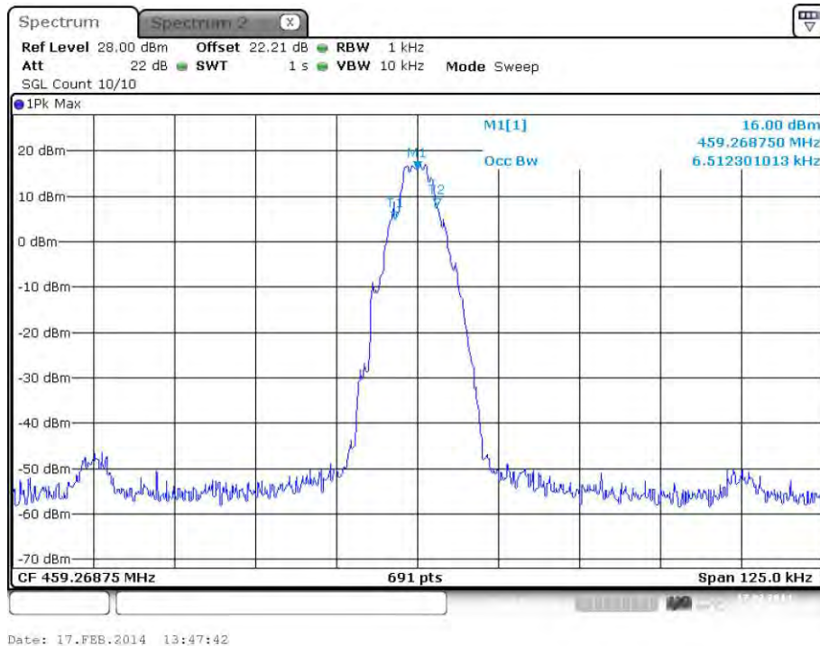
plot 6.3.1.2-#1 Occupied Bandwidth: §90.210, §2.1049; Test results; Downlink; Band # 2; APCO Phase1 C4FM; Output
