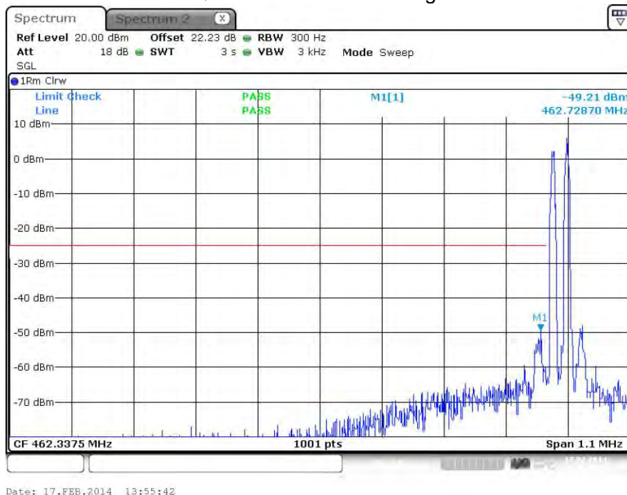
plot 7.3.1.3-#1 Spurious Emissions at Antenna Terminals: §90.210, §2.1051; Test results; Downlink; Band # 3; APCO Phase2 H-DQPSK < 1MHz to band edge; Lower Band Edge
