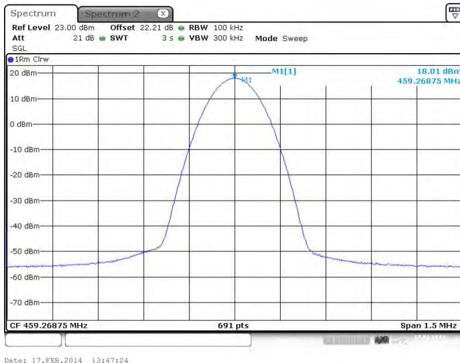
plot 5.3.1.2-#1 RF Power Out: §90.635, §2.1046; Test Results; Downlink; Band # 2; APCO Phase1 C4FM
