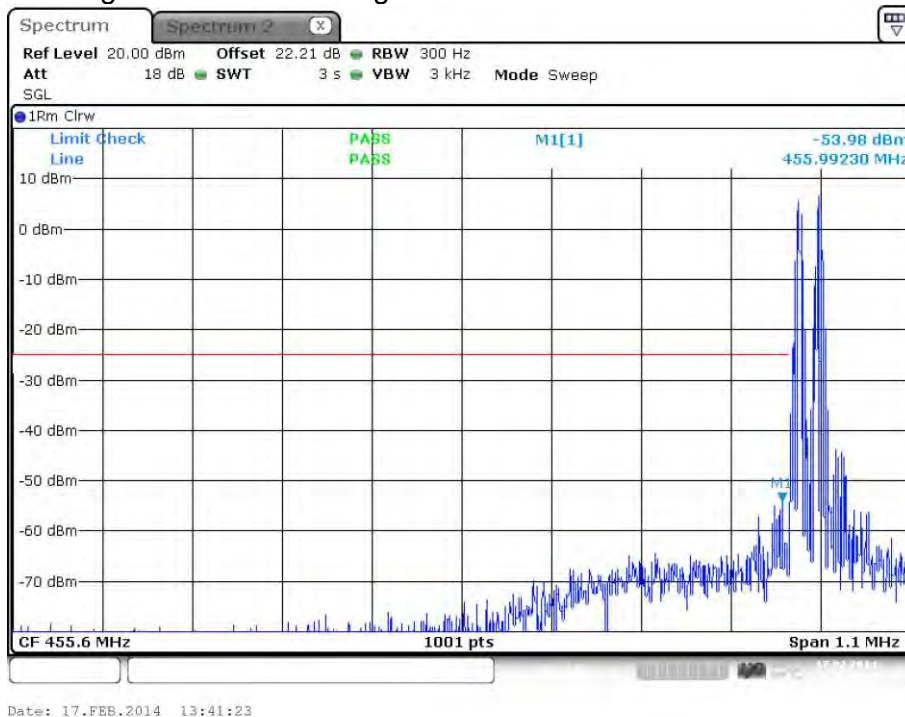
plot 7.3.1.2-#1 Spurious Emissions at Antenna Terminals: §90.210, §2.1051; Test results; Downlink; Band # 2; Analog < 1MHz to band edge; Lower Band Edge
