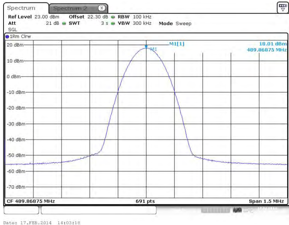
plot 5.3.1.4-#1 RF Power Out: $90.635, $2.1046; Test Results; Downlink; Band # 4; APCO Phase2 H-DQPSK
