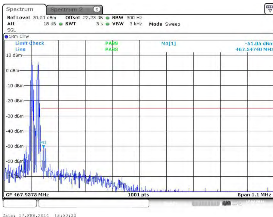
plot 7.3.1.3-#2 Spurious Emissions at Antenna Terminals: §90.210, §2.1051; Test results; Downlink; Band # 3; Analog < 1MHz to band edge; Upper Band Edge
