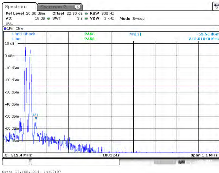
plot 7.3.1.4-#2 Spurious Emissions at Antenna Terminals: §90.210, §2.1051; Test results; Downlink; Band # 4; APCO Phase1 C4FM < 1MHz to band edge; Upper Band Edge
