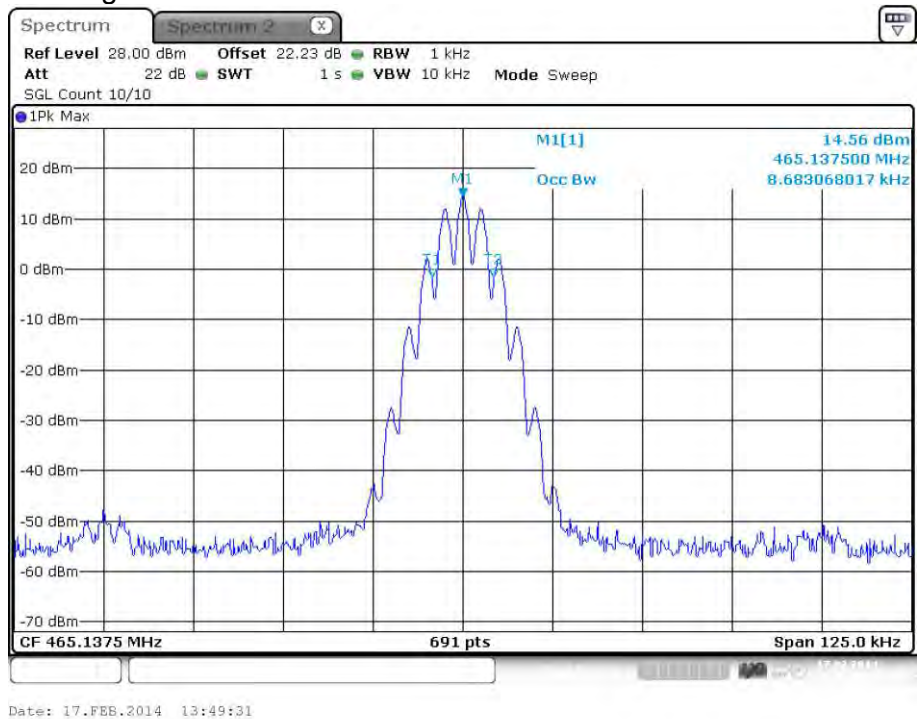
plot 6.3.1.3-#1 Occupied Bandwidth: $90.210, $2.1049; Test results; Downlink; Band # 3; Analog; Output
