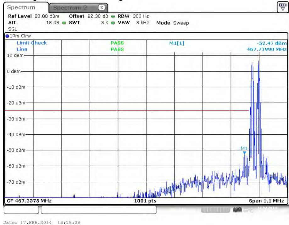
plot 7.3.1.4-#1 Spurious Emissions at Antenna Terminals: §90.210, §2.1051; Test results; Downlink; Band # 4; Analog < 1MHz to band edge; Lower Band Edge
