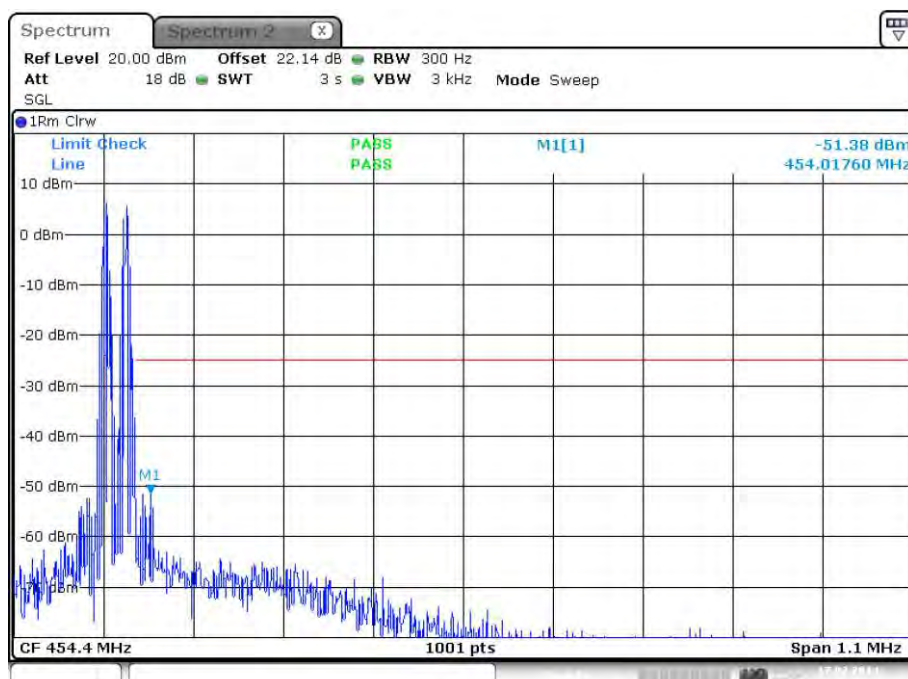
plot 7.3.1.1-#1 Spurious Emissions at Antenna Terminals: §90.210, §2.1051; Test results; Downlink; Band # 1; Analog < 1MHz to band edge; Lower Band Edge
