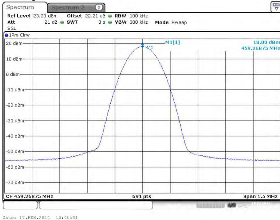
plot 5.3.1.2-#1 RF Power Out: §90.635, §2.1046; Test Results; Downlink; Band # 2; Analog
