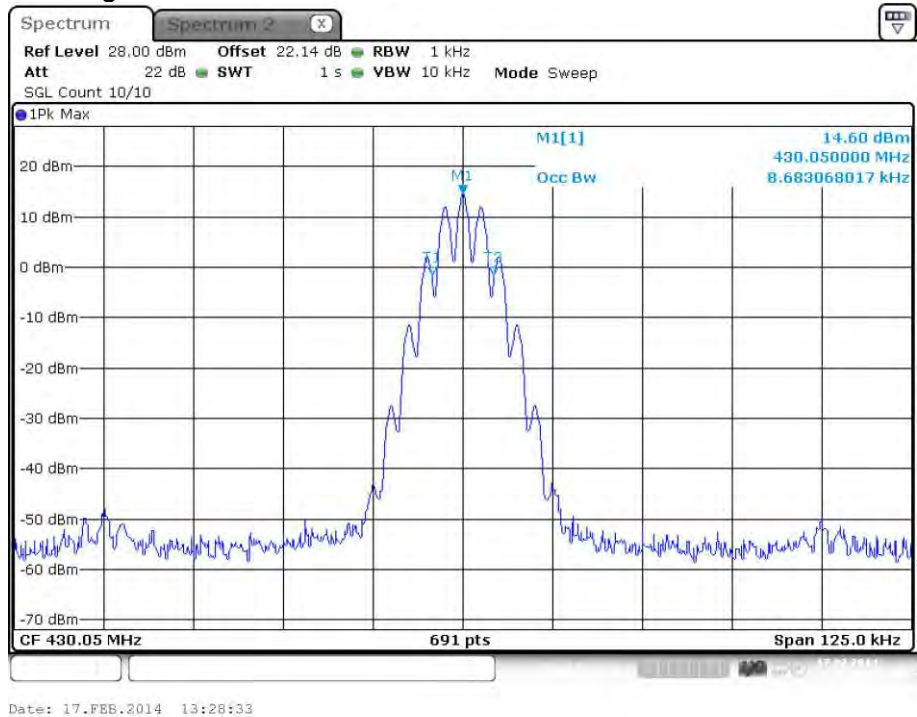
plot 6.3.1.1-#1 Occupied Bandwidth: $90.210, $2.1049; Test results; Downlink; Band # 1; Analog; Output
