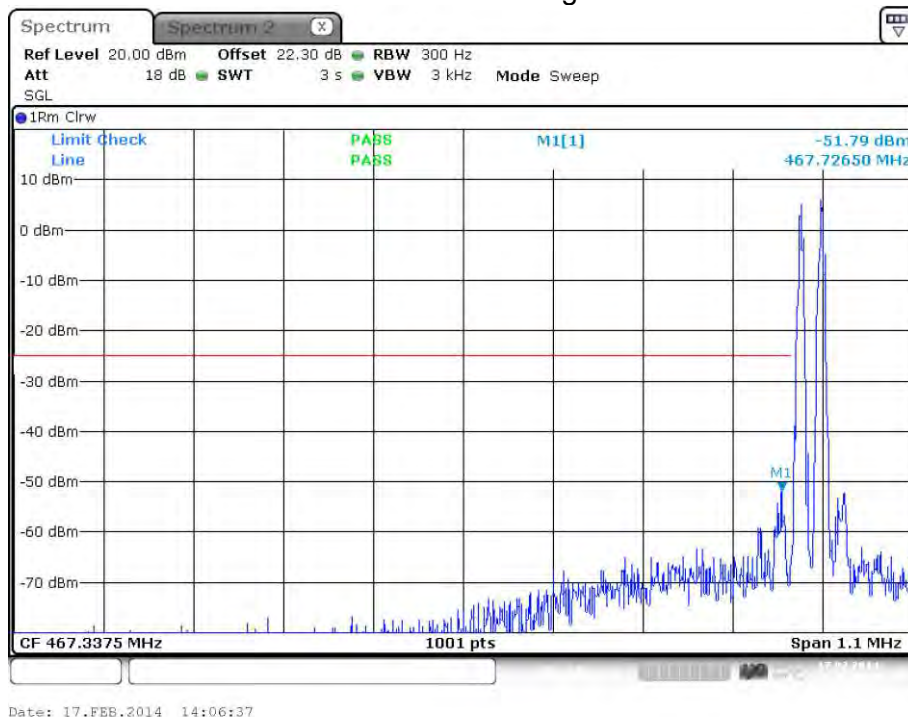
plot 7.3.1.4-#1 Spurious Emissions at Antenna Terminals: §90.210, §2.1051; Test results; Downlink; Band # 4; APCO Phase1 C4FM < 1MHz to band edge; Lower Band Edge
