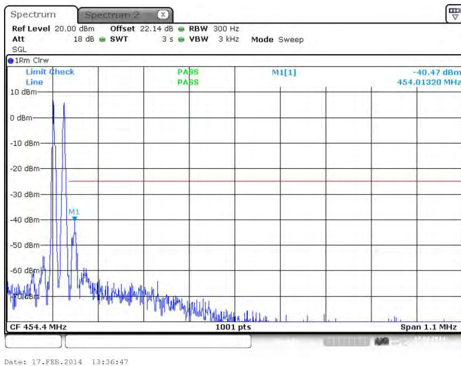
plot 7.3.1.1-#2 Spurious Emissions at Antenna Terminals: §90.210, §2.1051; Test results; Downlink; Band # 1; APCO Phase1 C4FM < 1MHz to band edge; Upper Band Edge
