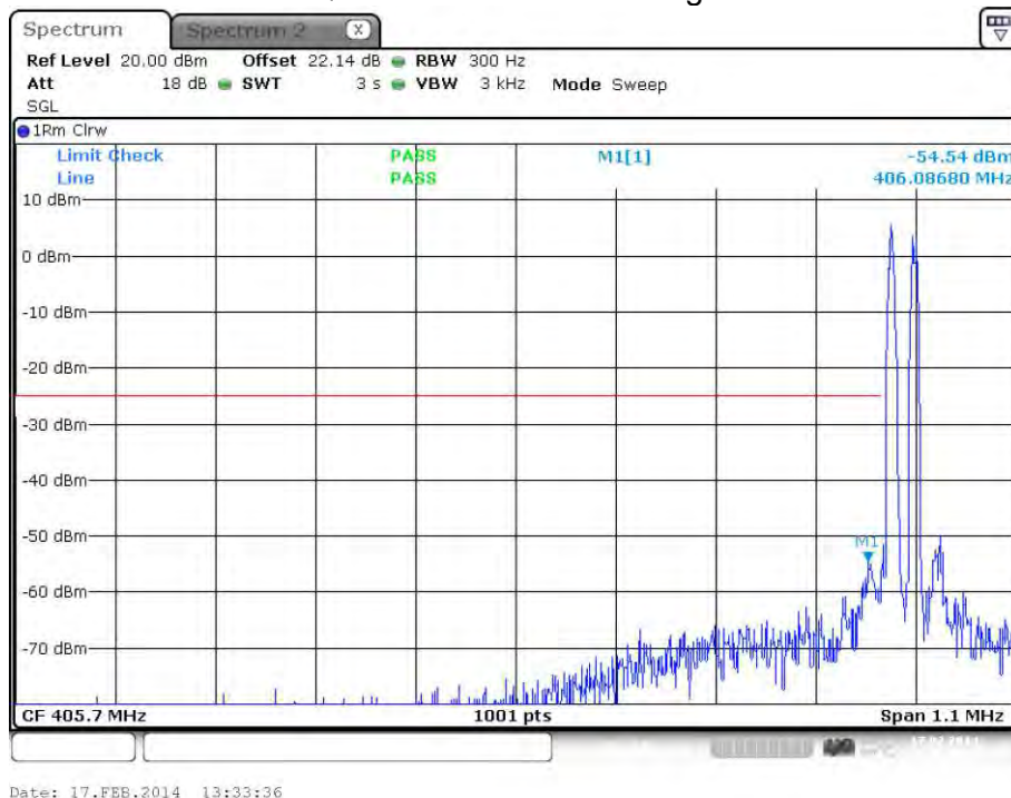
plot 7.3.1.1-#1 Spurious Emissions at Antenna Terminals: §90.210, §2.1051; Test results; Downlink; Band # 1; APCO Phase2 H-DQPSK < 1MHz to band edge; Lower Band Edge
