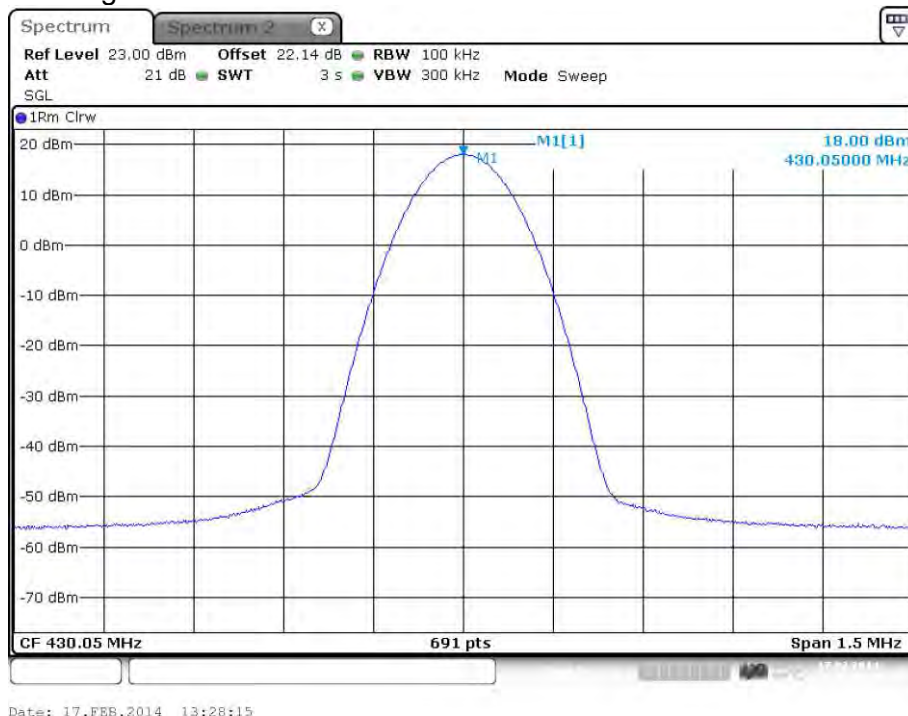
plot 5.3.1.1-#1 RF Power Out: §90.635, §2.1046; Test Results; Downlink; Band # 1; Analog
