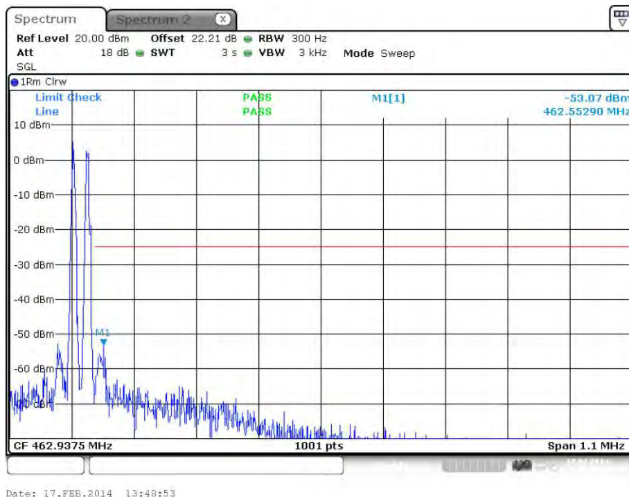
plot 7.3.1.2-#2 Spurious Emissions at Antenna Terminals: §90.210, §2.1051; Test results; Downlink; Band # 2; APCO Phase1 C4FM < 1MHz to band edge; Upper Band Edge
