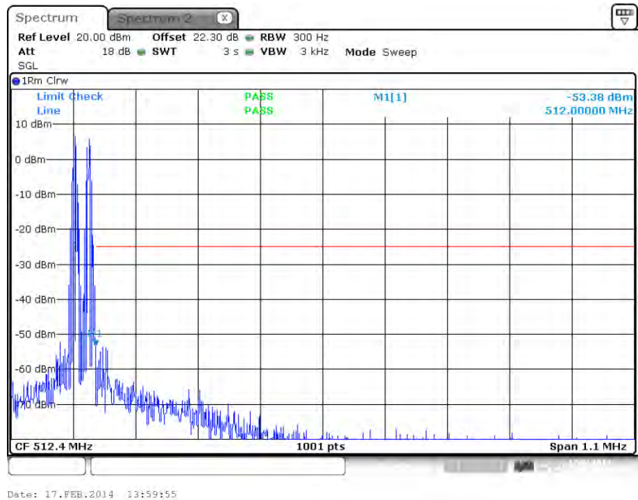
plot 7.3.1.4-#2 Spurious Emissions at Antenna Terminals: §90.210, §2.1051; Test results; Downlink; Band # 4; Analog < 1MHz to band edge; Upper Band Edge
