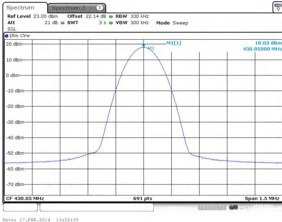
plot 5.3.1.1-#1 RF Power Out: §90.635, §2.1046; Test Results; Downlink; Band # 1; APCO Phase2 H-DQPSK
