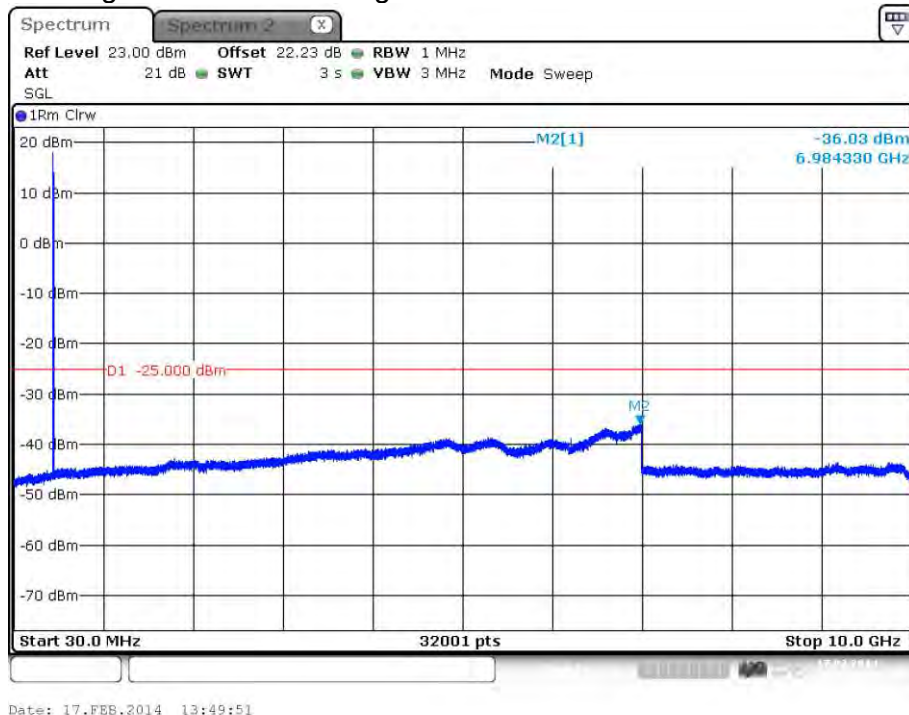
plot 7.3.1.7-#1 Spurious Emissions at Antenna Terminals: §90.210, §2.1051; Test results; Downlink; Band # 3; Analog > 1MHz to band edge;
