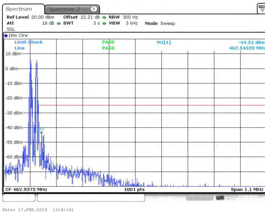
plot 7.3.1.2-#2 Spurious Emissions at Antenna Terminals: §90.210, §2.1051; Test results; Downlink; Band # 2; Analog < 1MHz to band edge; Upper Band Edge
