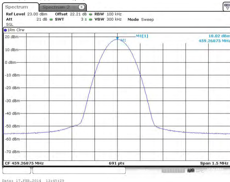
plot 5.3.1.2-#1 RF Power Out: §90.635, §2.1046; Test Results; Downlink; Band # 2; APCO Phase2 H-DQPSK
