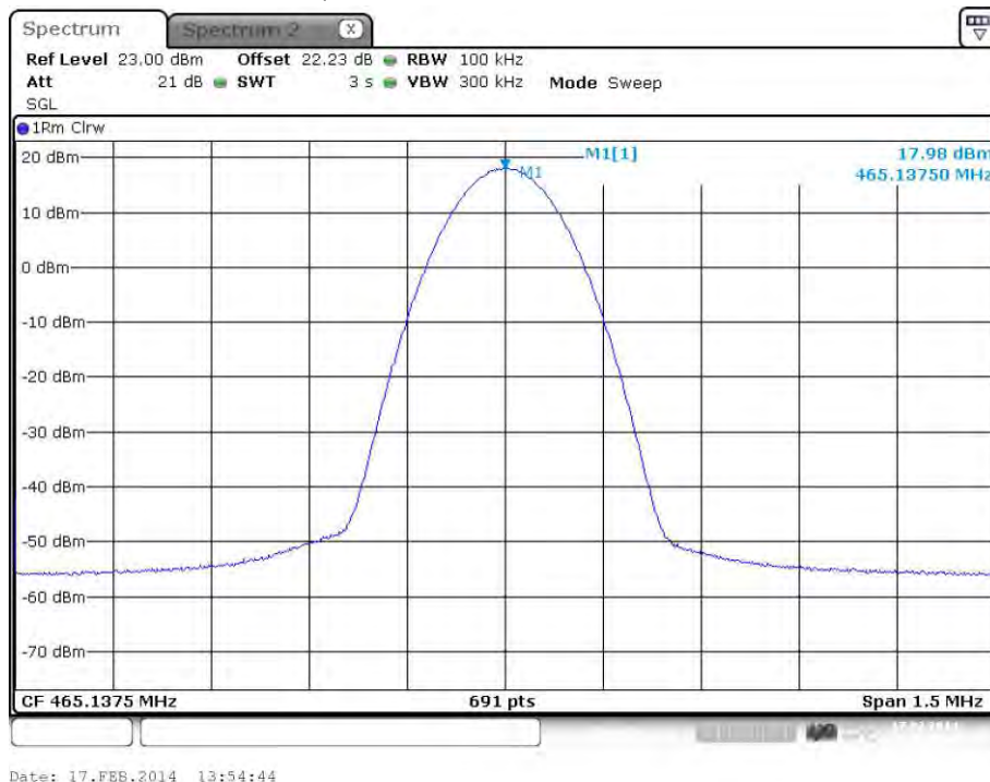
plot 5.3.1.3-#1 RF Power Out: §90.635, §2.1046; Test Results; Downlink; Band # 3; APCO Phase2 H-DQPSK
