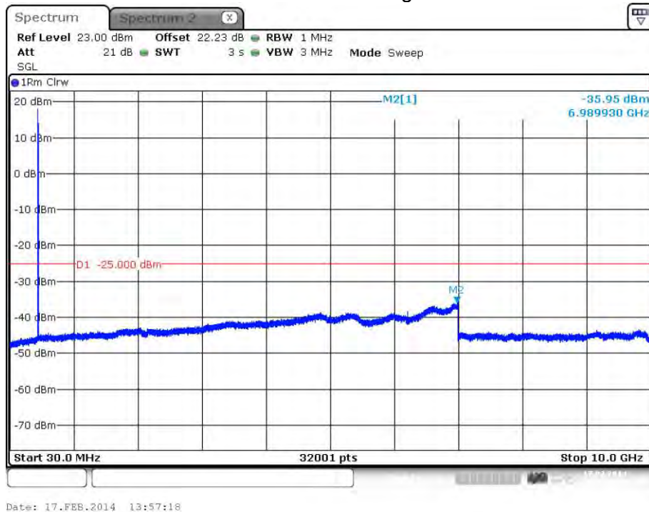
plot 7.3.1.7-#1 Spurious Emissions at Antenna Terminals: §90.210, §2.1051; Test results; Downlink; Band # 3; APCO Phase1 C4FM > 1MHz to band edge;
