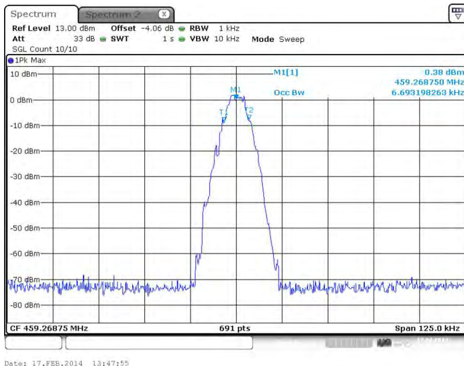
plot 6.3.1.2-#2 Occupied Bandwidth: §90.210, §2.1049; Test results; Downlink; Band # 2; APCO Phase1 C4FM; Input
