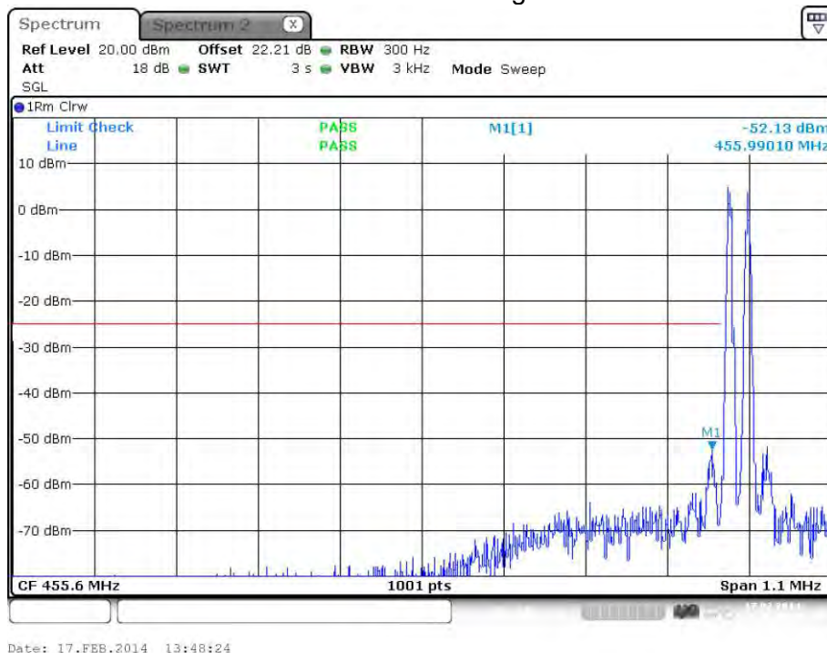
plot 7.3.1.2-#1 Spurious Emissions at Antenna Terminals: §90.210, §2.1051; Test results; Downlink; Band # 2; APCO Phase1 C4FM < 1MHz to band edge; Lower Band Edge
