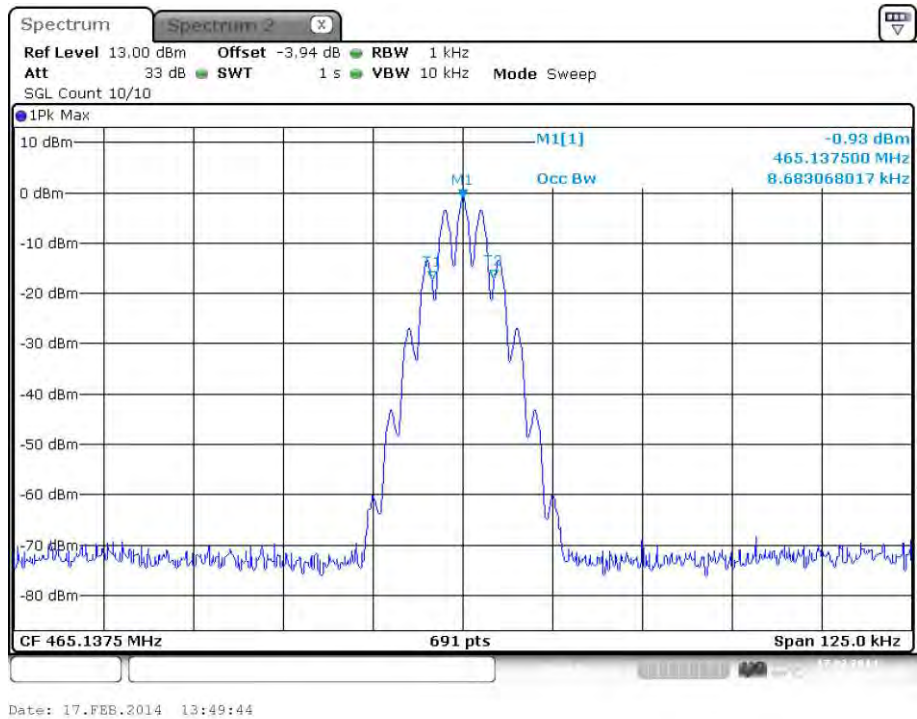
plot 6.3.1.3-#2 Occupied Bandwidth: $90.210, $2.1049; Test results; Downlink; Band # 3; Analog; Input
