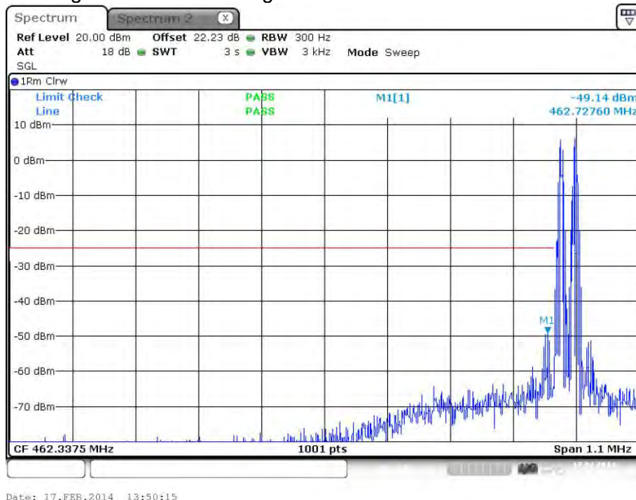
plot 7.3.1.3-#1 Spurious Emissions at Antenna Terminals: §90.210, §2.1051; Test results; Downlink; Band # 3; Analog < 1MHz to band edge; Lower Band Edge
