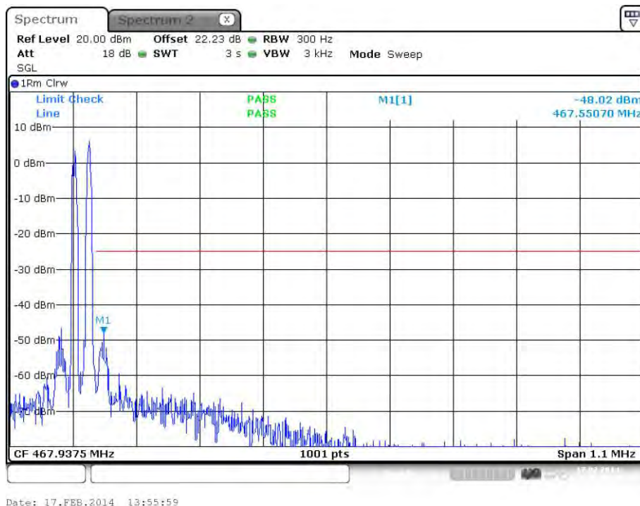
plot 7.3.1.3-#2 Spurious Emissions at Antenna Terminals: §90.210, §2.1051; Test results; Downlink; Band # 3; APCO Phase2 H-DQPSK < 1MHz to band edge; Upper Band Edge
