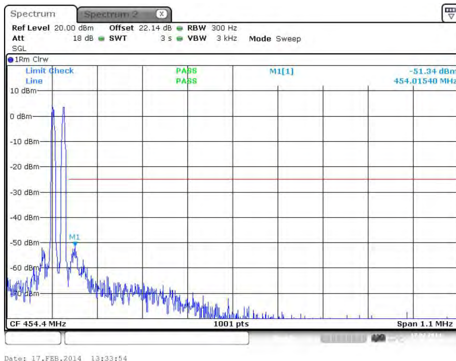
plot 7.3.1.1-#2 Spurious Emissions at Antenna Terminals: §90.210, §2.1051; Test results; Downlink; Band # 1; APCO Phase2 H-DQPSK < 1MHz to band edge; Upper Band Edge
