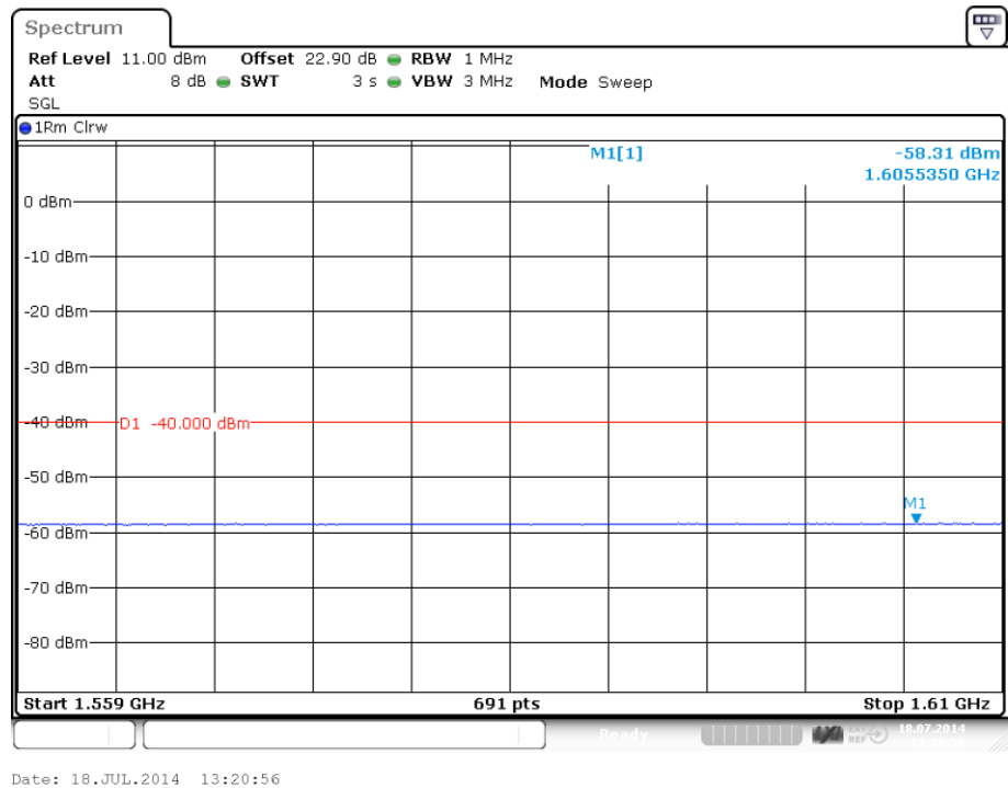
plot 7.3.1.3-#1 Spurious Emissions at Antenna Terminals: §90.543, §2.1051; Test results; Downlink; Measurement in the band of 1559 MHz – 1610 MHz acc. to 27.53(f)
