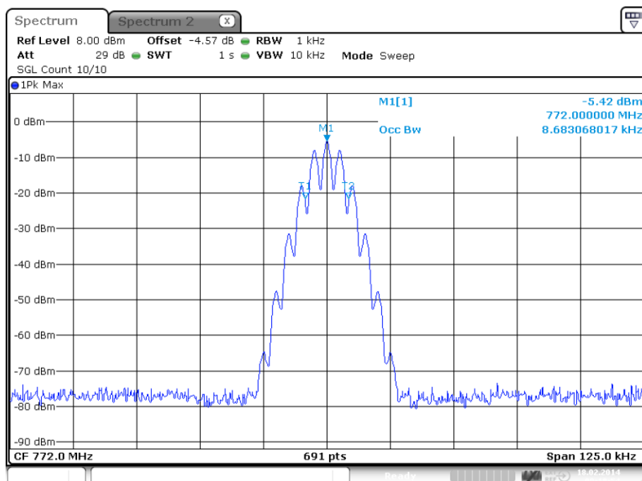
plot 6.3.1.1-#2 Occupied Bandwidth: 8.683068017 kHz; Test results; Downlink; Analog Input
