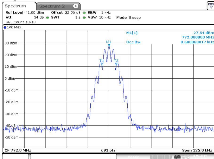
plot 6.3.1.1-#1 Occupied Bandwidth: 8.683068017 kHz; Test results; Downlink; Analog Output
