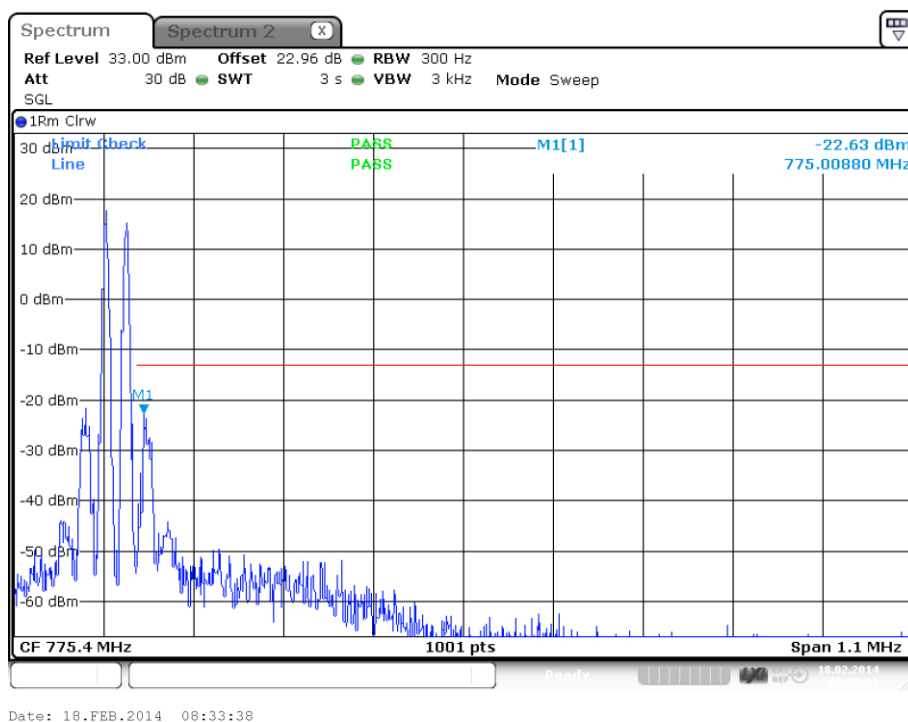
plot 7.3.1.1-#4 Spurious Emissions at Antenna Terminals: §90.543, §2.1051; Test results; Downlink; Analog < 1MHz to band edge; Upper Band Edge
