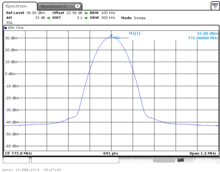
plot 5.3.1.3-#1 RF Power Out: §90.635, §2.1046; Test Results; Downlink; APCO Phase2 H-DQPSK
