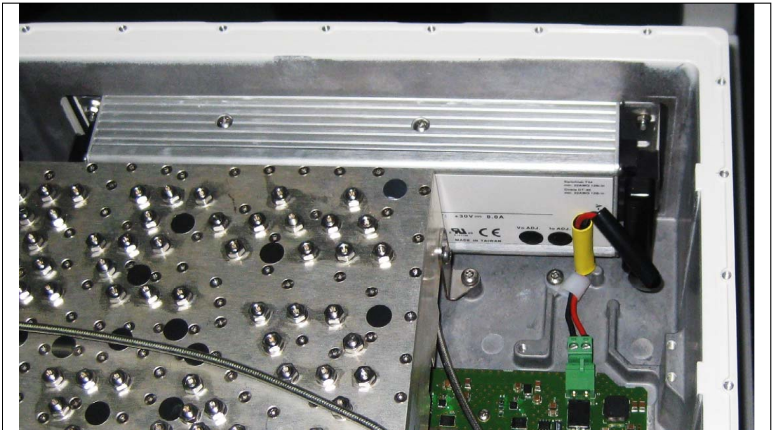
Power Supply
