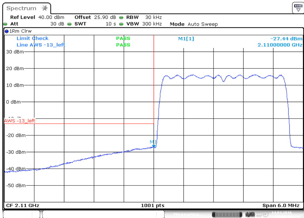
plot 8.3.1.1-#1 Intermodulation: §27.53, §2.1051; Test results; Downlink; CDMA Lower Band Edge
