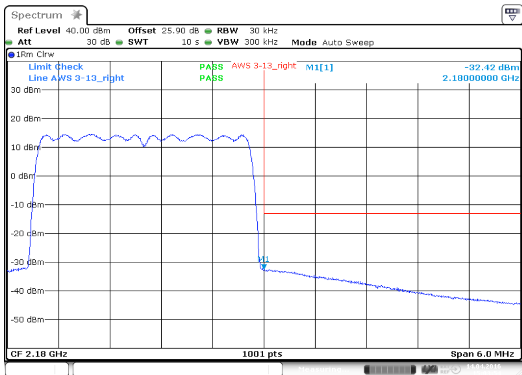
plot 8.3.1.1-#2 Intermodulation: §27.53, §2.1051; Test results; Downlink; CDMA Upper Band Edge
