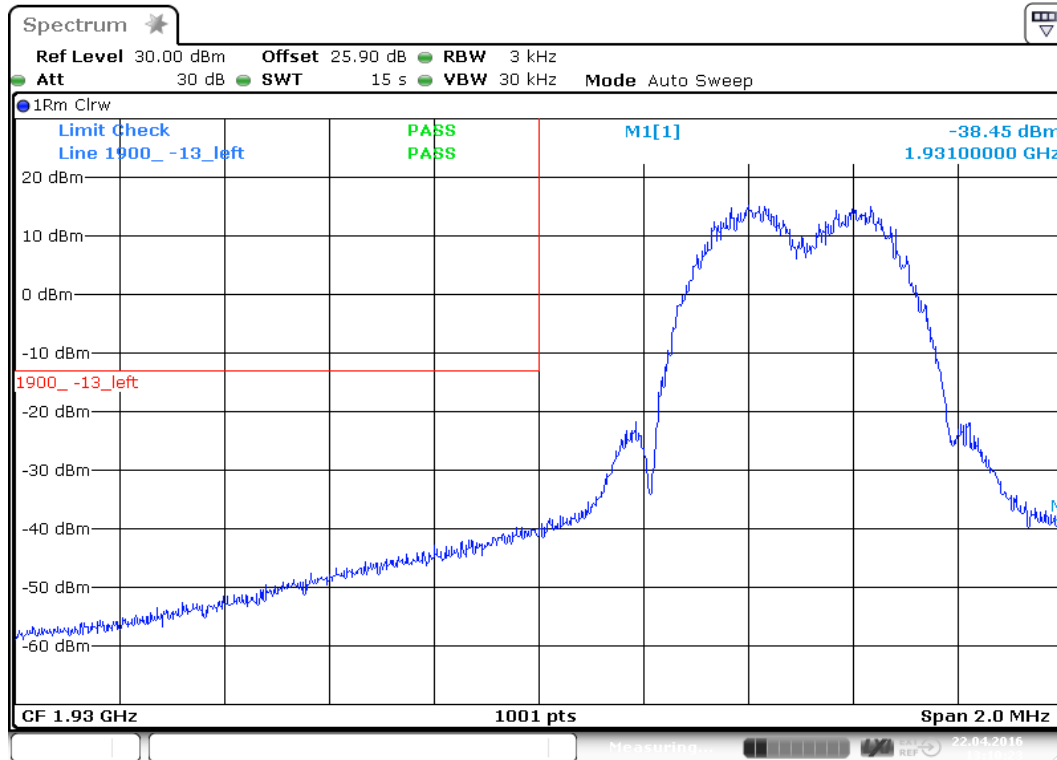
plot 8.3.1.2-#1 Intermodulation: §24.238, §2.1051; Test results; Downlink; EDGE Lower Band Edge
