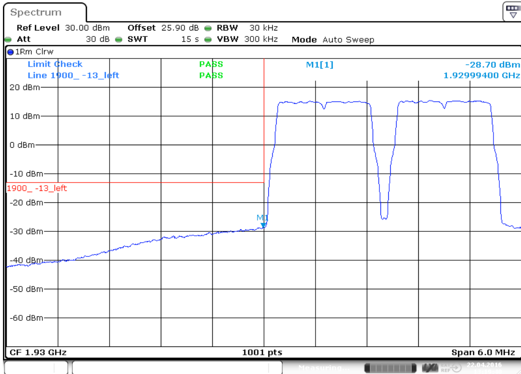
plot 8.3.1.5-#1 Intermodulation: §24.238, §2.1051; Test results; Downlink; LTE Lower Band Edge
