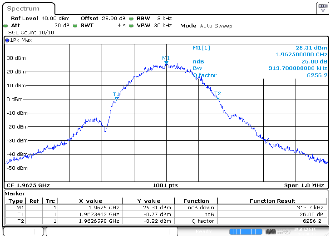
plot 6.3.2.2-#1 Occupied Bandwidth: $2.1049;; Test results; 26dB Bandwidth; EDGE Output
