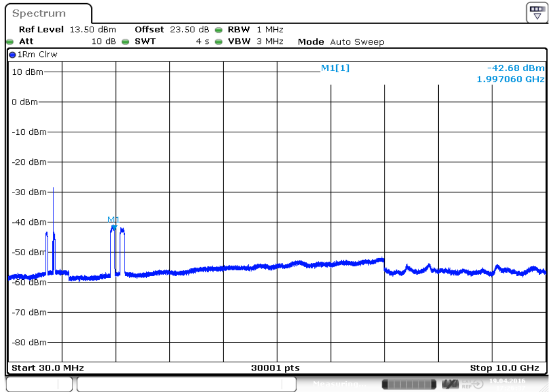
plot 7.3.1.5-#1 Spurious Emissions at Antenna Terminals: §90.210, §2.1051; Test results; Downlink; LTE; carrier (865,5MHz) notched
