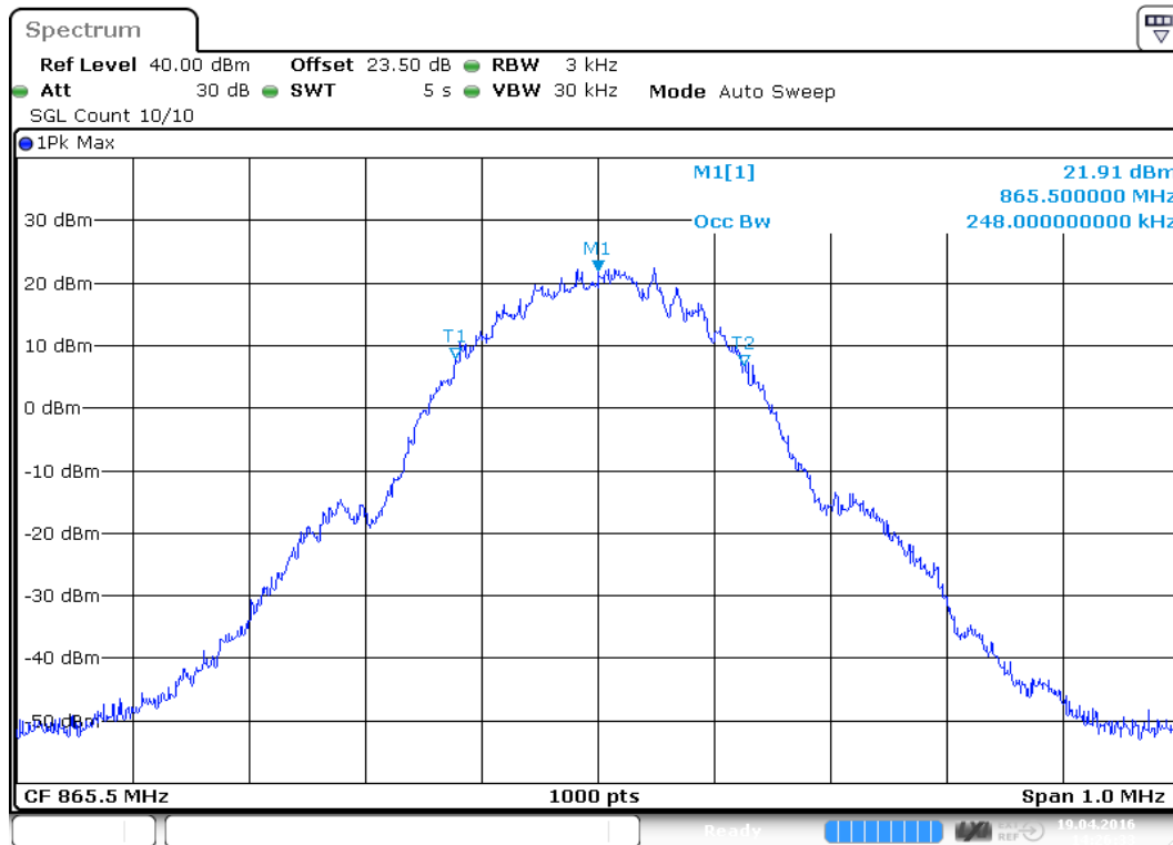
plot 6.3.1.1-#1 Occupied Bandwidth: §90.210, §2.1049; Test results; Downlink; GSM Output
