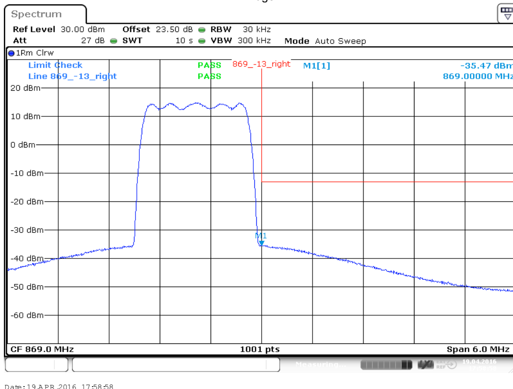
plot 9.3.1.3-#2 Emission Mask: §90.691, §2.1051; Test results; Downlink; CDMA < 1MHz to band edge Upper Band Edge
