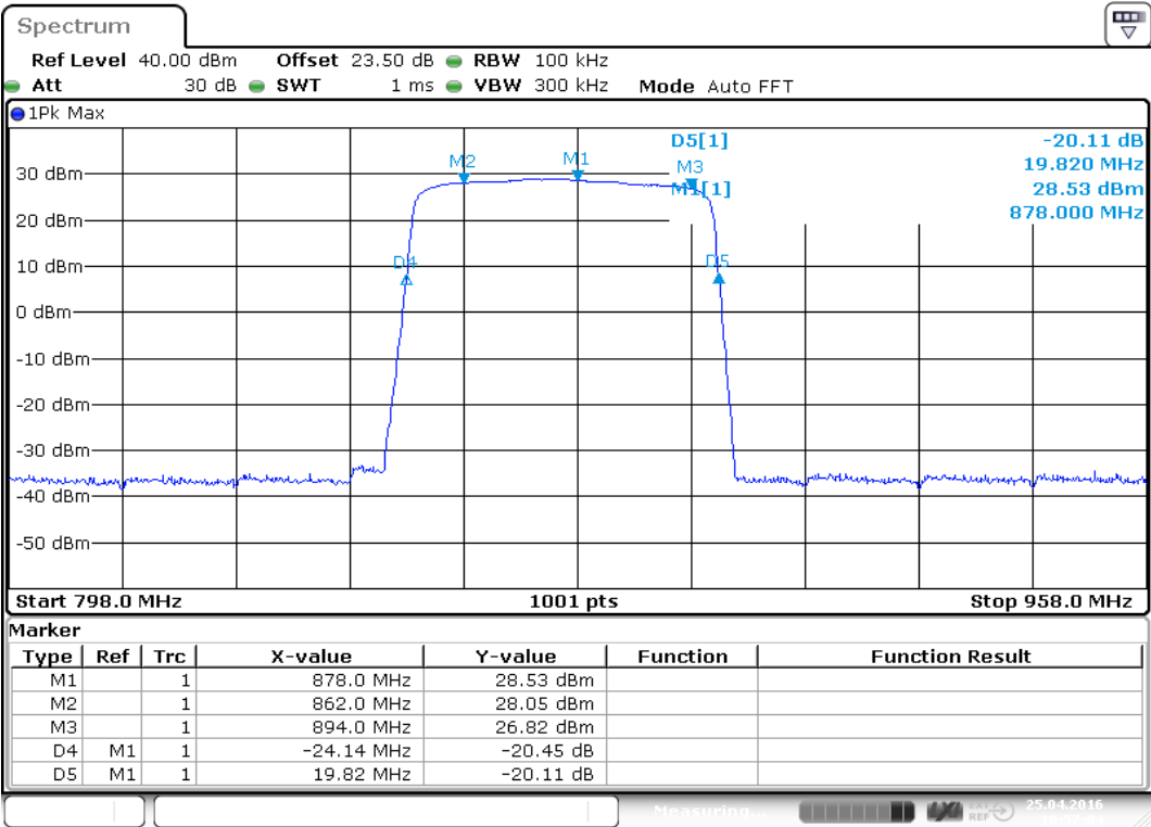
plot 10.3.1-#1 Out of Band Rejection; Test results; Downlink;
