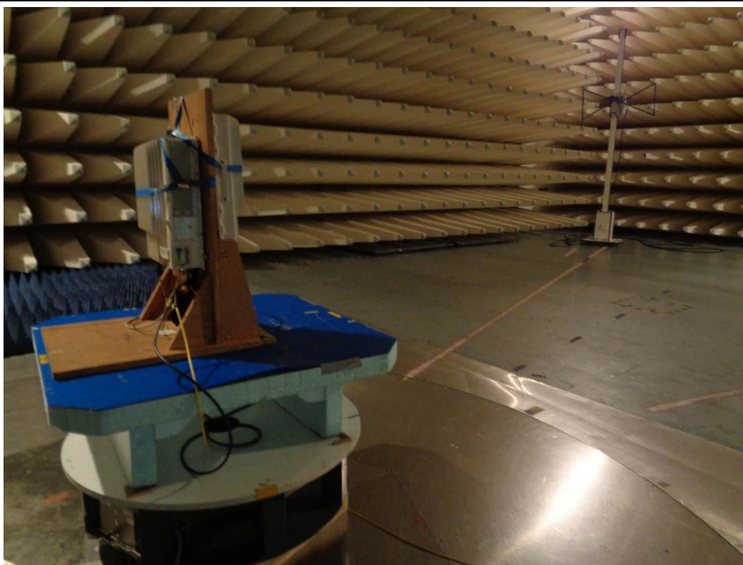
picture 8.2: Test setup: Field Strength Emission 30 MHz – 1 GHz @10m in the SAC
