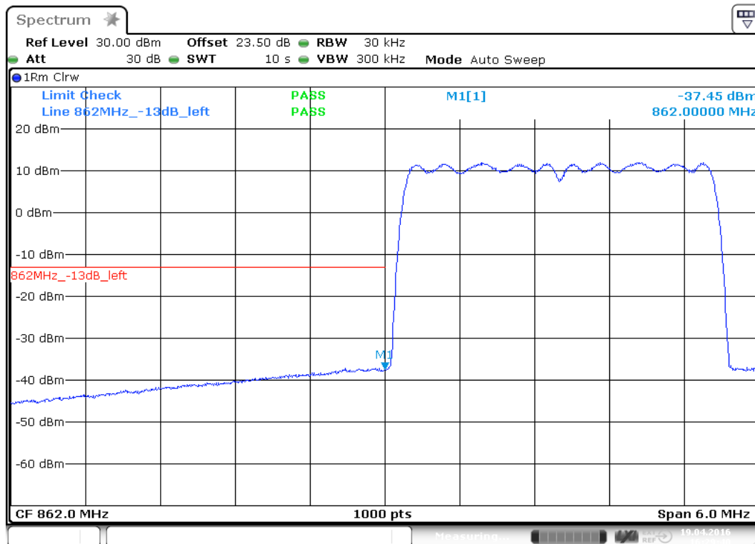
plot 8.3.1.3-#1 Intermodulation: §90.219, §2.1051; Test results; Downlink; CDMA Lower Band Edge
