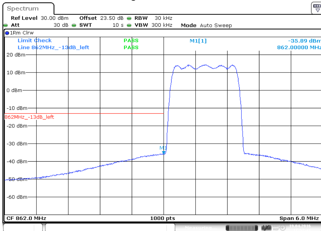
plot 9.3.1.3-#1 Emission Mask: §90.691, §2.1051; Test results; Downlink; CDMA < 1MHz to band edge Lower Band Edge
