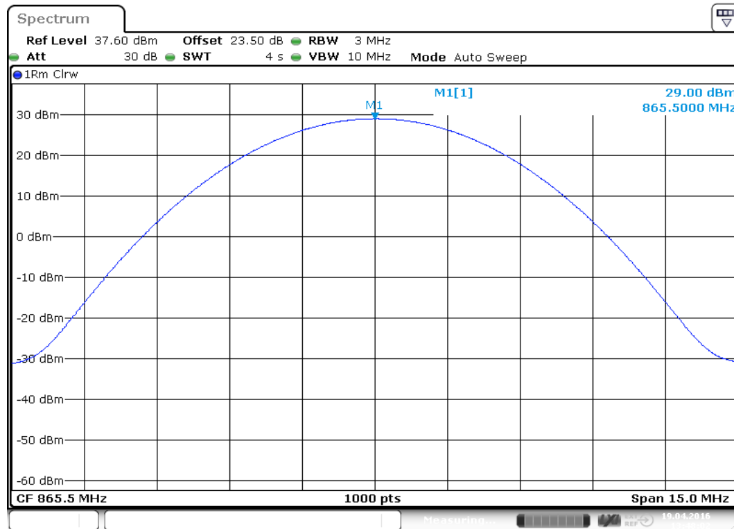
plot 5.3.1.3-#1 RF Power Out: §90.635, §2.1046; Test Results; Downlink; CDMA Middle
