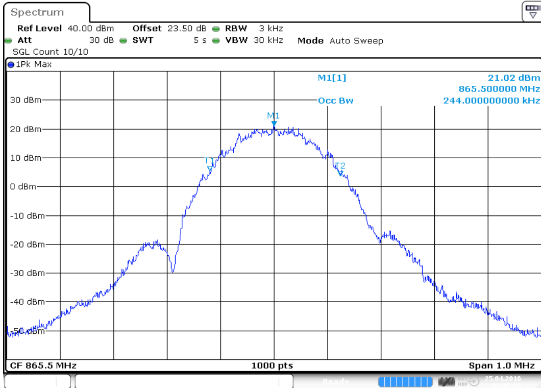
plot 6.3.1.2-#1 Occupied Bandwidth: §90.210, §2.1049; Test results; Downlink; EDGE Output
