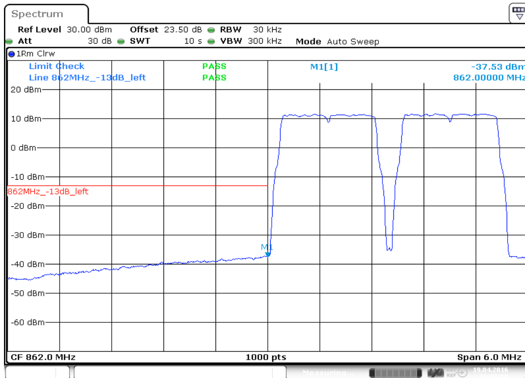
plot 8.3.1.5-#1 Intermodulation: §90.219, §2.1051; Test results; Downlink; LTE Lower Band Edge
