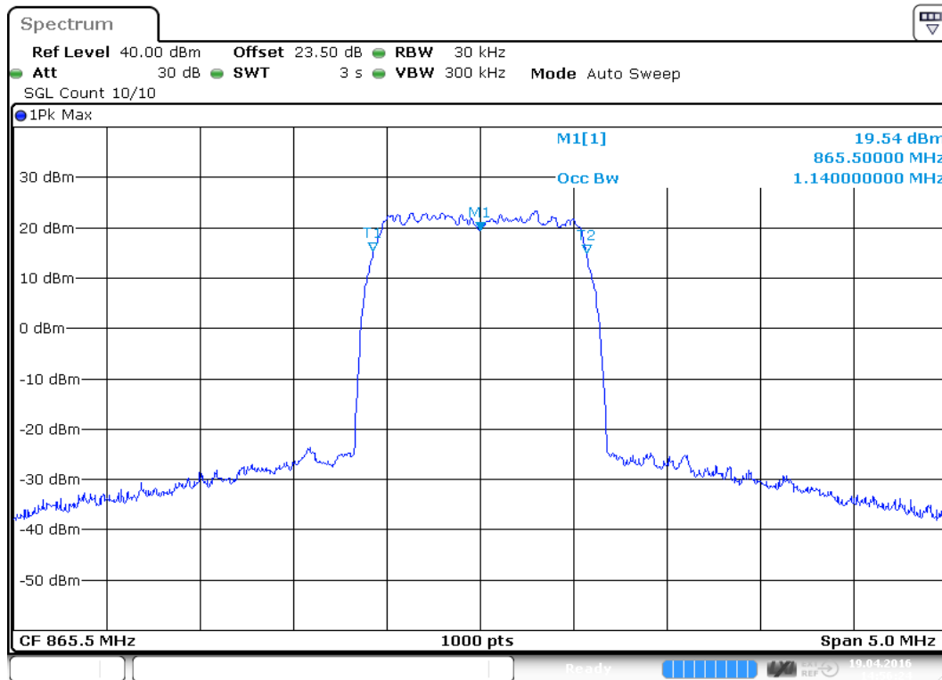
plot 6.3.1.5-#1 Occupied Bandwidth: $90.210, $2.1049; Test results; Downlink; LTE Output
