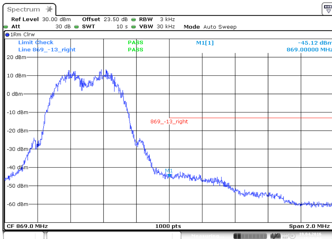
plot 8.3.1.1-#1 Intermodulation: §90.219, §2.1051; Test results; Downlink; GSM Lower Band Edge
