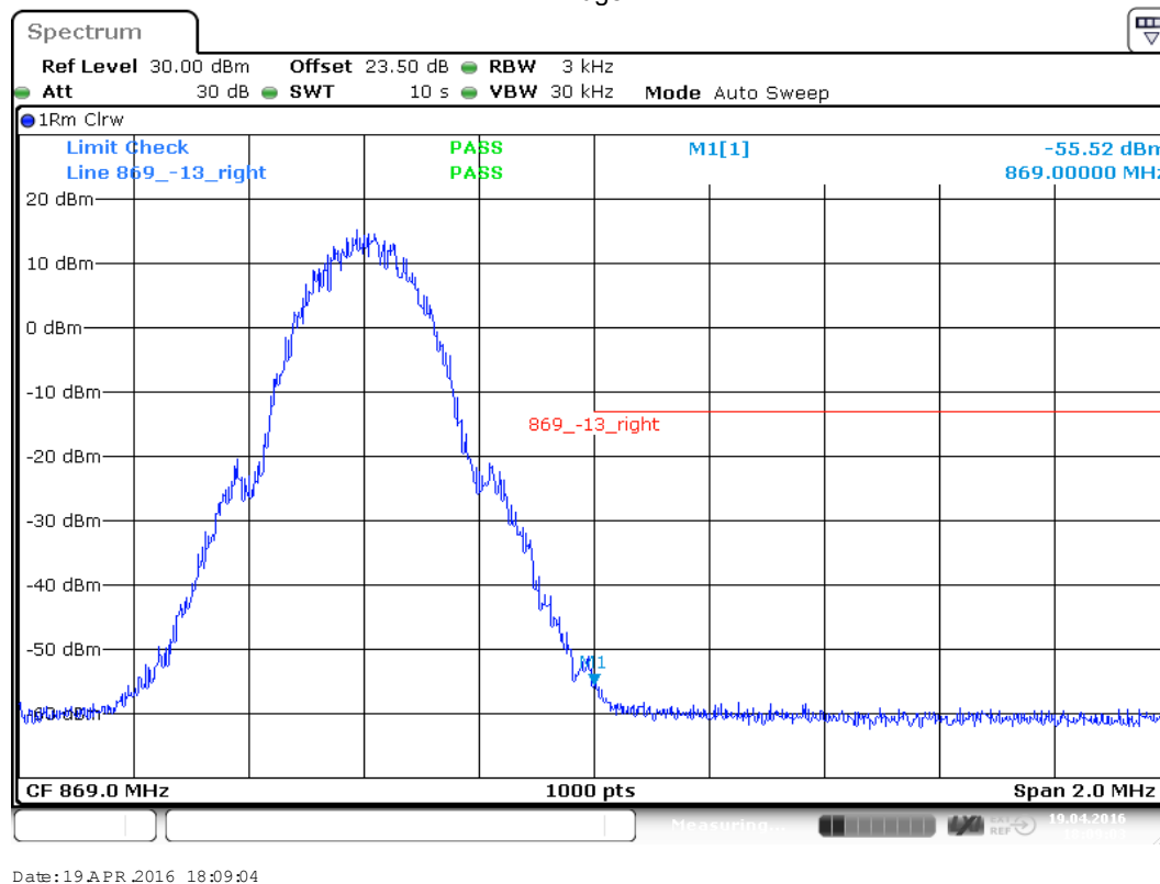
plot 9.3.1.1-#2 Emission Mask: §90.691, §2.1051; Test results; Downlink; GSM < 1MHz to band edge Upper Band Edge
