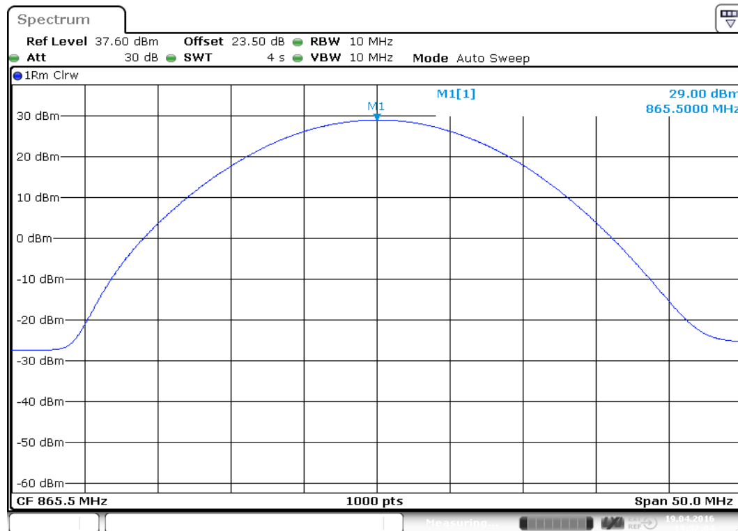
plot 5.3.1.4-#1 RF Power Out: §90.635, §2.1046; Test Results; Downlink; WCDMA Middle
