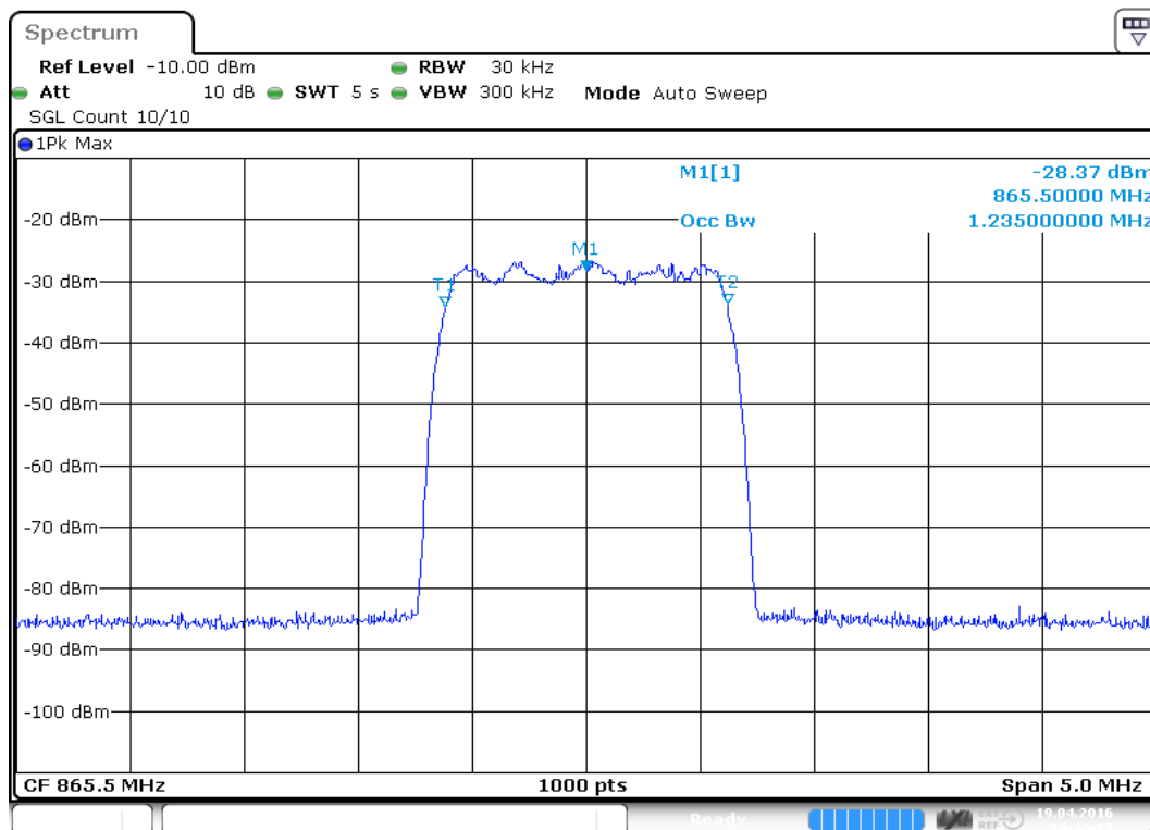
plot 6.3.1.3-#1 Occupied Bandwidth: $90.210, $2.1049; Test results; Downlink; CDMA Output
