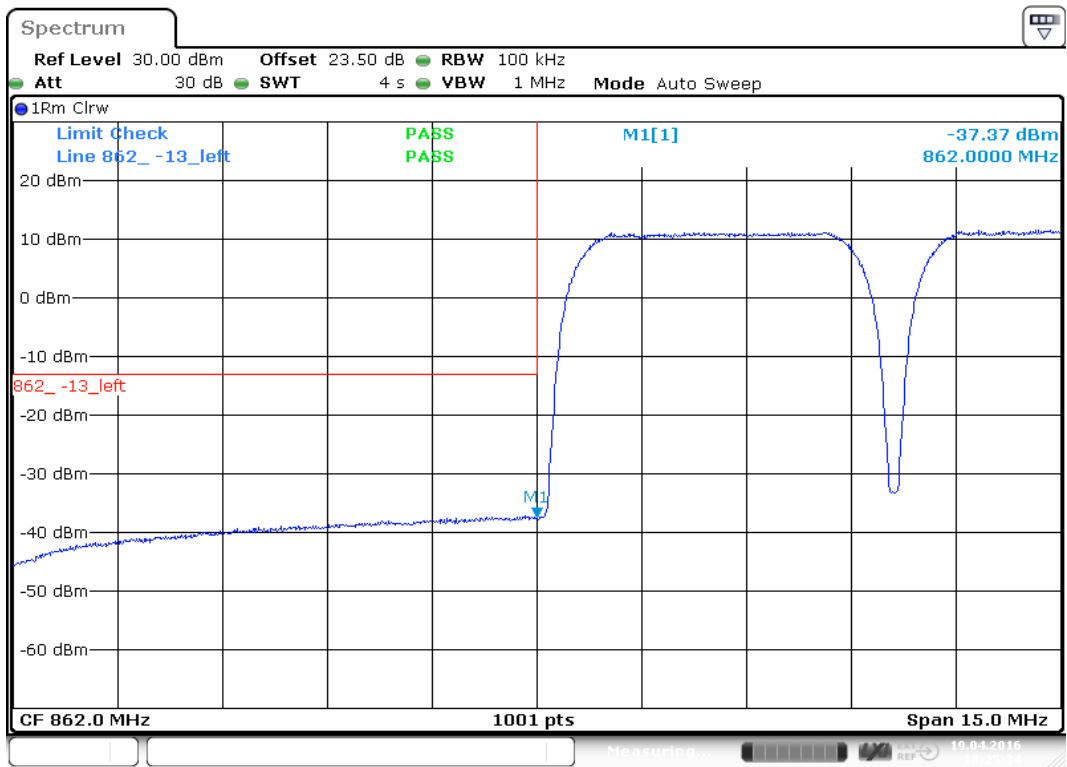
plot 8.3.1.4-#1 Intermodulation: §90.219, §2.1051; Test results; Downlink; WCDMA Lower Band Edge
