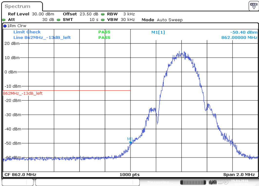
plot 9.3.1.2-#1 Emission Mask: §90.691, §2.1051; Test results; Downlink; EDGE < 1MHz to band edge Lower Band Edge
